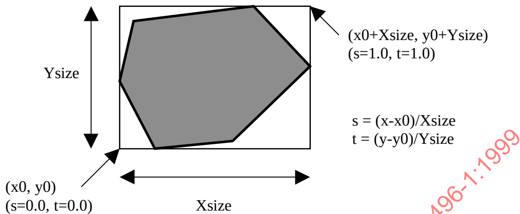
Figure 22 - IndexedFaceSet2D default texture mapping coordinates for a simple shape
