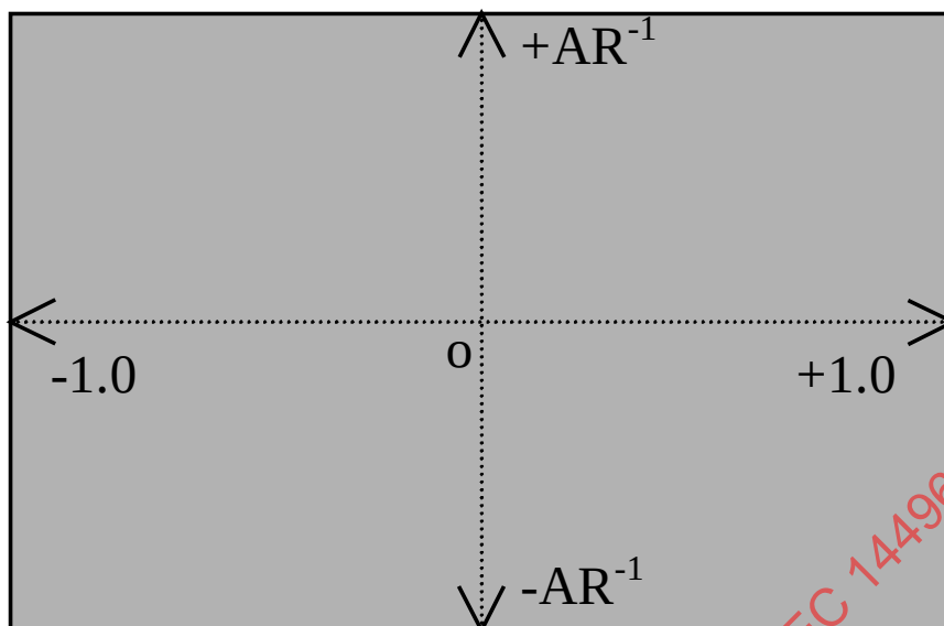
Figure 13 - 2D co-ordinate system ( AR = \text{Aspect Ratio} )
