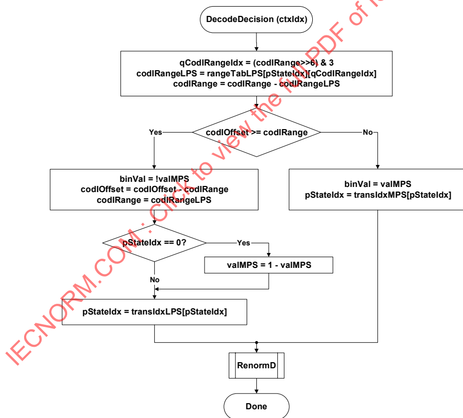
Figure 9-3 – Flowchart for decoding a decision
