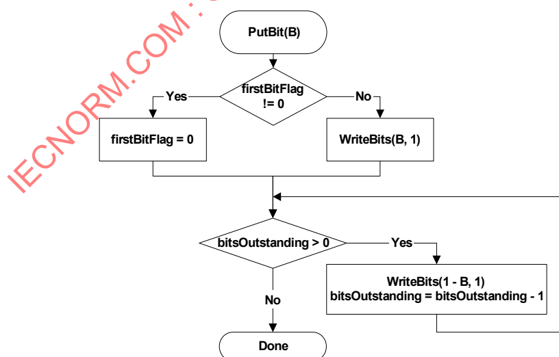
Figure 9-9 – Flowchart of PutBit(B)
