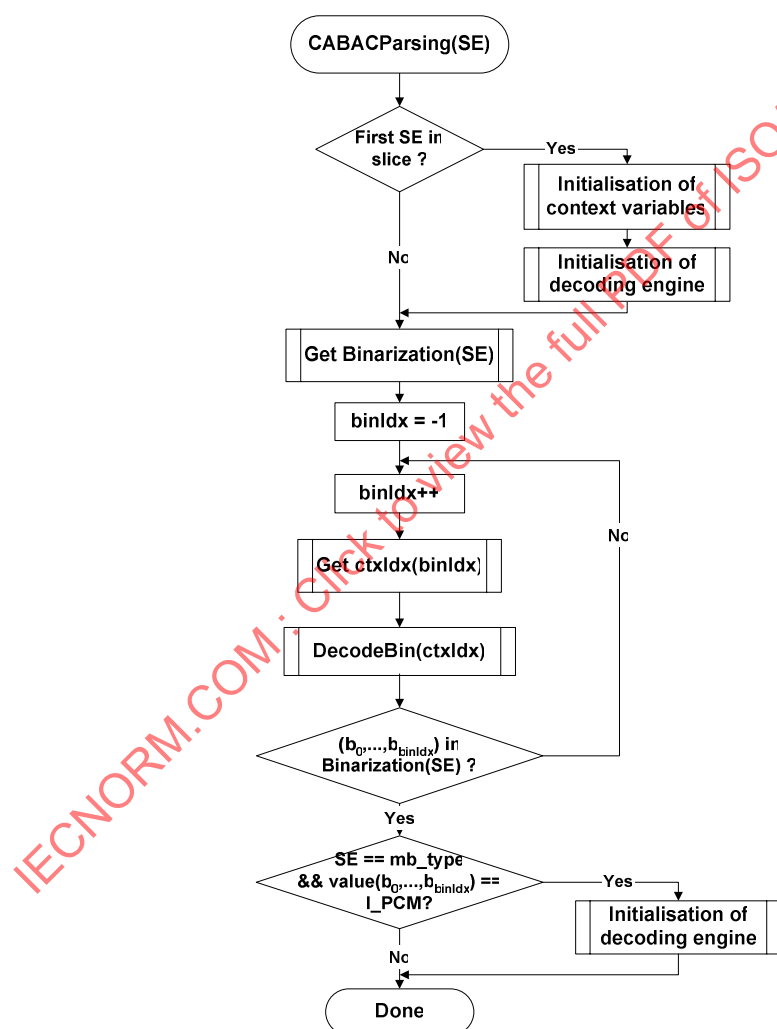
Figure 9-1 – Illustration of CABAC parsing process for a syntax element SE (informative)
