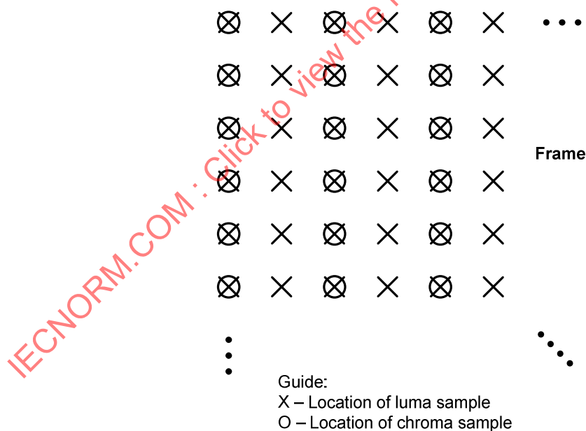
Figure 6-3 – Nominal vertical and horizontal locations of 4:2:2 luma and chroma samples in a frame
