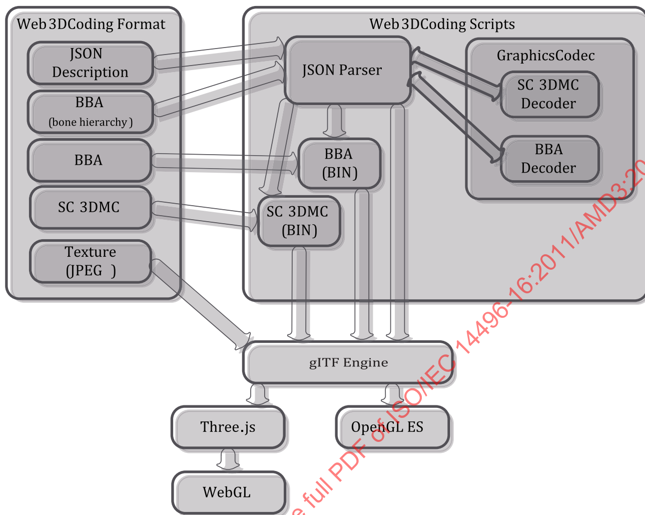
Figure 82 — Overview of the Web3DCoding architecture
