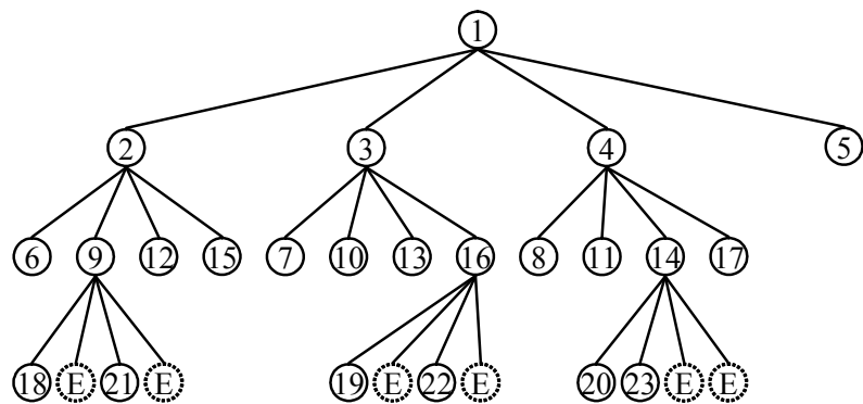
Figure 72 — Example of the decoding order for the tree nodes in Figure 70.
