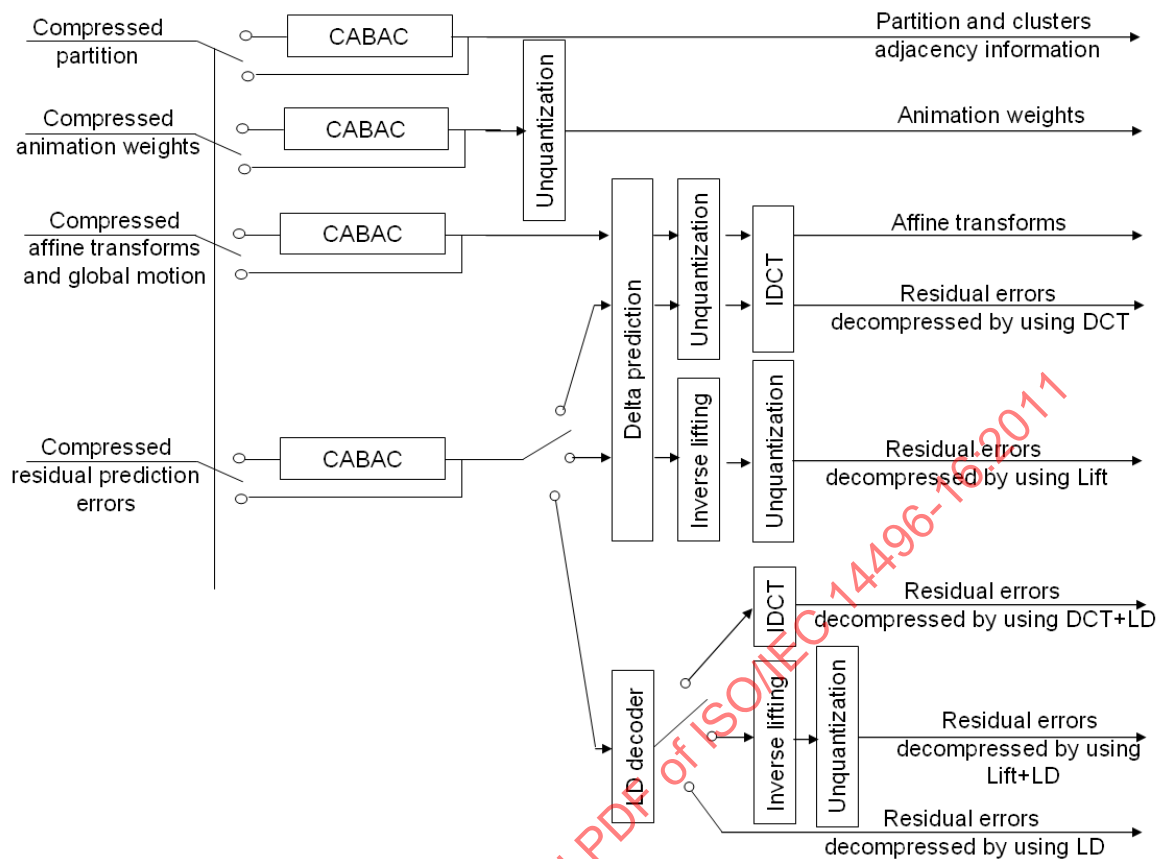
Figure 80 — FAMC decoding process.
