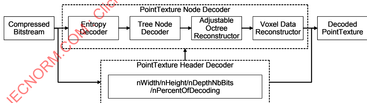
Figure 67 — Block diagram of decoder for PointTexture compression.
