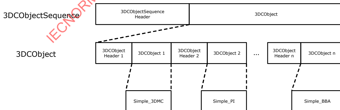
Figure 81 — Syntax of the MP43D stream
