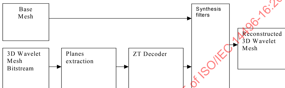
Figure A.1 — The typical Wavelet Mesh decoding process.
