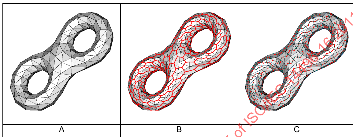
Figure 32 — A triangular 3D mesh (A), its dual graph (B), and a triangle tree (C)
