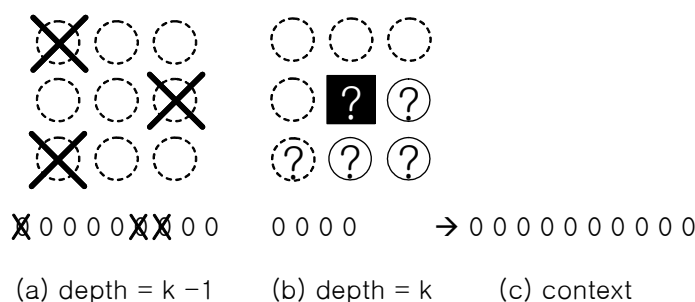
Figure 75 — Example of context: voxels represented by dotted circles in (a) and (b) are not existed voxels and a voxel to be decoded in (b) is located at a corner actually.
