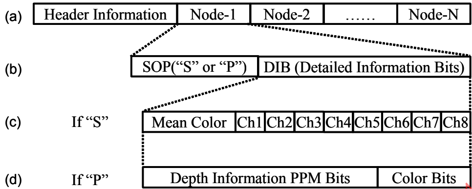
Figure 70 — Example of the bitstream structure for compressed PointTexture.
