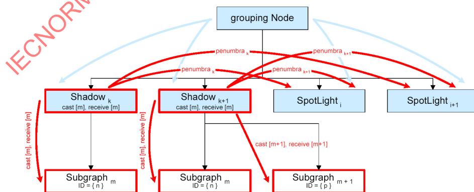
Figure 31 — Transmission of shadow properties to multiple 3D-surfaces and light sources
