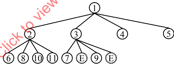
Figure 71 — Example of the decoding order for the tree nodes in Figure 69.
