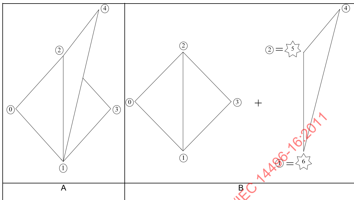
Figure 39 — A non-manifold 3D mesh (A) and converted manifold meshes (B)
