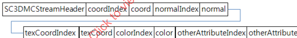
Figure 63 — SC3DMC stream structure.
