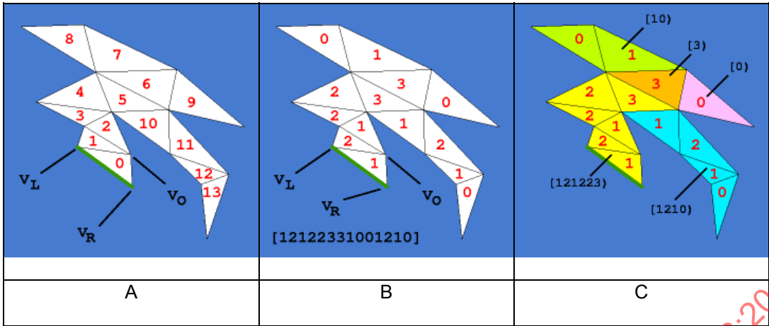
Figure 38 — Representing a simple polygon as a table of triangle runs.
