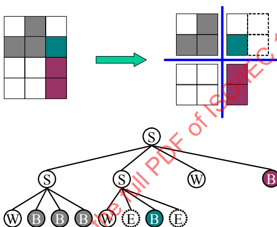
Figure 68 — Example of adjustable octree in the resolution of 3×4.
