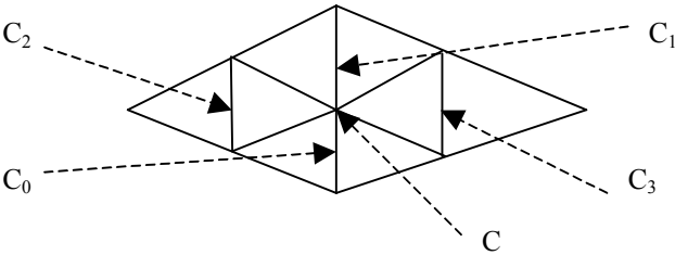
Figure A.2 — Definition of the offspring .
