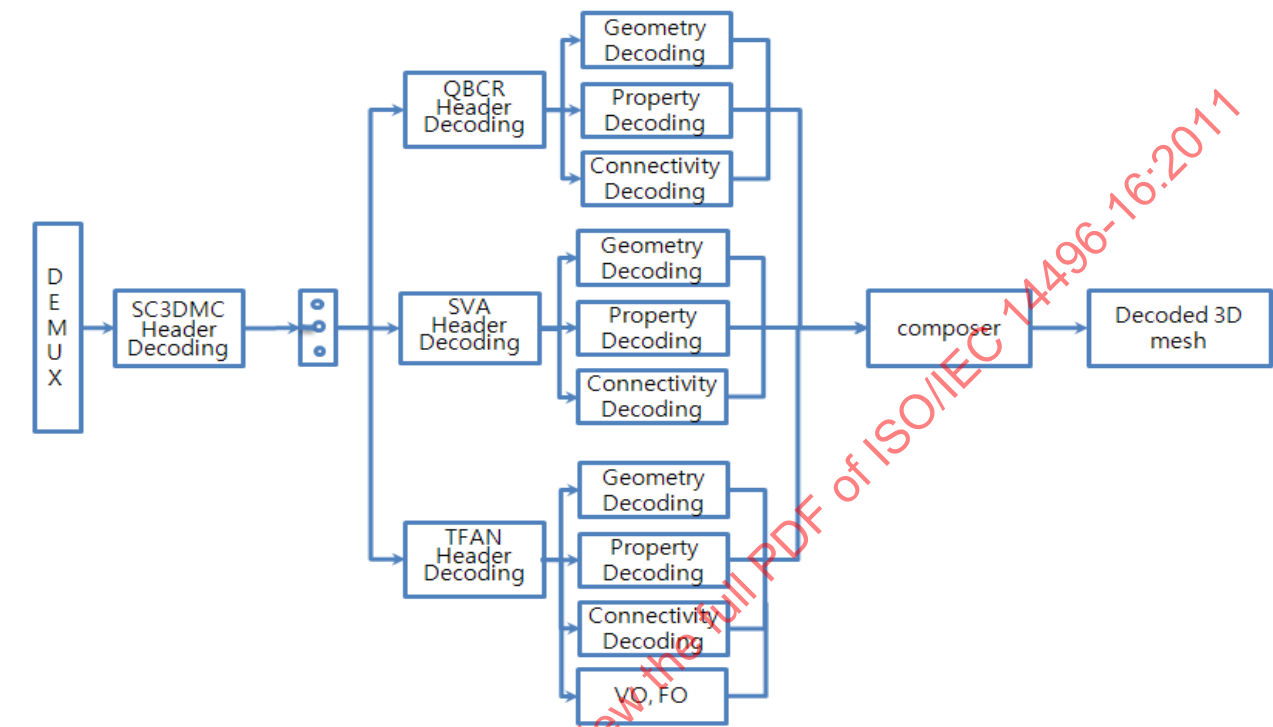
Figure 64 — SC3DMC Decoder structure
