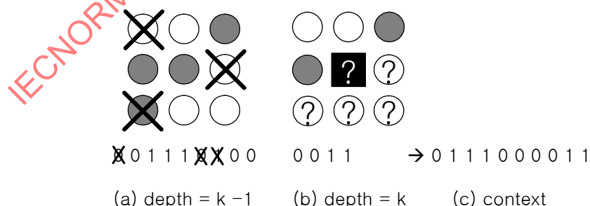
Figure 74 — Example of context: a voxel represented by a question marked black square in (b) is the voxel to be decoded and voxels represented by white circles and gray circles in (a) and (b) are used to make a context excluding three voxels which are marked with 'X'.
