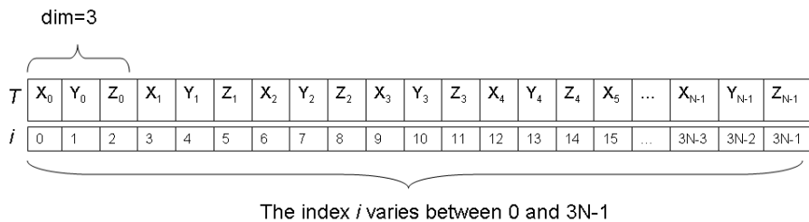
Figure 65 — Example of a flat representation of an array of quantized position coordinates.
