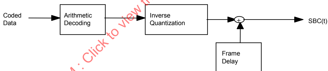
Figure 77 — SBC predictive coding.
