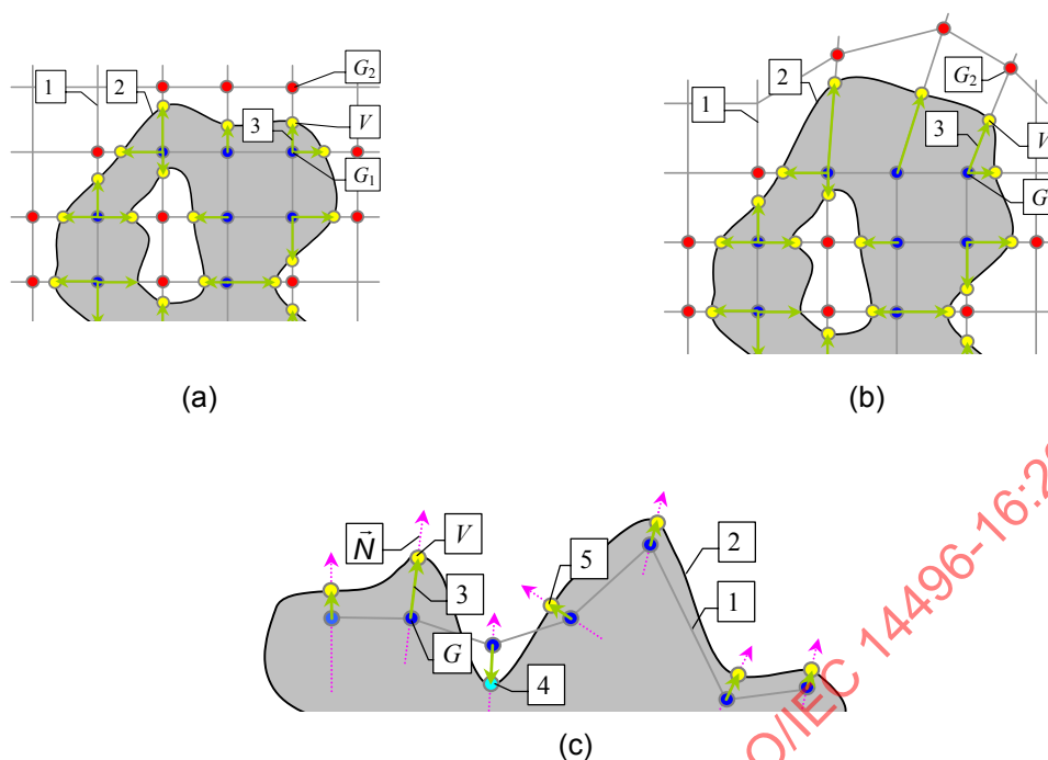
Figure 23 — A cross-section through a 3D object, illustrating the contour of the object, the reference-grid, and the relation between the vertices (belonging to the connectivity-wireframe and located at the surface of the object) and the grid points.
