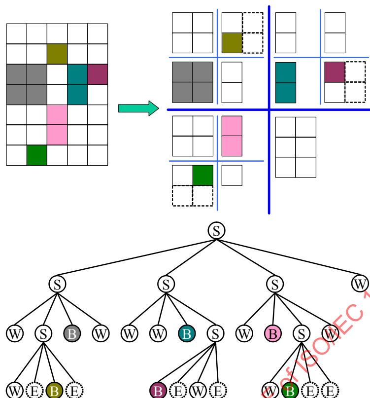
Figure 69 — Example of adjustable octree in the resolution of 5x7.
