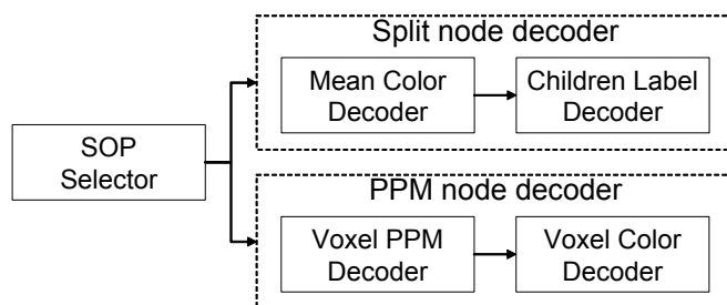
Figure 73 — Block diagram of tree node decoder.
