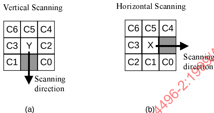
Figure V2 - 15 -- The context information at different scanning of SI
