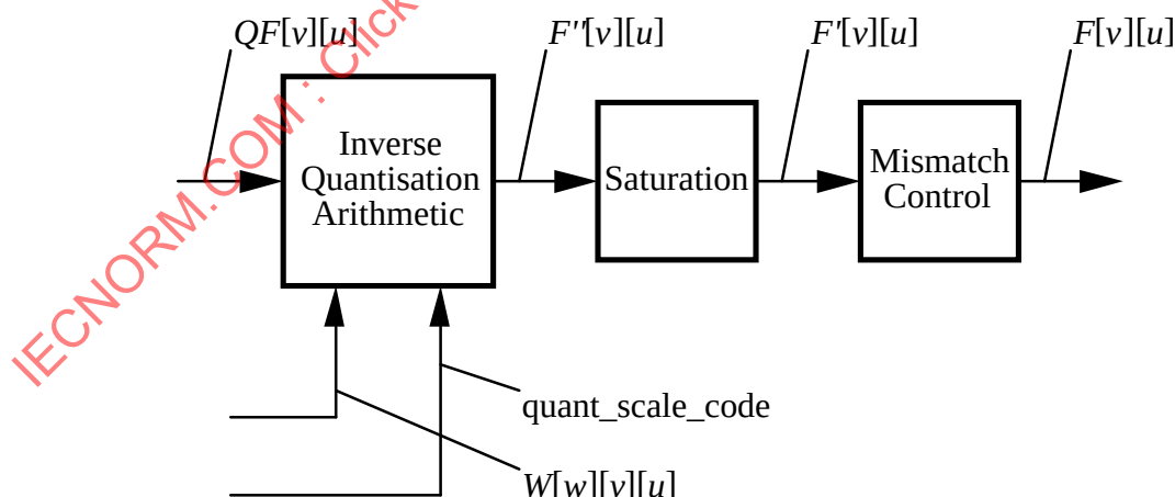
Figure 7-7 -- Inverse quantisation process
