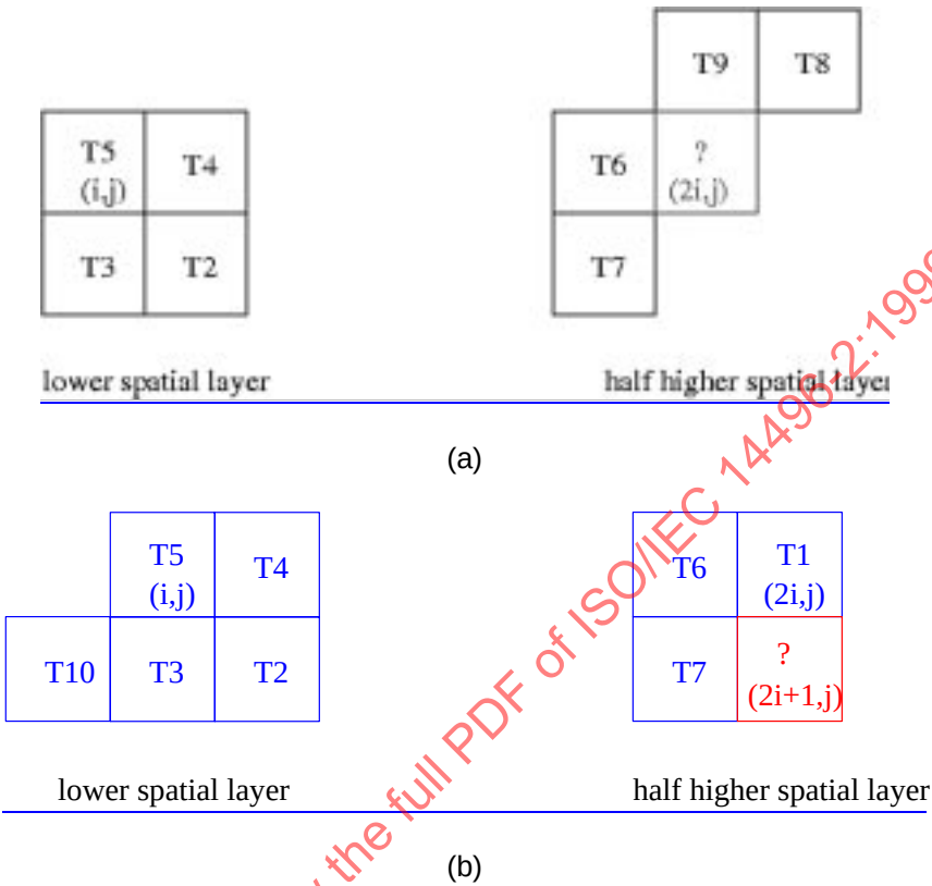
Figure V2 -36 -- The context used for vertically enhanced exceptional BABs
