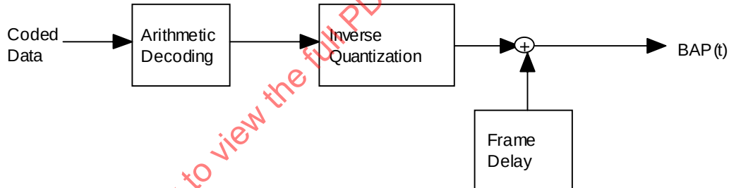
Figure V2 -38 -- BAP predictive coding
