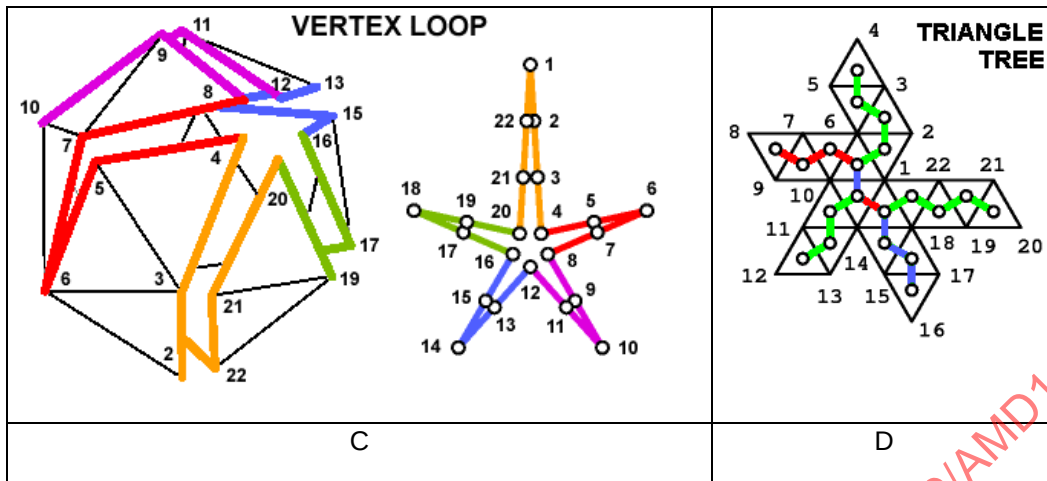
Figure V2 - 42 -- Topological Surgery representation of a simple mesh.
