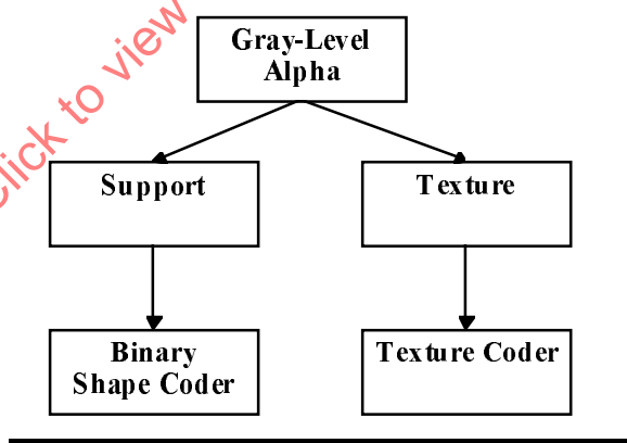
Figure 7-15 -- Grayscale shape coding
