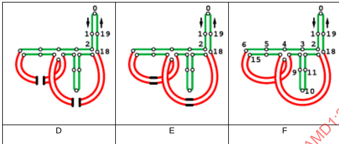
Figure V2 -46 -- Steps to build the bounding loop from the vertex graph.
