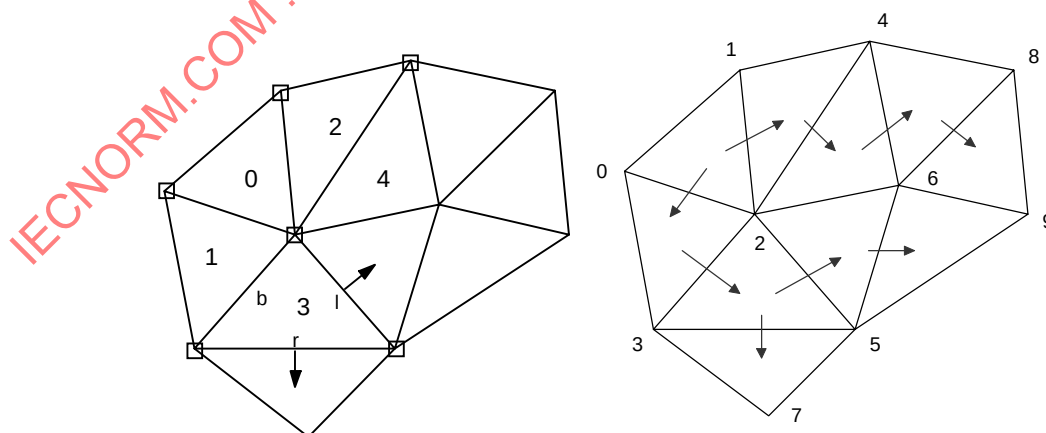
Figure 7-46 -- Breadth-first traversal of a 2D triangular example mesh
