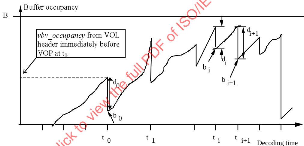
Figure D-2 -- VBV Buffer occupancy
