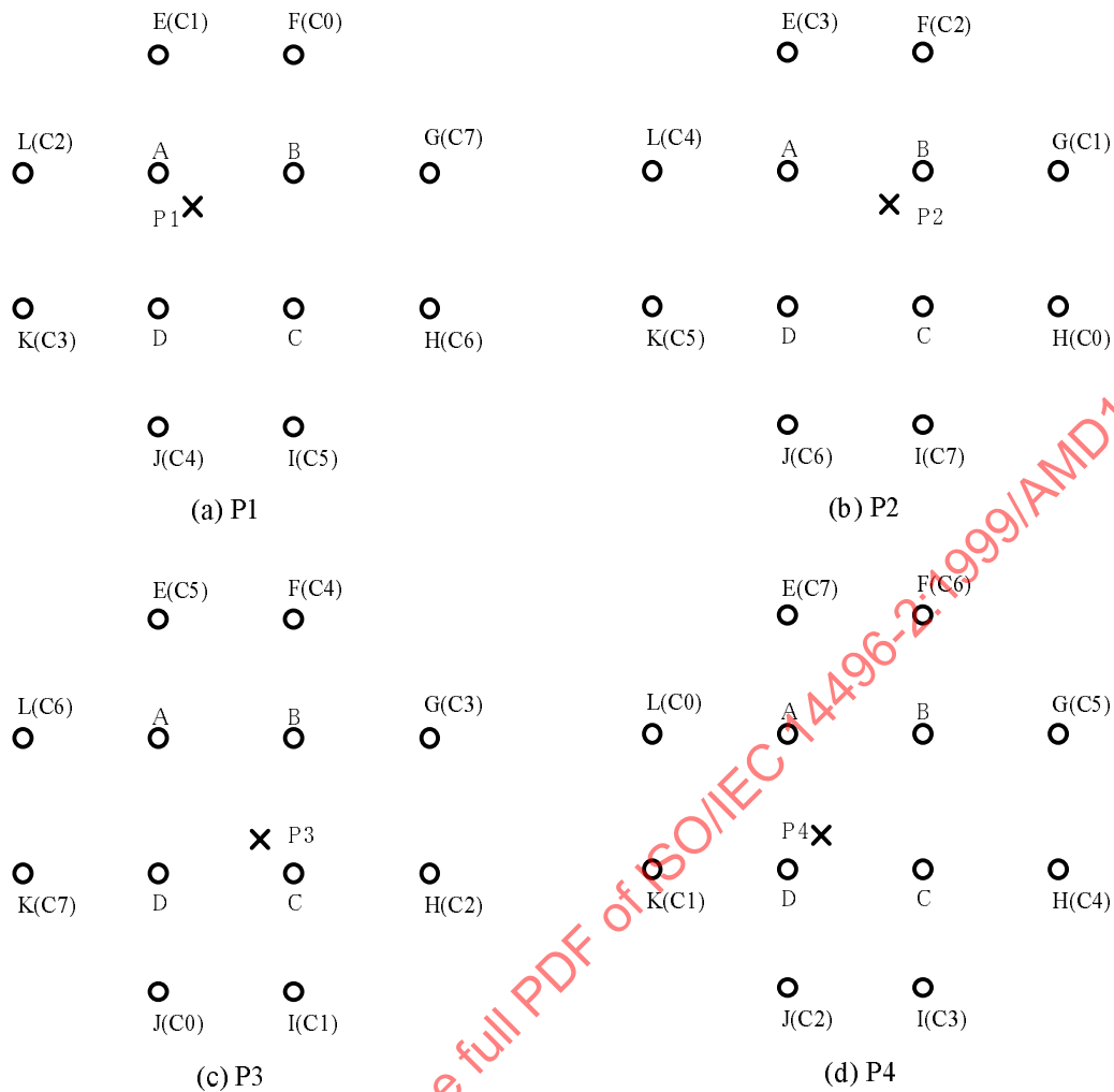
Figure 7-14 -- Interpolation filter and interpolation construction
