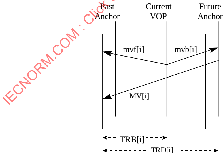
Figure 7-29 -- Interlaced direct mode
