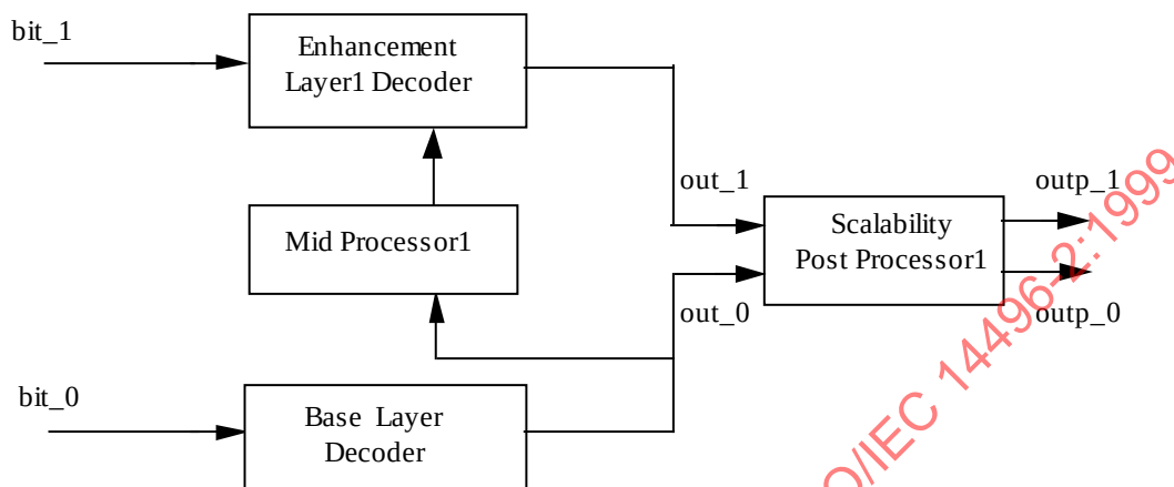
Figure 7-32 -- High level decoder structure for generalized scalability
