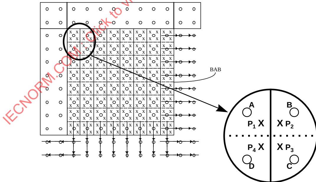
Figure 7-13 -- Upsampling
