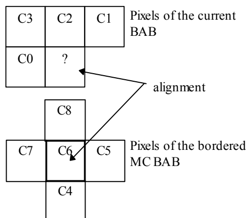
Figure V2 - 16 -- The templates of Inter-mode CAE for enhancement layer. C6 is aligned with the pixel to be decoded. The pixel to be decoded is marked with '?'. IECNORM.COM : Click to view the full PDF of ISO/IEC 14496-2:2001
