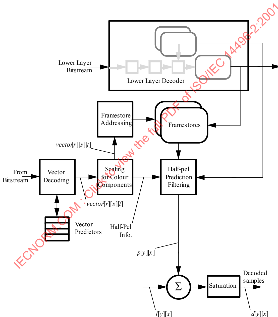
Figure 7-33 -- Simplified motion compensation process for temporal scalability
