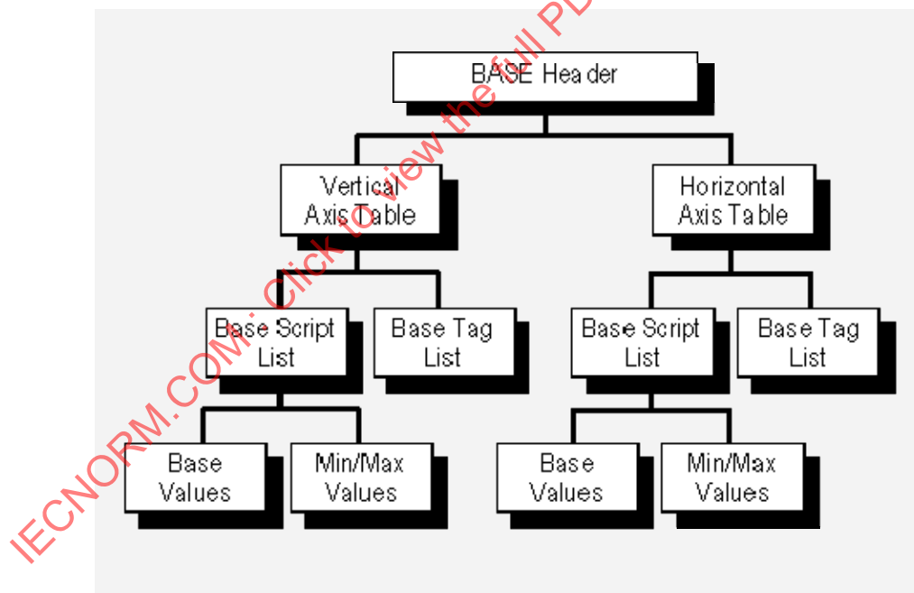
Figure 21 – High-level organization of BASE table
