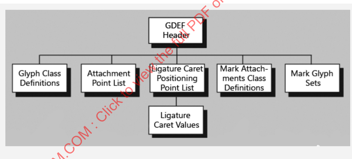
Figure 22 – High-level organization of GDEF table
