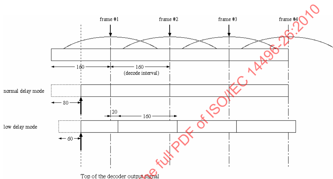
Figure 3 — Decoder output signal timing for testing decoder conformance
