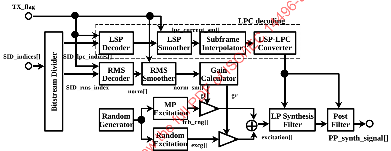
Figure 33: CNG module
