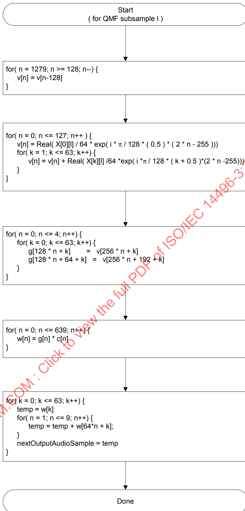
Figure 4.42 – Flowchart of decoder synthesis QMF bank
