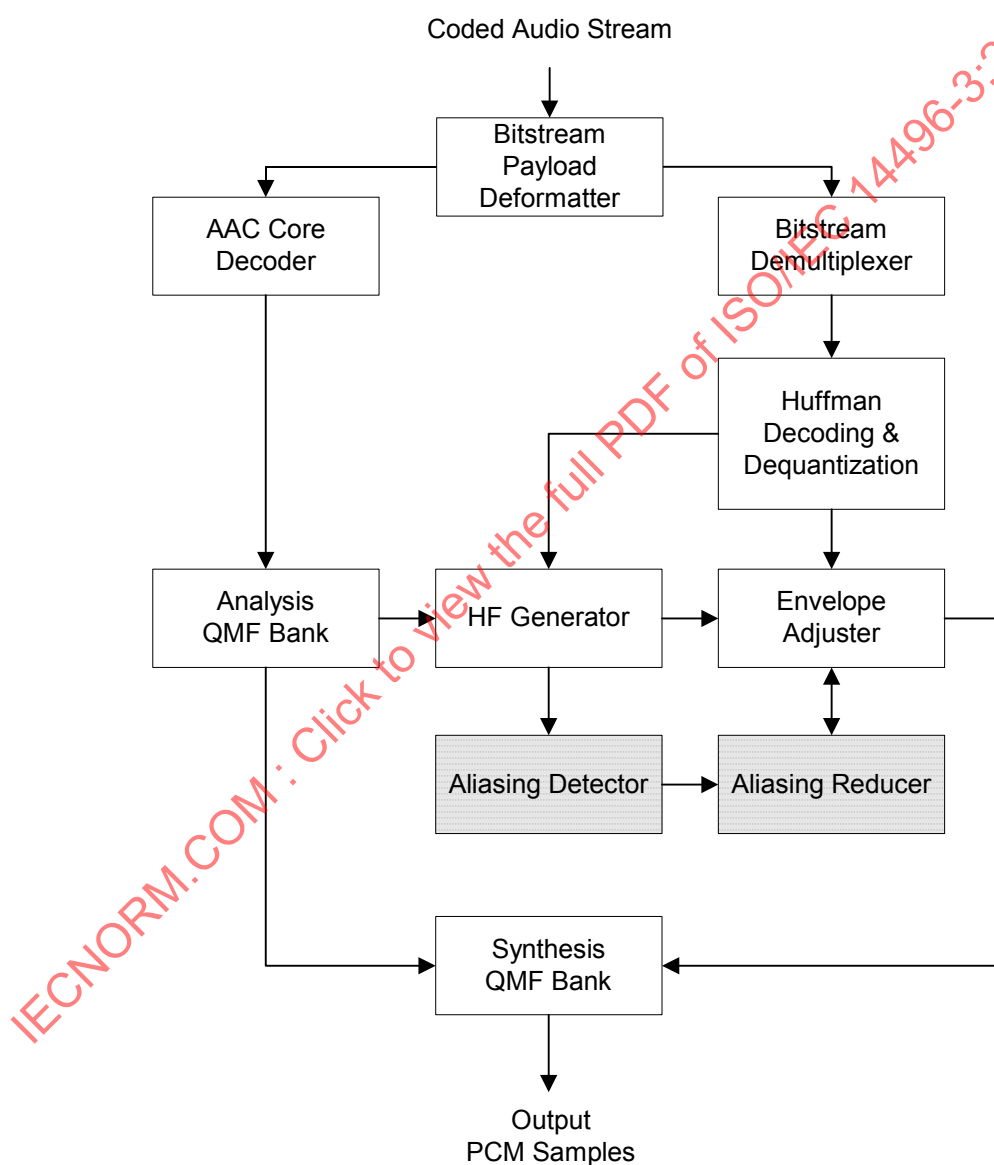
Figure 4.47 – Block diagram of the SBR low power decoder
