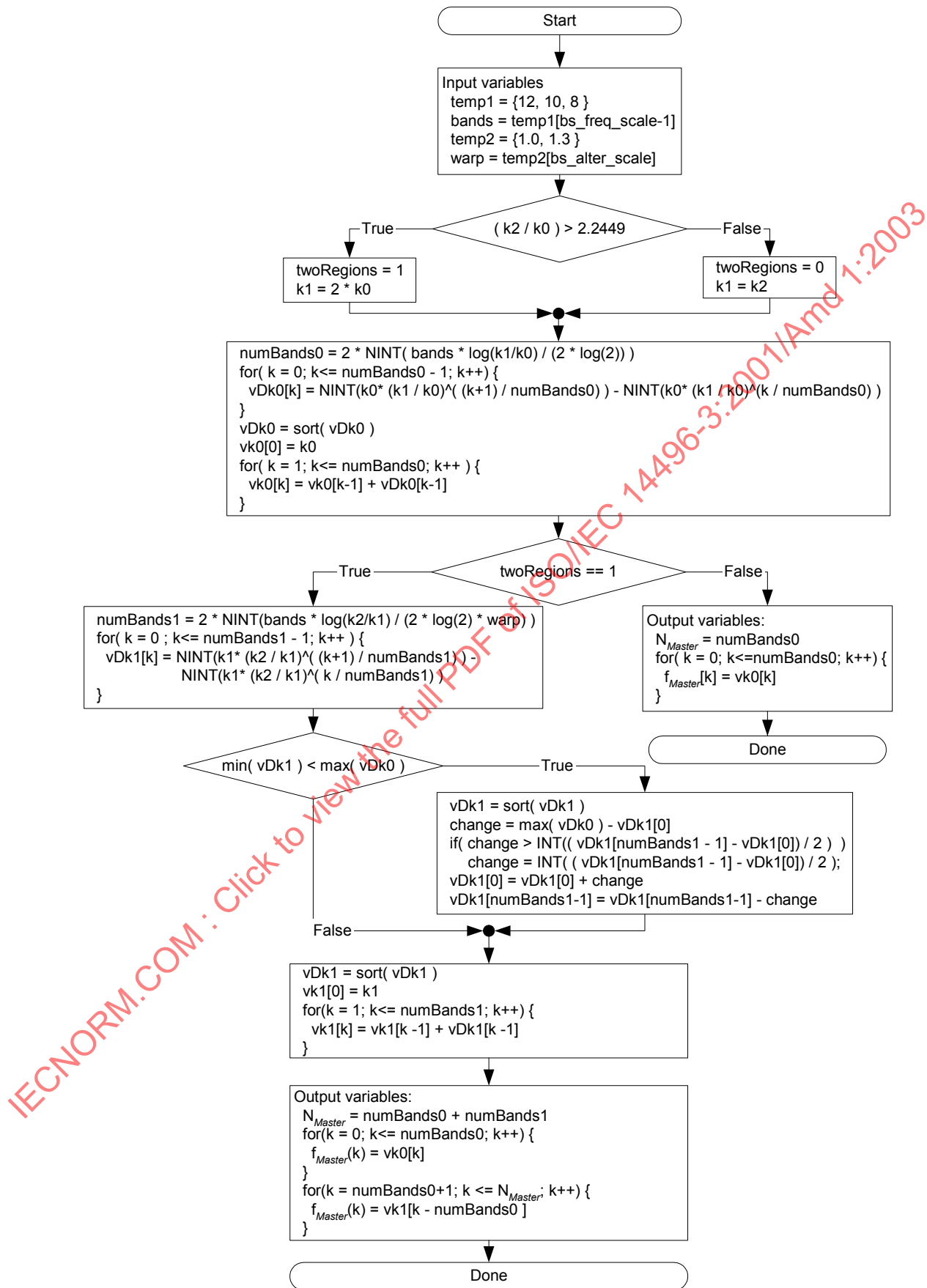
Figure 4.39 – Flowchart calculation of f_{Master} when bs\_freq\_scale > 0
