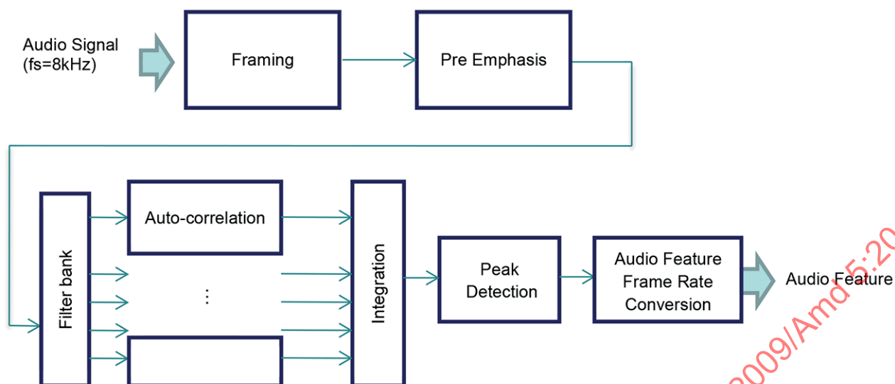
Figure 13.2 — Block diagram of Audio Feature Extraction Tool
