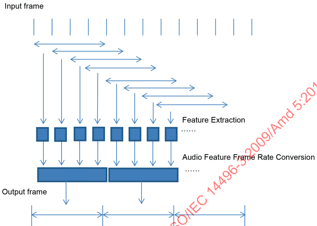
Figure 13.3 — Audio framing structure of Audio Feature Extraction tool
