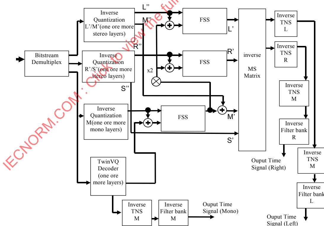
Figure 4.10 – Decoding of a TwinVQ (mono) AAC (mono) and AAC (stereo) configuration, TwinVQ does use TNS
