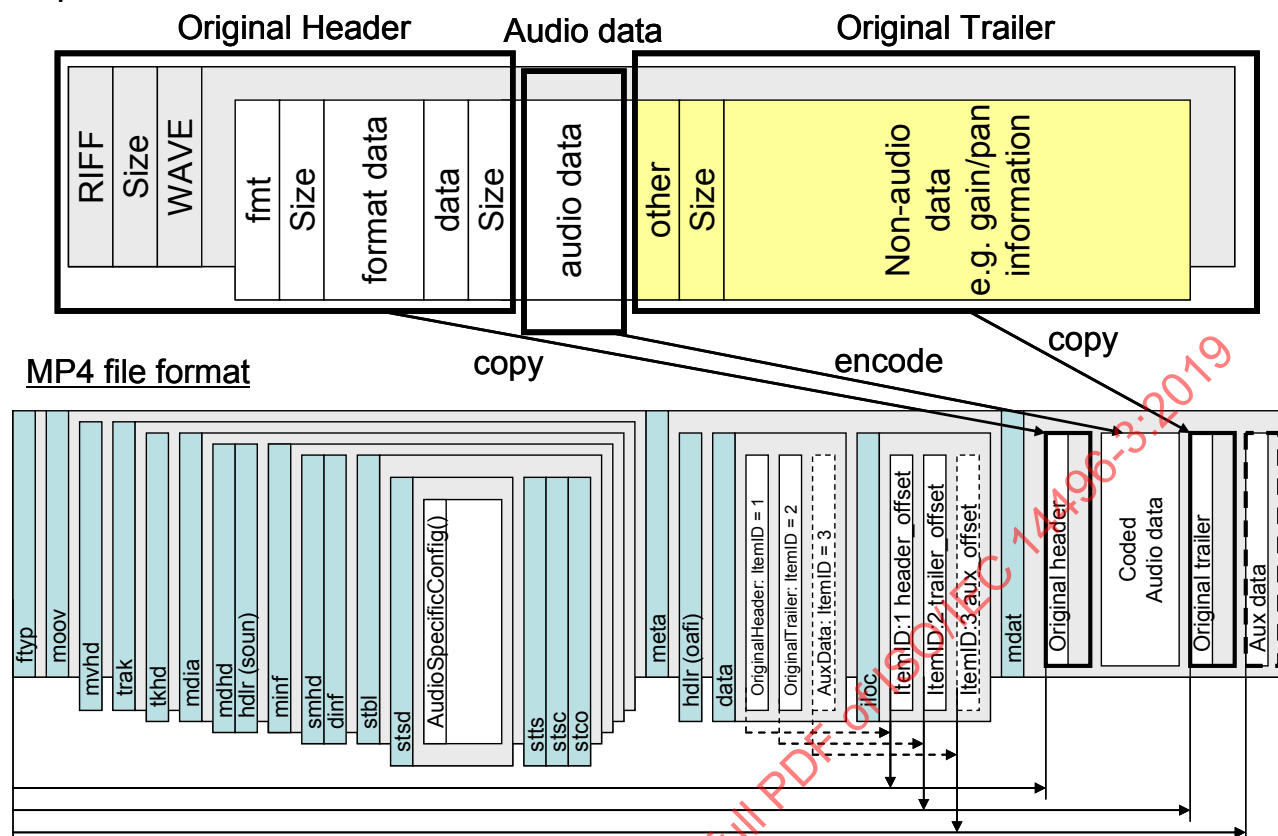
Figure 1.2 – Possible order of blocks
