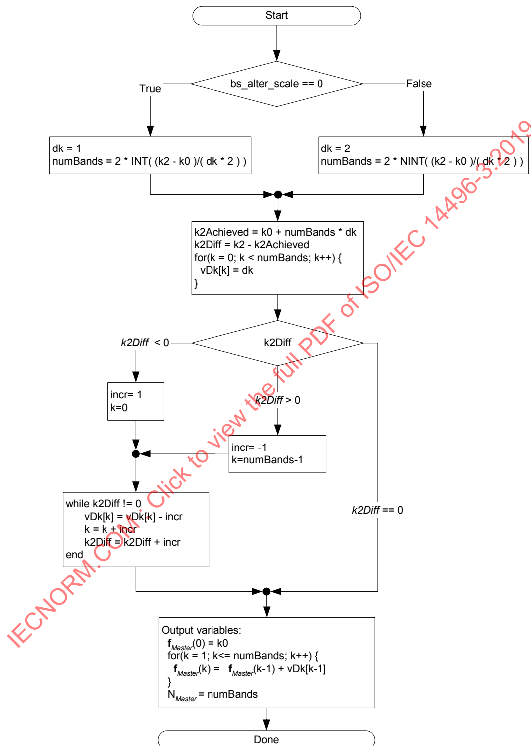
Figure 4.39 – Flowchart calculation of f_{Master} when bs\_freq\_scale = 0
