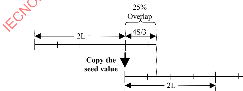
Figure 8.15 — The start-seed value used in the next interval is copied from the previous interval at the corresponding time location
