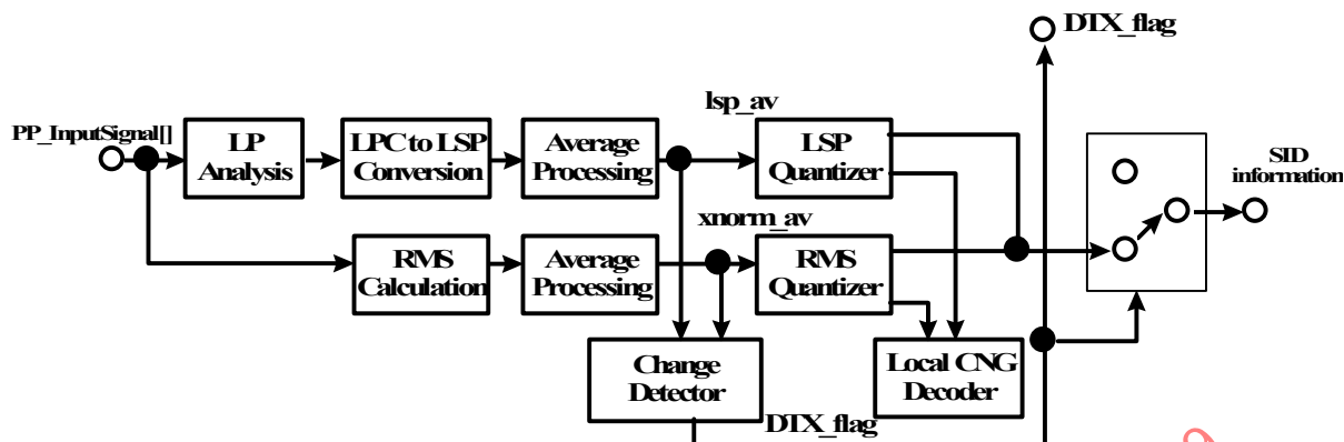
Figure 3.B.2 — DTX module
