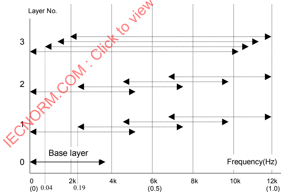
Figure 4.30 – Example of adaptive active band selection. (Sampling_Frequency=24kHz, Total bitrate=40kbit/s(8+8+8+16kbps) In this case, q_{\text{sample}} = 0.43 , \text{bias} = 0.19 for layer 1 and layer 2 q_{\text{sample}} = 0.87 , \text{bias} = 0.04 for layer 3)
