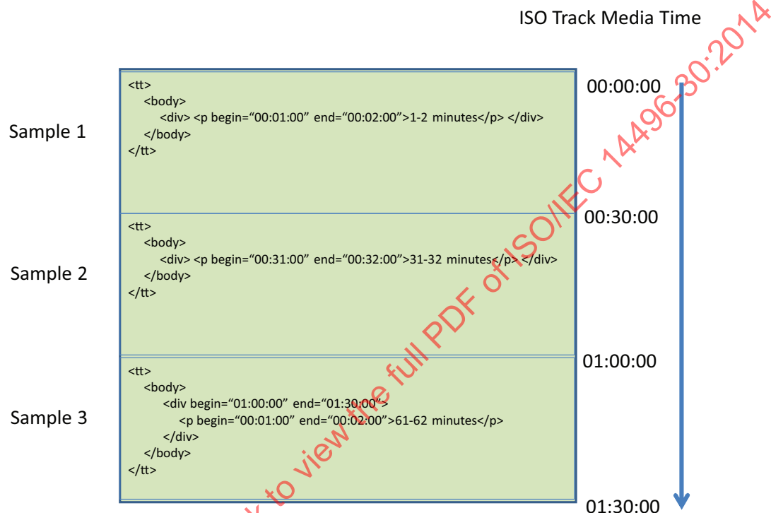
Figure 1 — Example of a TTML track with three samples
