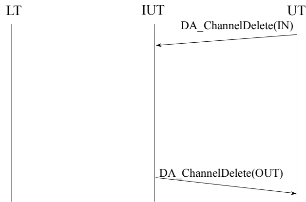
Figure 22 — Channel Delete for Local Storage
