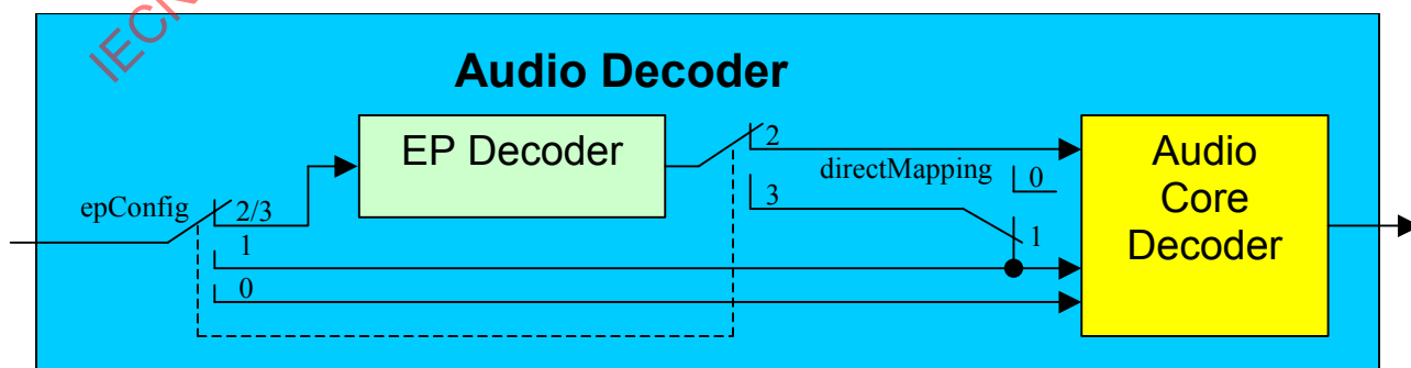
Figure 5 – Audio decoder structure
