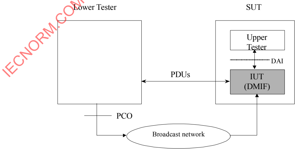
Figure 23 — The test method for the DAI test environment for a broadcast scenario
