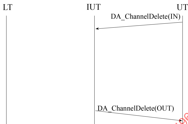
Figure 27 — Channel Delete for Broadcast
