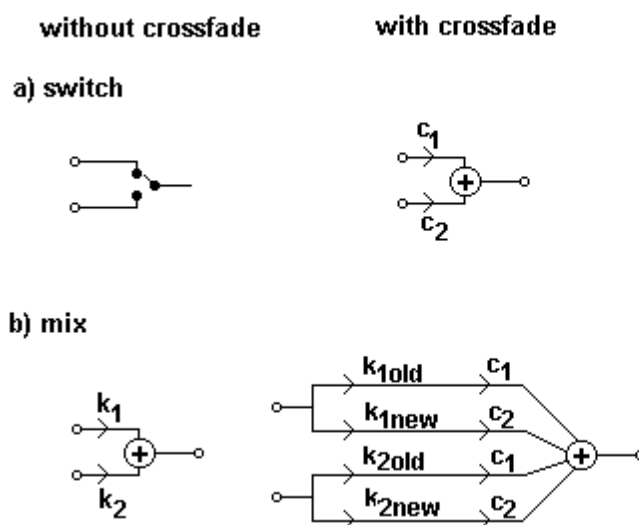
Figure 13 — Click free switch and mix
