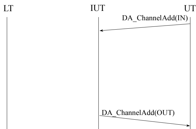
Figure 21 — Channel Add for Local Storage
