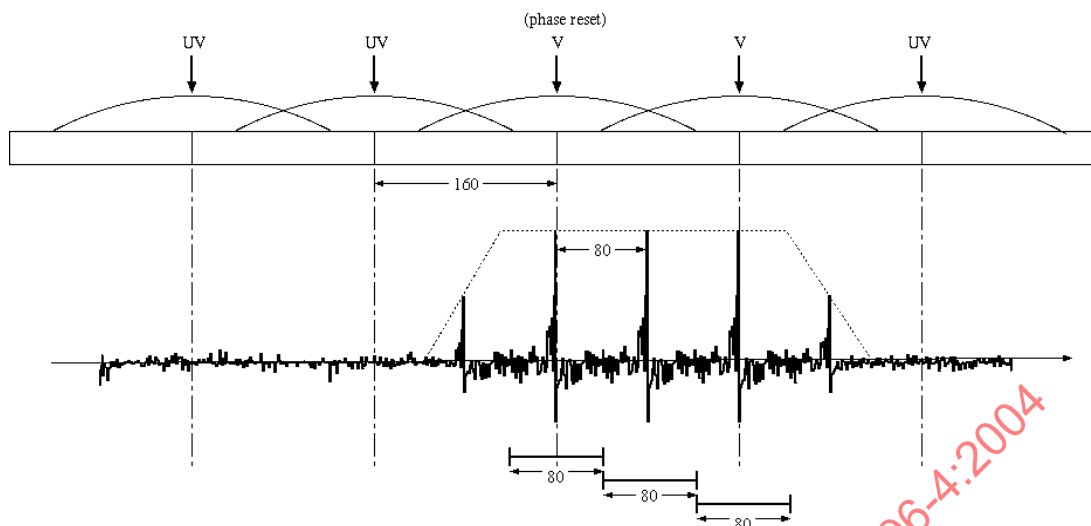
Figure 10— An example decoder output signal and HVXC framing timing
