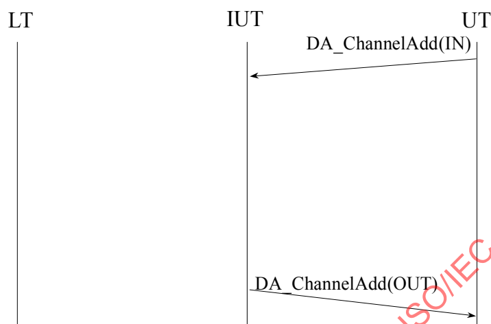
Figure 26 — Channel Add for Broadcast
