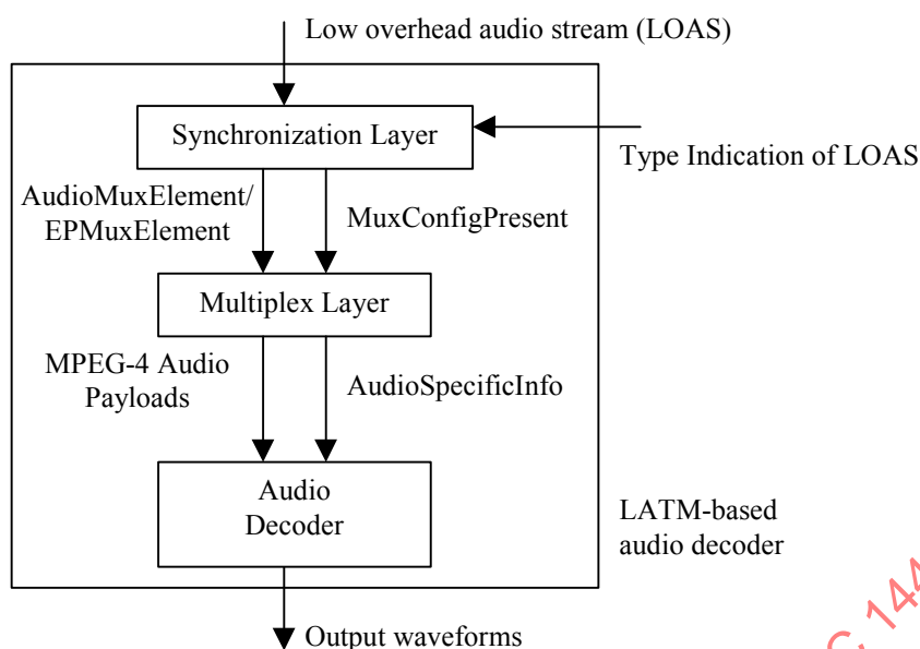
Figure 15 – Audio Conformance Points for LATM-based decoders
