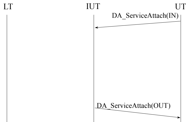
Figure 19 — Service Attach for Local Storage
