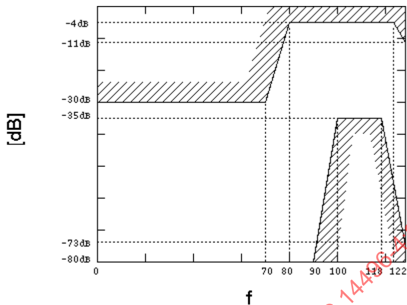
Figure 8 — Acceptable range of differential spectrum (for bitstream HV01)
