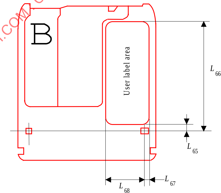
Figure 14c - User label area on Side B
