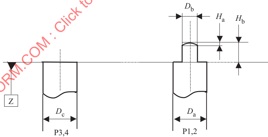
Figure C.1 - Compliance gauge
