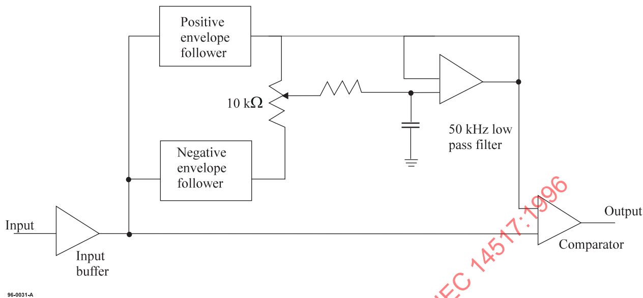
Figure H.1a - Tracking threshold block diagram
