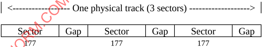
Figure 22 - Track format in the PEP Zone
