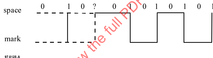
Figure 19 - Postamble pattern
