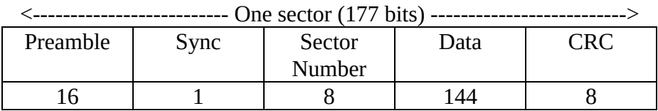
Figure 23 - Sector format in the PEP Zone
