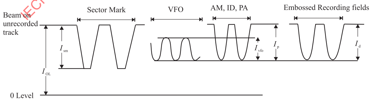
Figure 24c - Signals from Headers and embossed Recording fields in Channel 1
