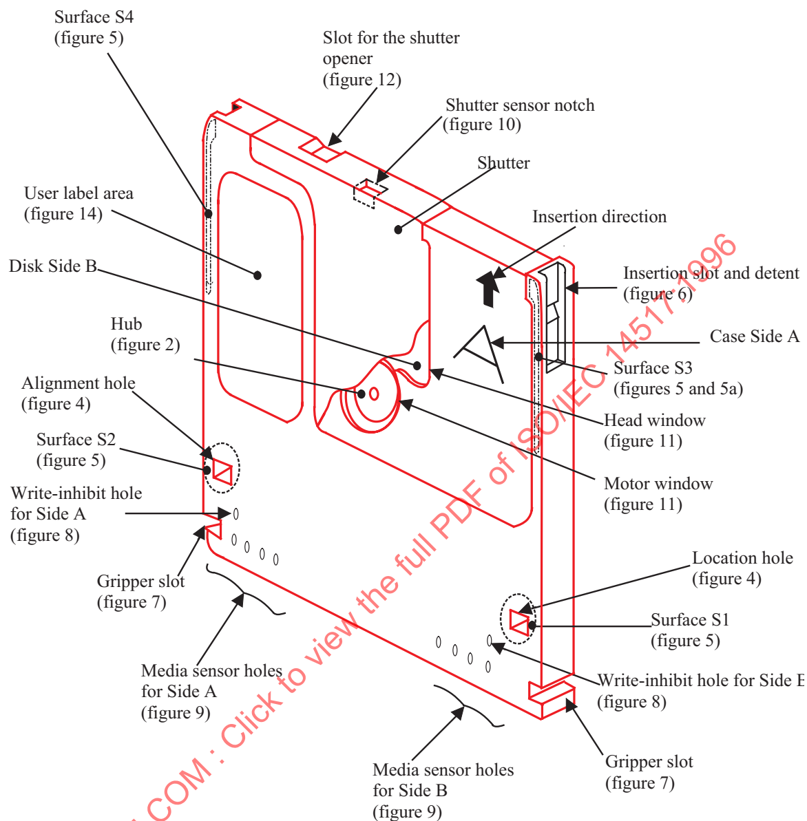
Figure 3 - Case
