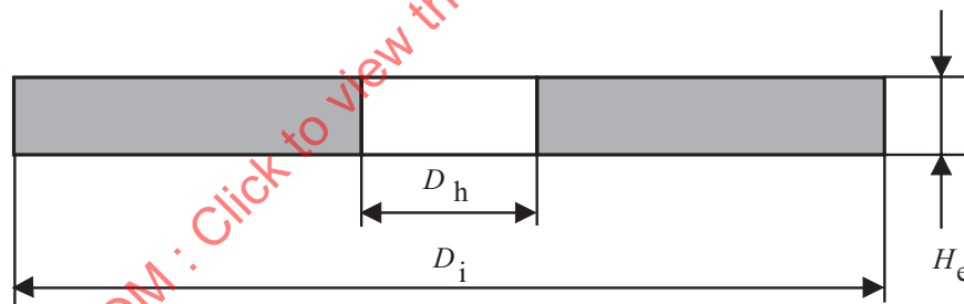
Figure D.1 - Test device for the clamping characteristic of the hub
