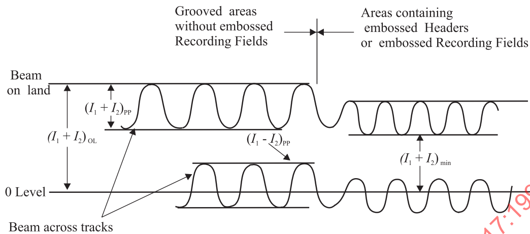
Figure 24a - Signals from grooves in the Tracking Channel
