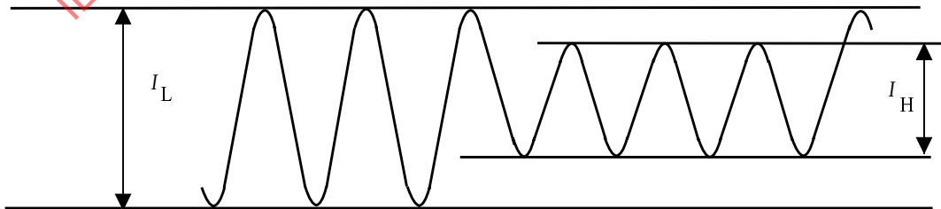
Figure 26 - Definition of I_L and I_H
