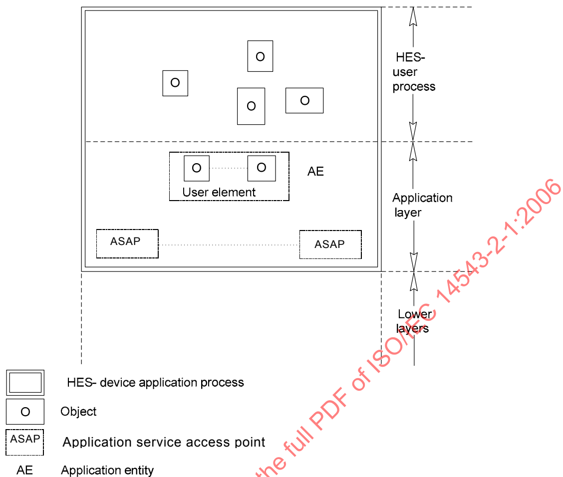
Figure 4 – HES device application process model
