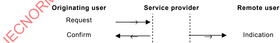
Figure 4 – Exchange of primitives for the L_Data-Service
