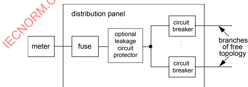
Figure 5 – Example of a typical PL topology
