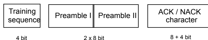
Figure 8 – Structure of an acknowledgement frame
