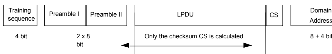
Figure 7 – Structure of a datagram
