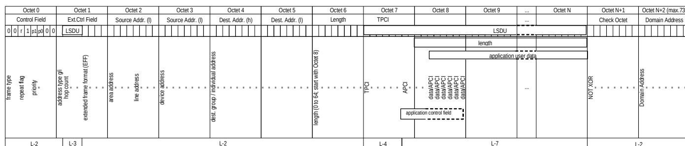
Figure 20 – Format 1e, L_Data_Extended request frame format
