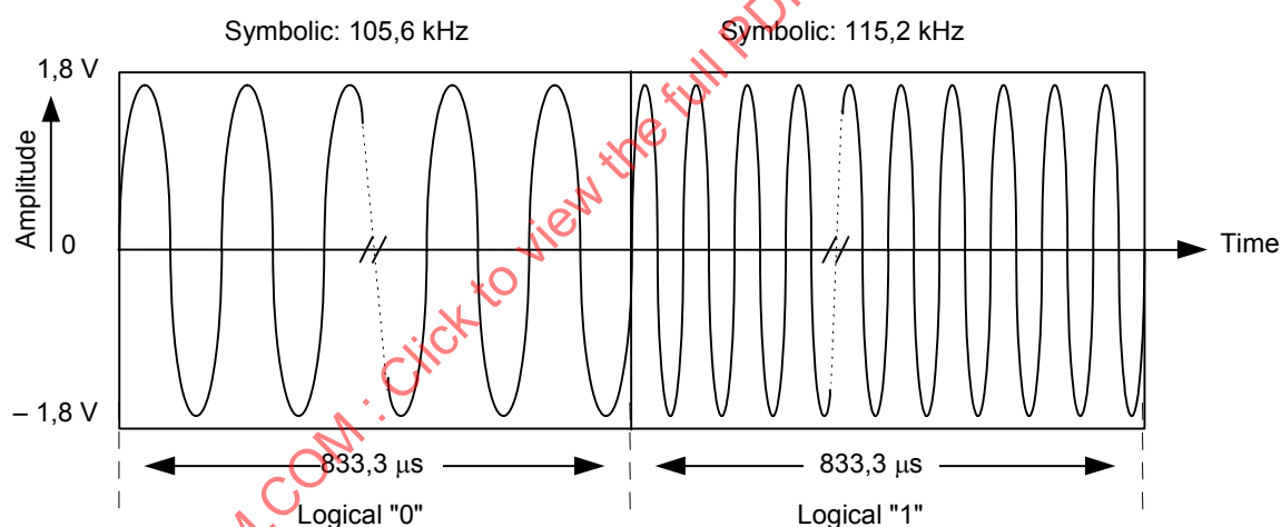
Figure 2 – Signal encoding
