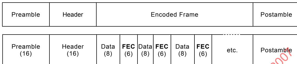
Figure 24 – Complete frame encapsulation (Datagram)
