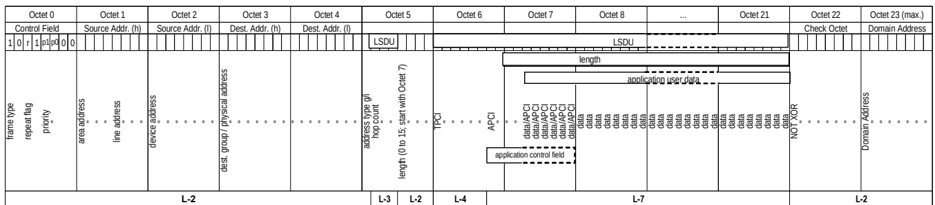
Figure 16 – Format 1s, L_Data_Standard request frame format
