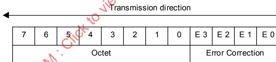
Figure 6 – Character
