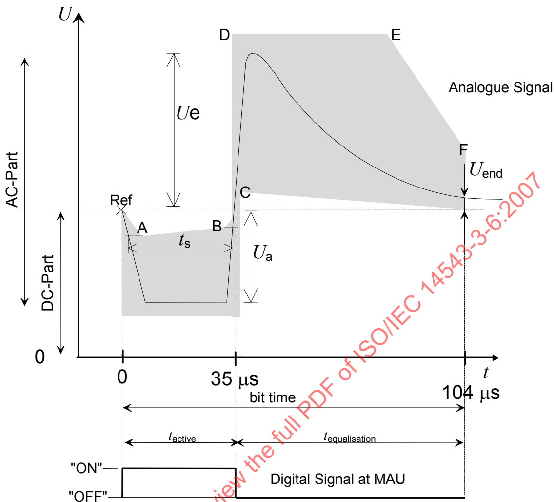
Figure 24 – “0”-Bit frame
