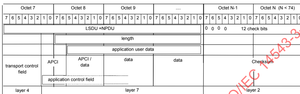
Figure 20 – Format 1e, Full L_Data_Extended request frame format
