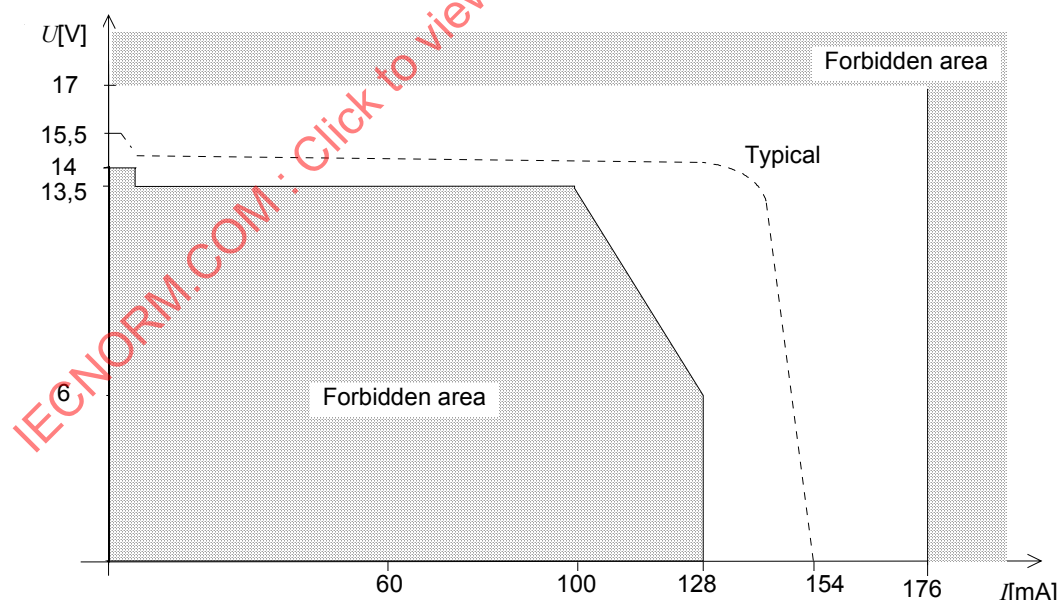
Figure 10 – Voltage/Current gauge of entire distributed power supply with 6 to 8 supply nodes
