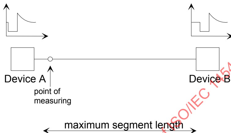
Figure 25 – Delayed logical “0”
