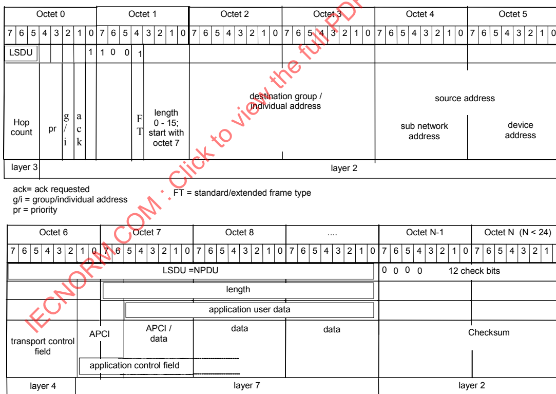
Figure 19 – Format 1s, Full L_Data_Standard request frame format
