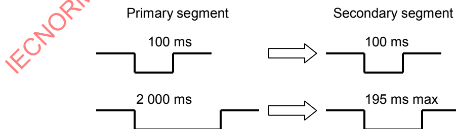
Figure 4 – Repeater maximum transition time
