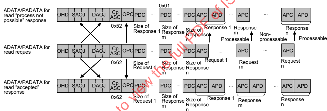
Figure 35 – Relationship among read request (requiring a response), read accepted response and read process not possible response
