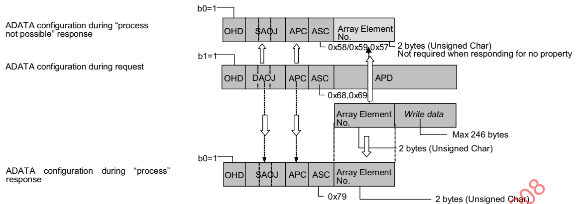
Figure 26 – Relationship among property value element-stipulated addition request, property value element-stipulated addition "accepted" response and property value element-stipulated addition "process not possible" response
