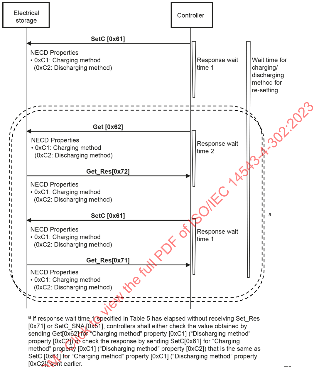
Figure 12 – Sequence for setting "Charging method" property (or "Discharging method" property) when no response is received from the storage battery
