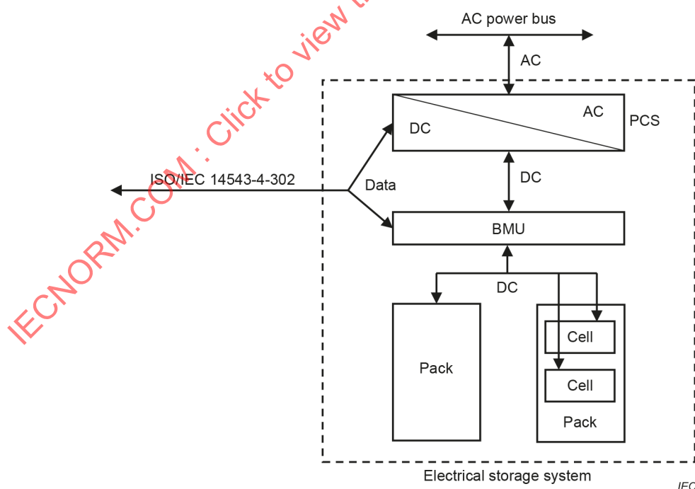
Figure 2 – Example of electrical storage system configuration and components
