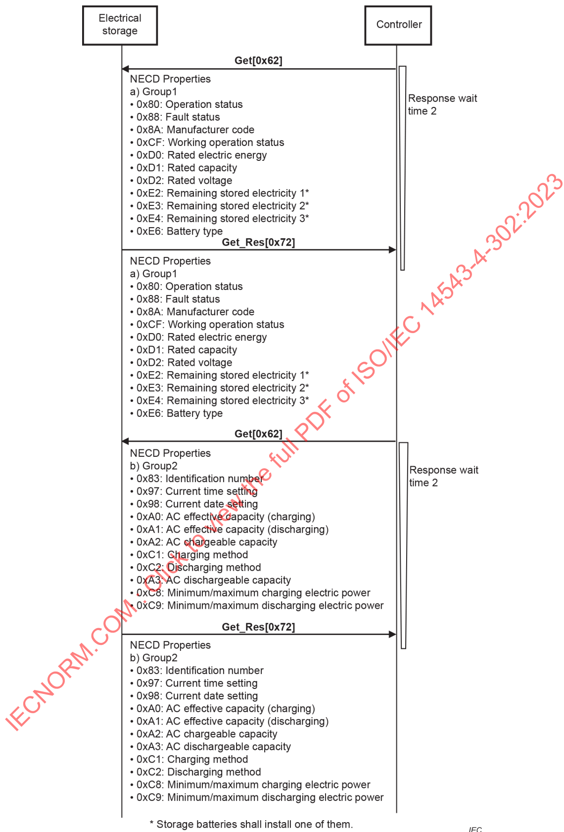
Figure 7 – Sequence of obtaining electrical storage system attribute information
