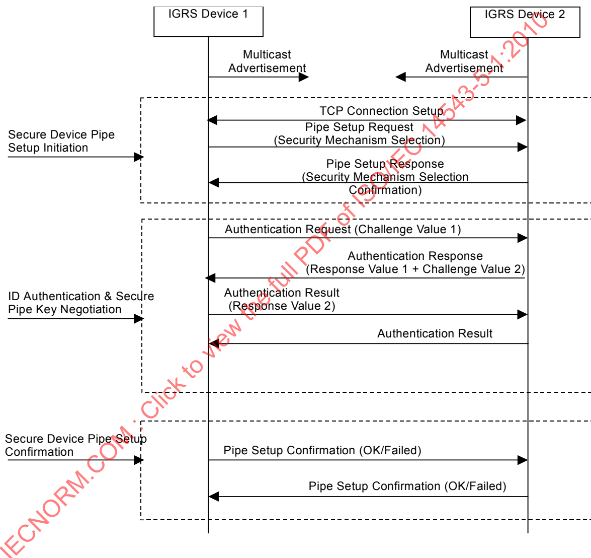
Figure 4 – Secure device pipe setup
