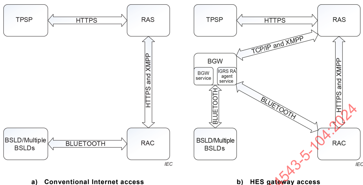
Figure 1 – Interaction models of Bluetooth smart lock device in the server management framework
