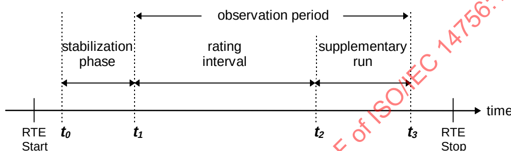
Figure 3 — Phases of the measurement procedure
