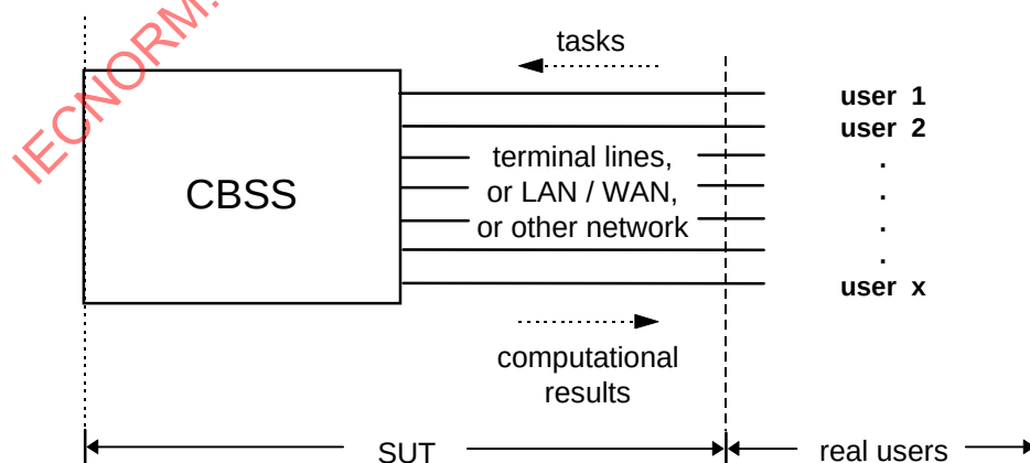
Figure 1 — CBSS in real operation
