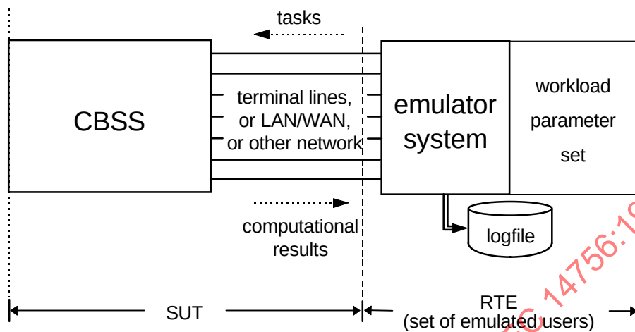
Figure 2 — CBSS in measurement
