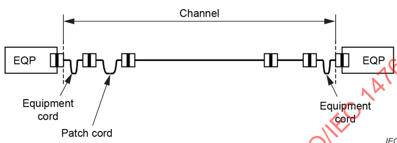
Figure 27 – Example of a cabling channel
