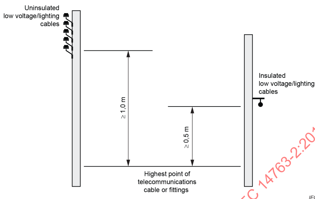
Figure 18 – Separation distances on supporting structures
