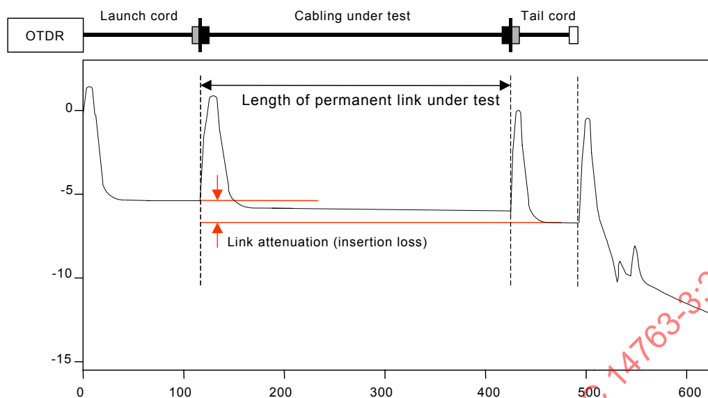
Figure 11 – OTDR measurement of installed cabling (permanent link)
