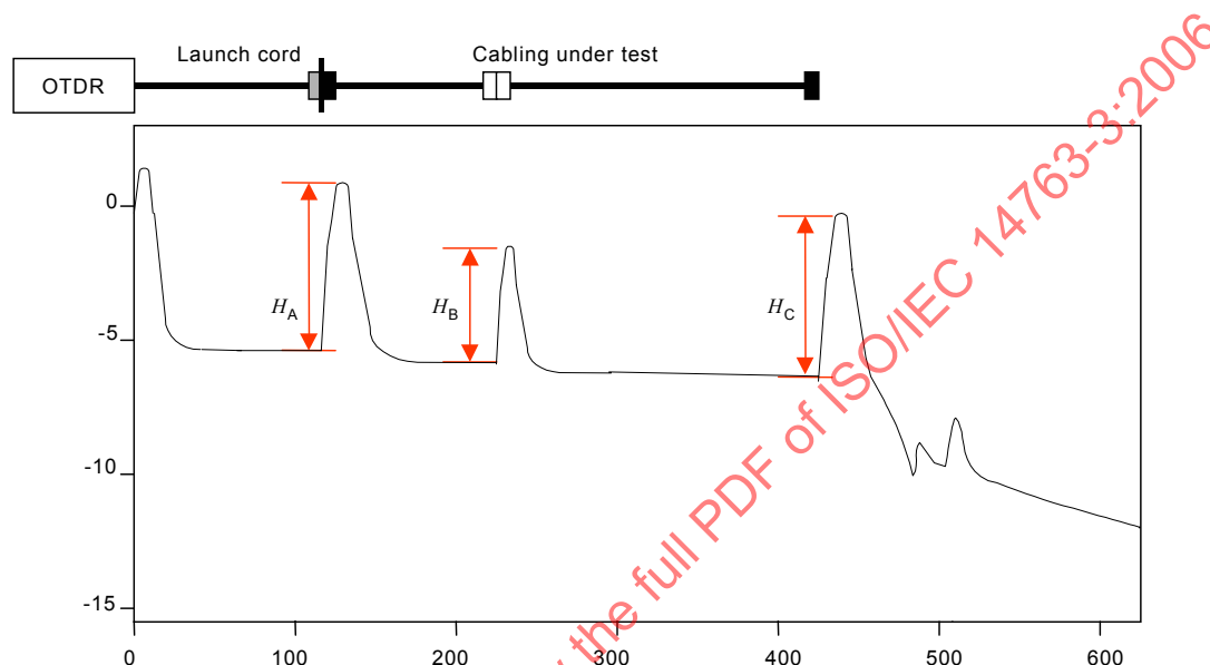
Figure 16 – OTDR measurement of return loss
