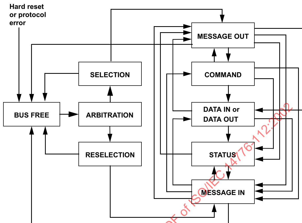
Figure 52 - Phase sequences
