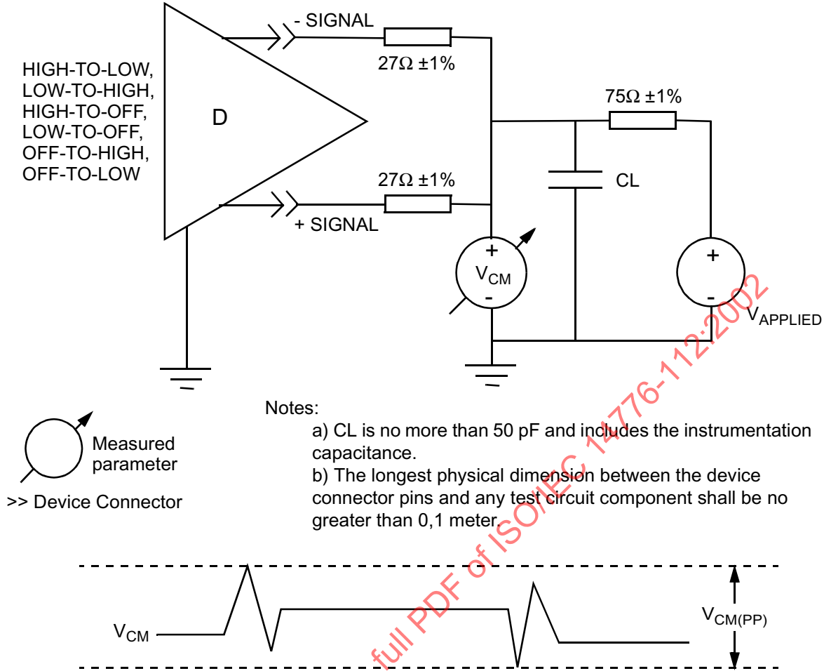
Figure A.9 - Driver offset switching voltage test circuit
