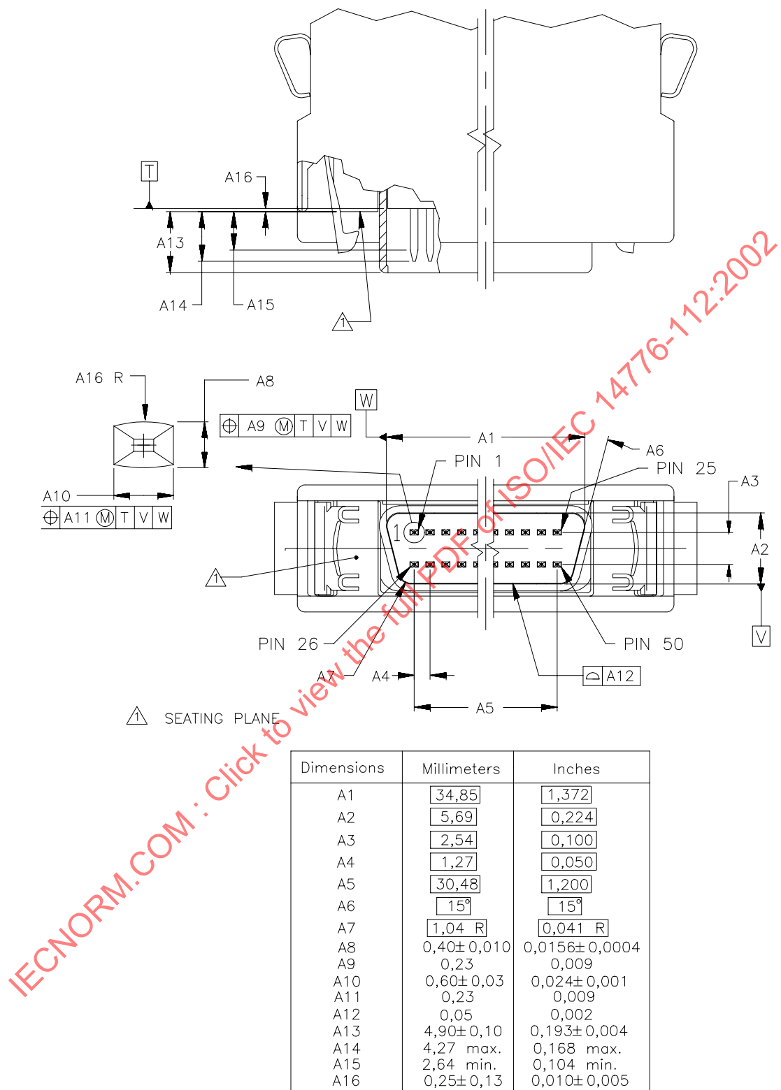
Figure 15 - 50-contact alternative 1 shielded mating connector (A cable)
