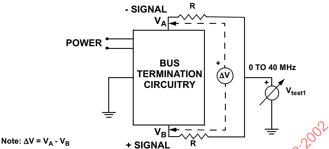
Figure 29 - Termination balance test configuration
