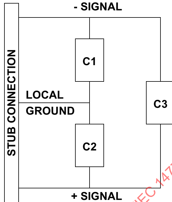
Figure 33 - Capacitive loads
