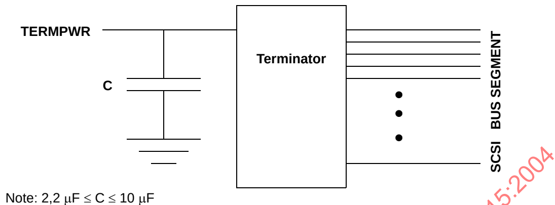
Figure 39 - Terminator decoupling example
