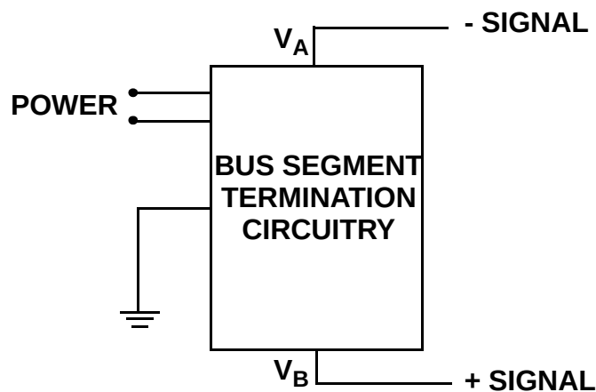
Figure 40 - LVD bus segment terminator
