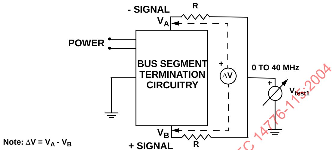
Figure 44 - Termination balance test configuration
