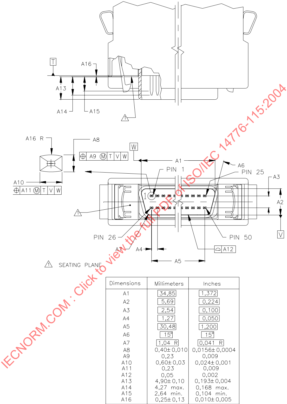
Figure 32 - 50-contact alternative 1 shielded mating connector (A cable)
