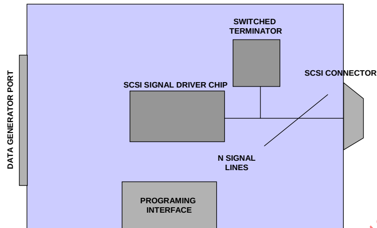
Figure 23 - SCSI signal driver board (FIX_ASY_3)
