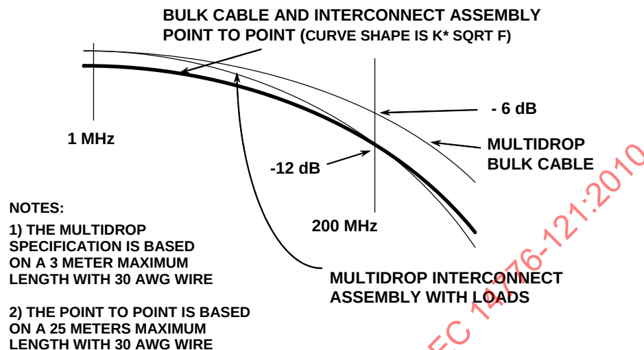
Figure 1 - Relationship between S21 for different configurations
