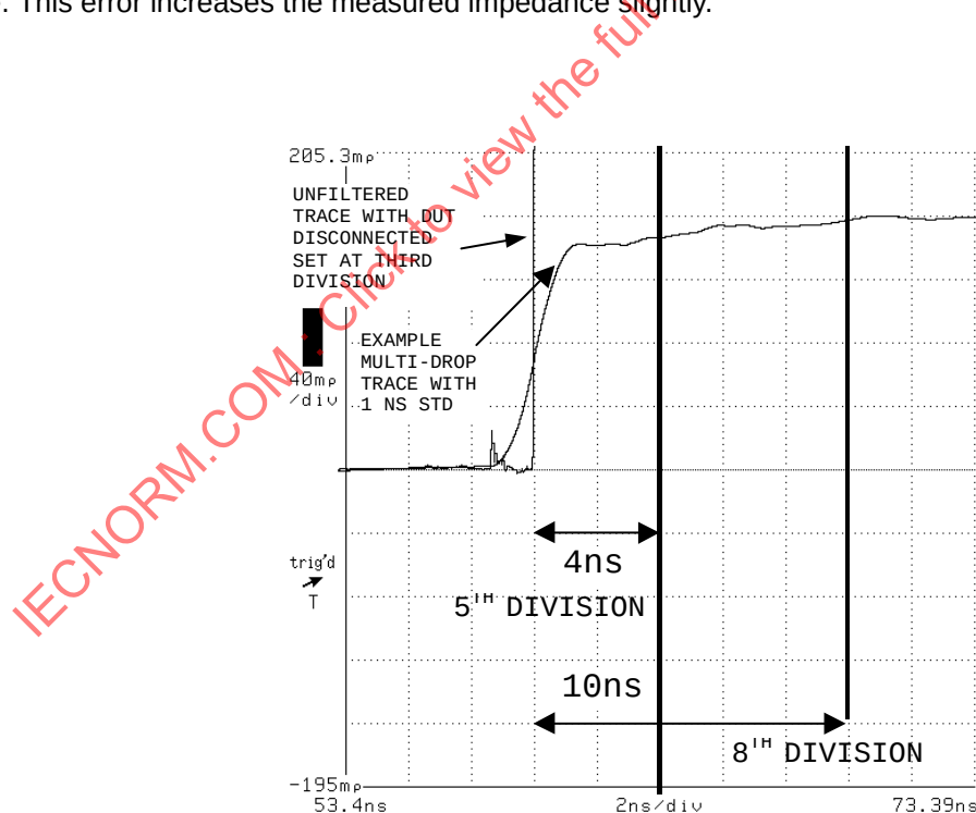
Figure 14 - Cursor placement for constant interval multi-drop cable
