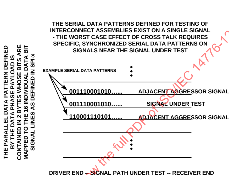
Figure 30 - Distinction between parallel and serial data in the same signal path
