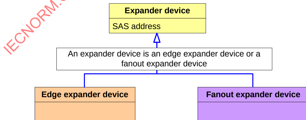
Figure 13 — Expander device object classes
