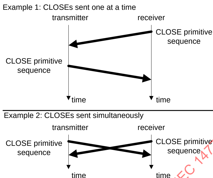
Figure 84 — Closing a connection example
