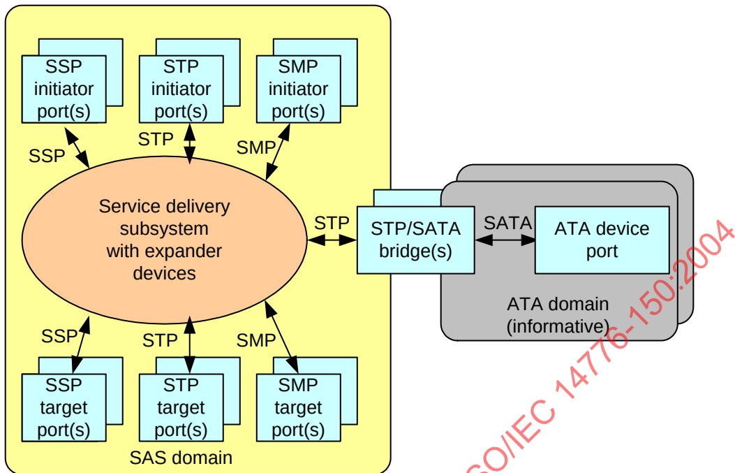
Figure 15 — SAS domain bridging to ATA domains
