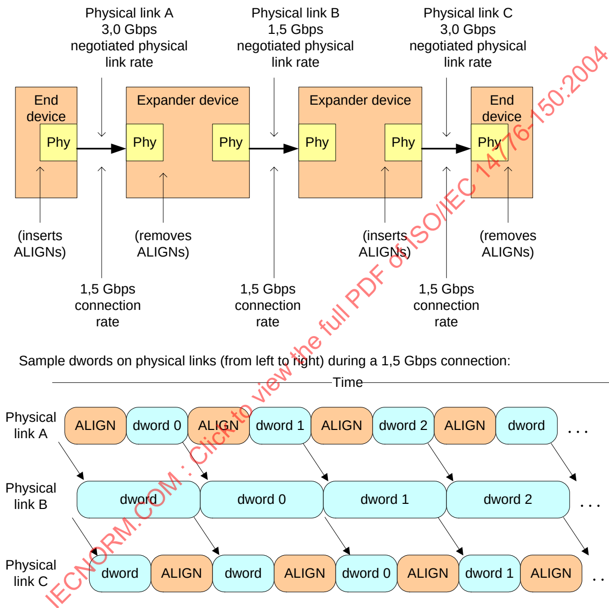
Figure 85 — Rate matching example
