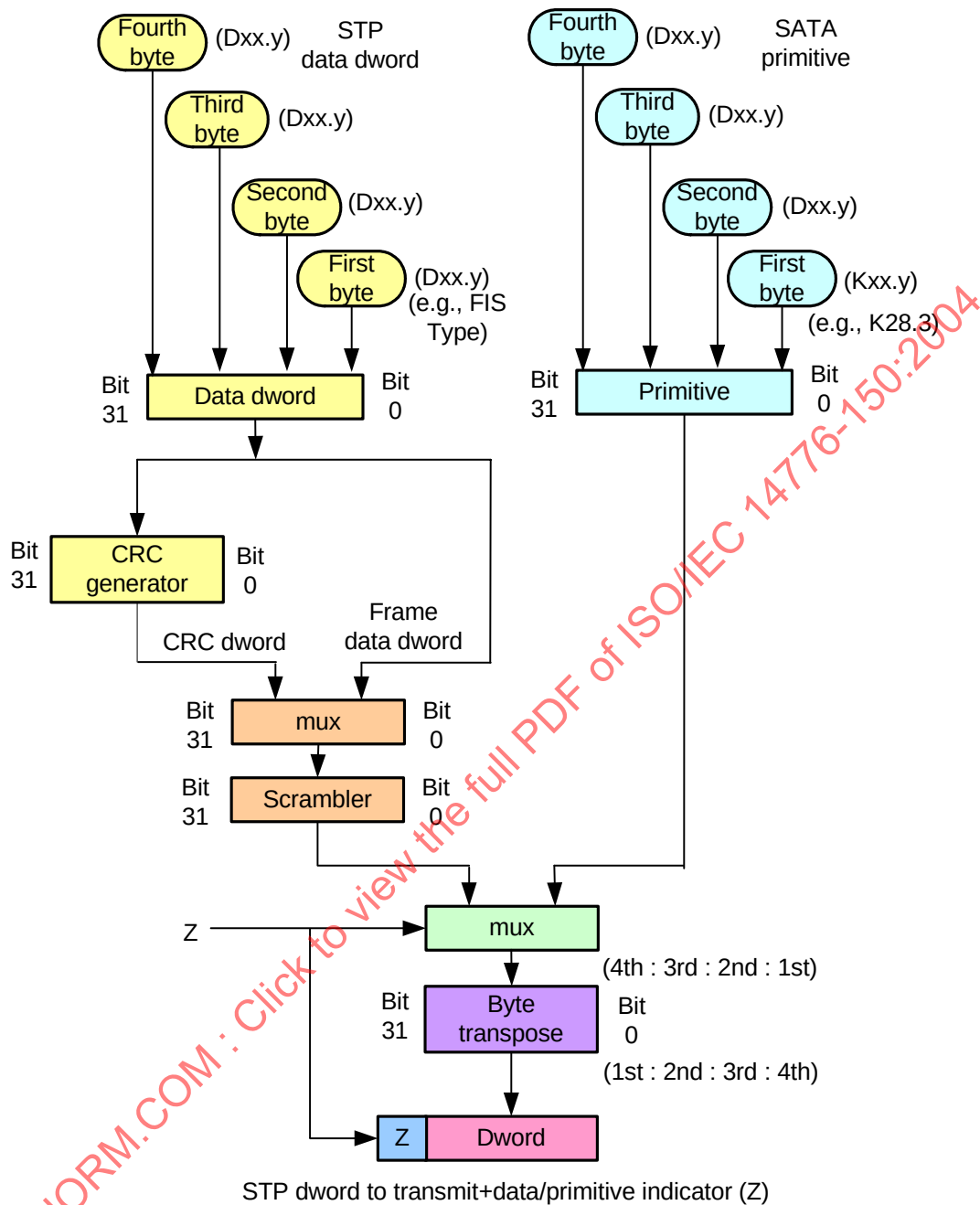
Figure 79 — STP transmit path bit ordering
