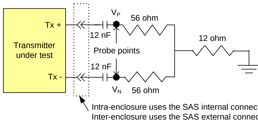
Figure 46 — Transmitter transient test circuit
