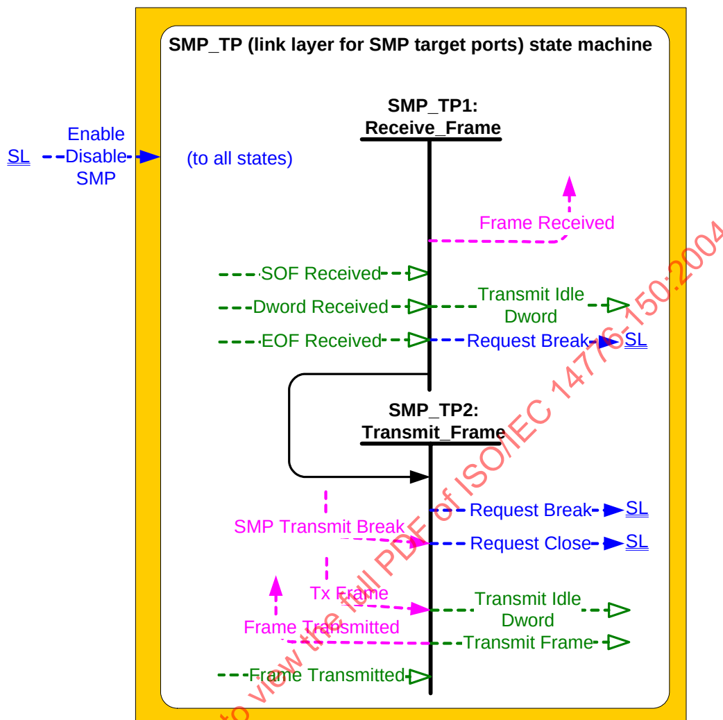
Figure 104 — SMP_TP (link layer for SMP target phys) state machine
