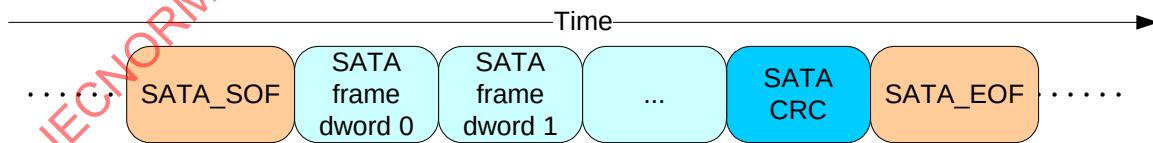
Figure 98 — STP frame transmission
