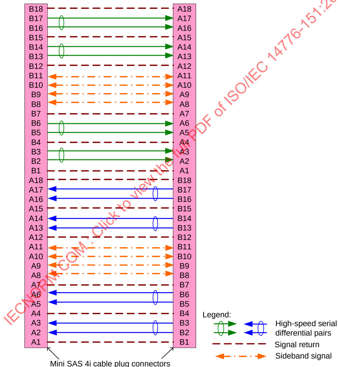
Figure 79 — SAS internal symmetric cable assembly - Mini SAS 4i
