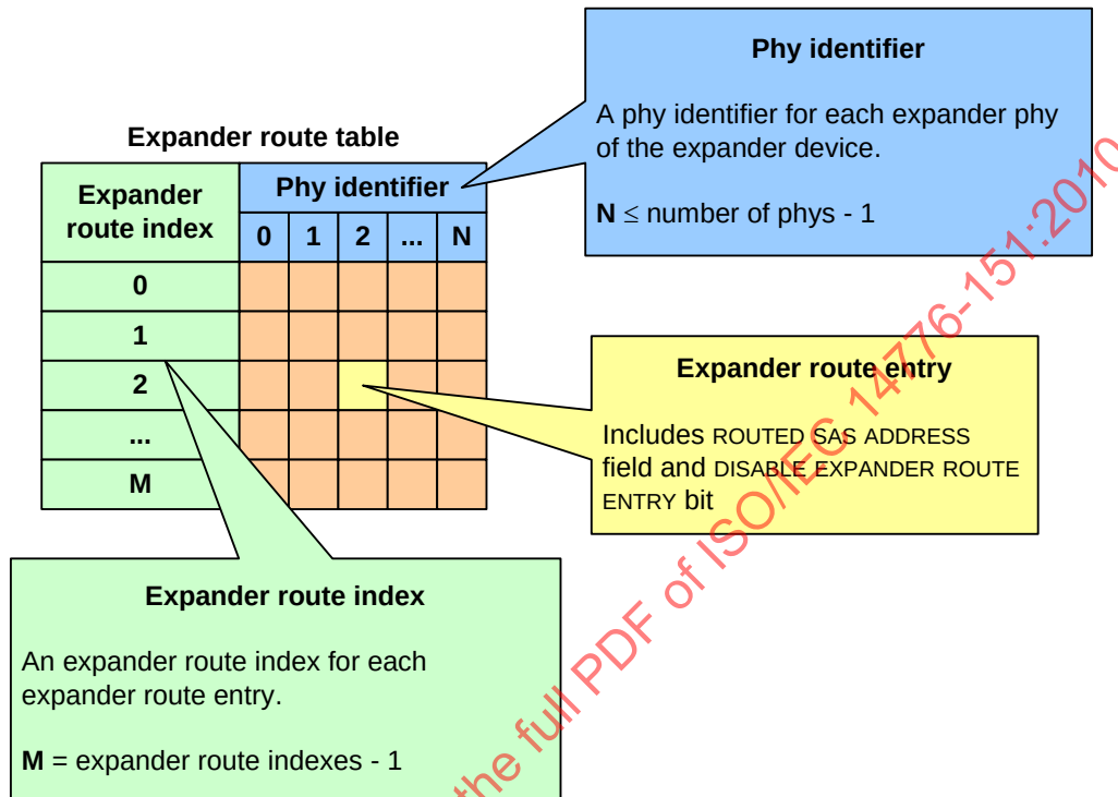
Figure 45 — Expander route table example
