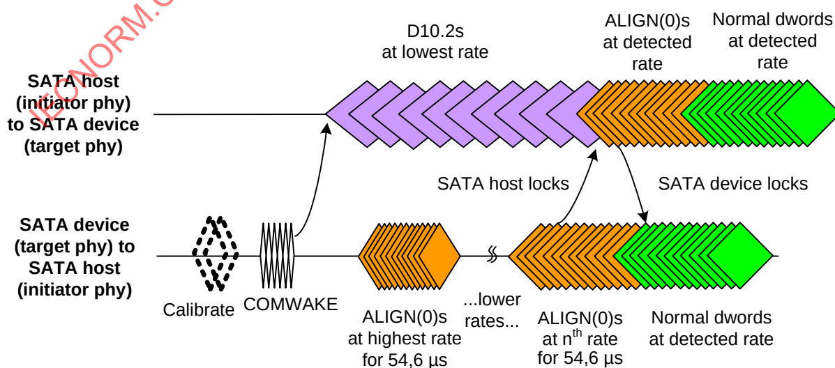
Figure 115 — SATA speed negotiation sequence
