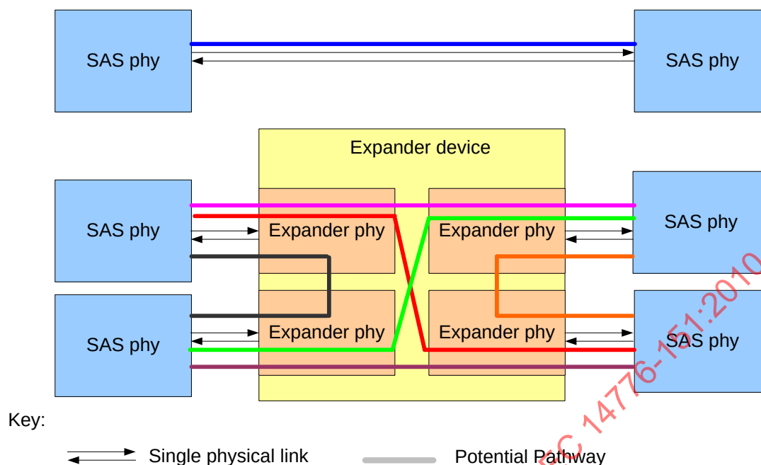
Figure 28 — Potential pathways
