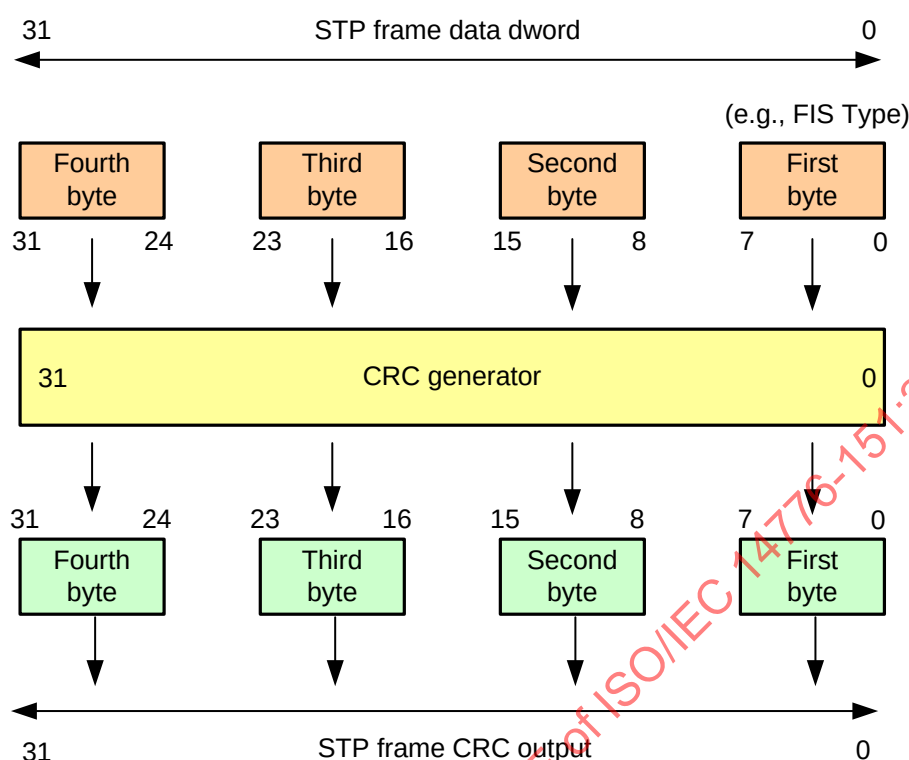
Figure 134 — STP frame CRC bit ordering
