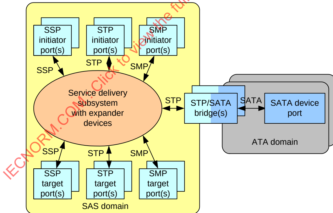
Figure 21 — SAS domain bridging to ATA domains
