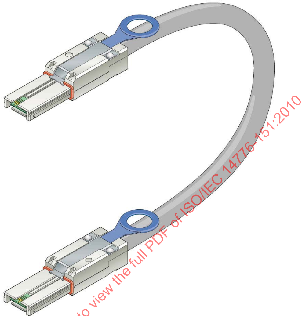
Figure 87 — SAS external cable assembly with Mini SAS 4x cable plug connectors
