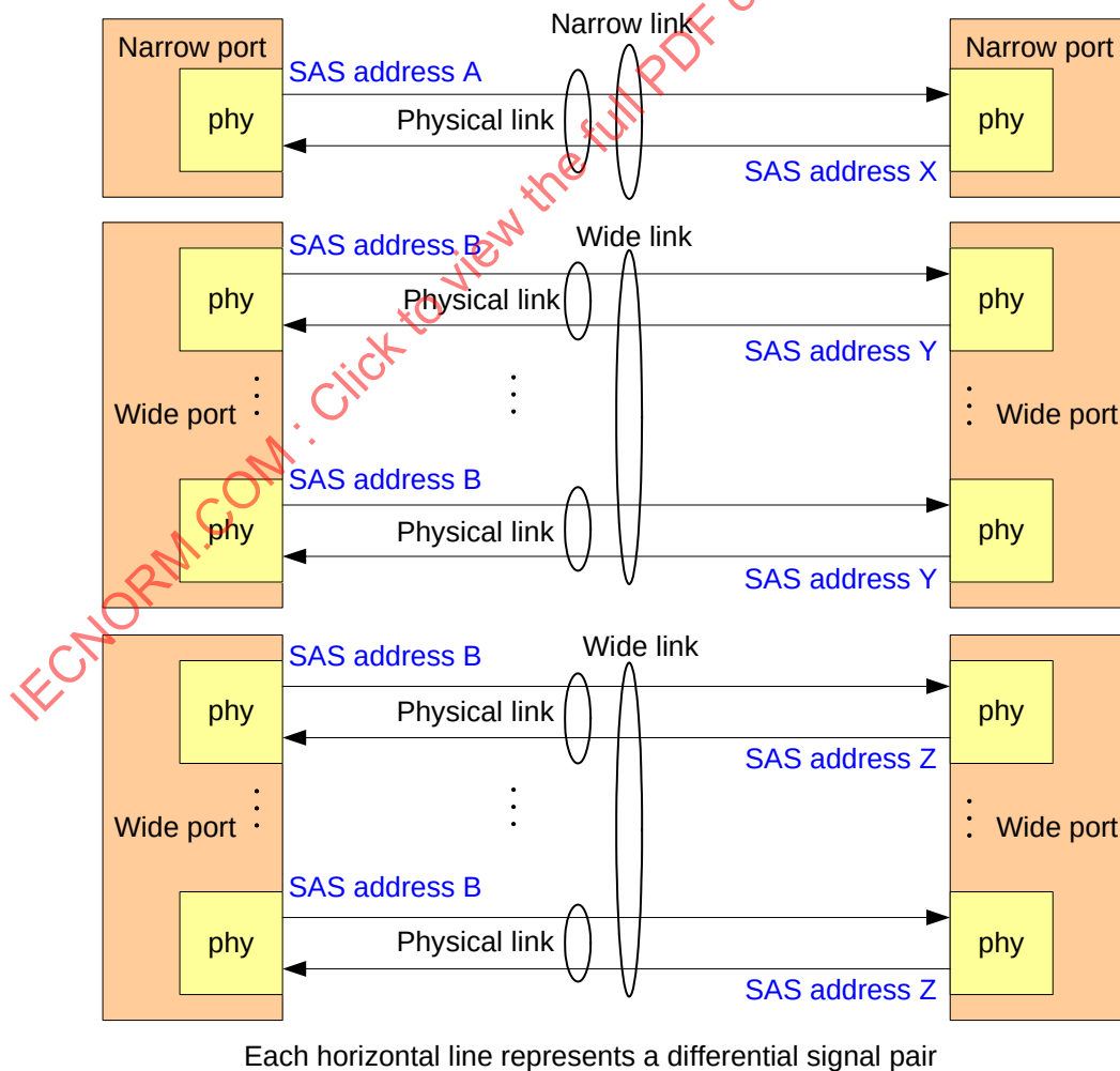
Figure 14 — Ports (narrow ports and wide ports)
