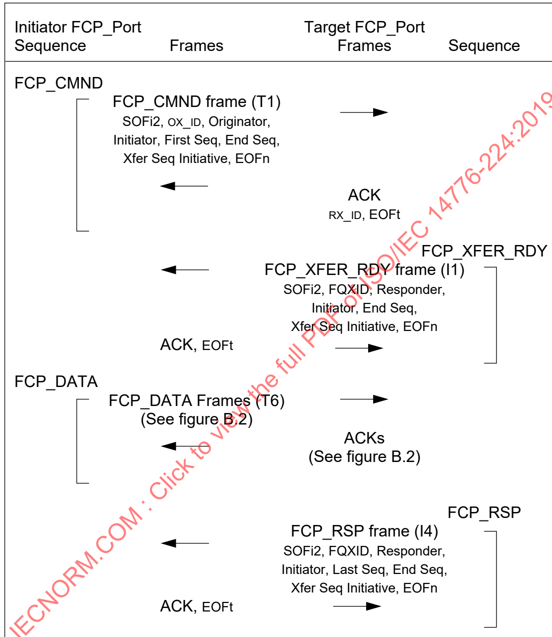
Figure B.1 - Class 2 write command example
