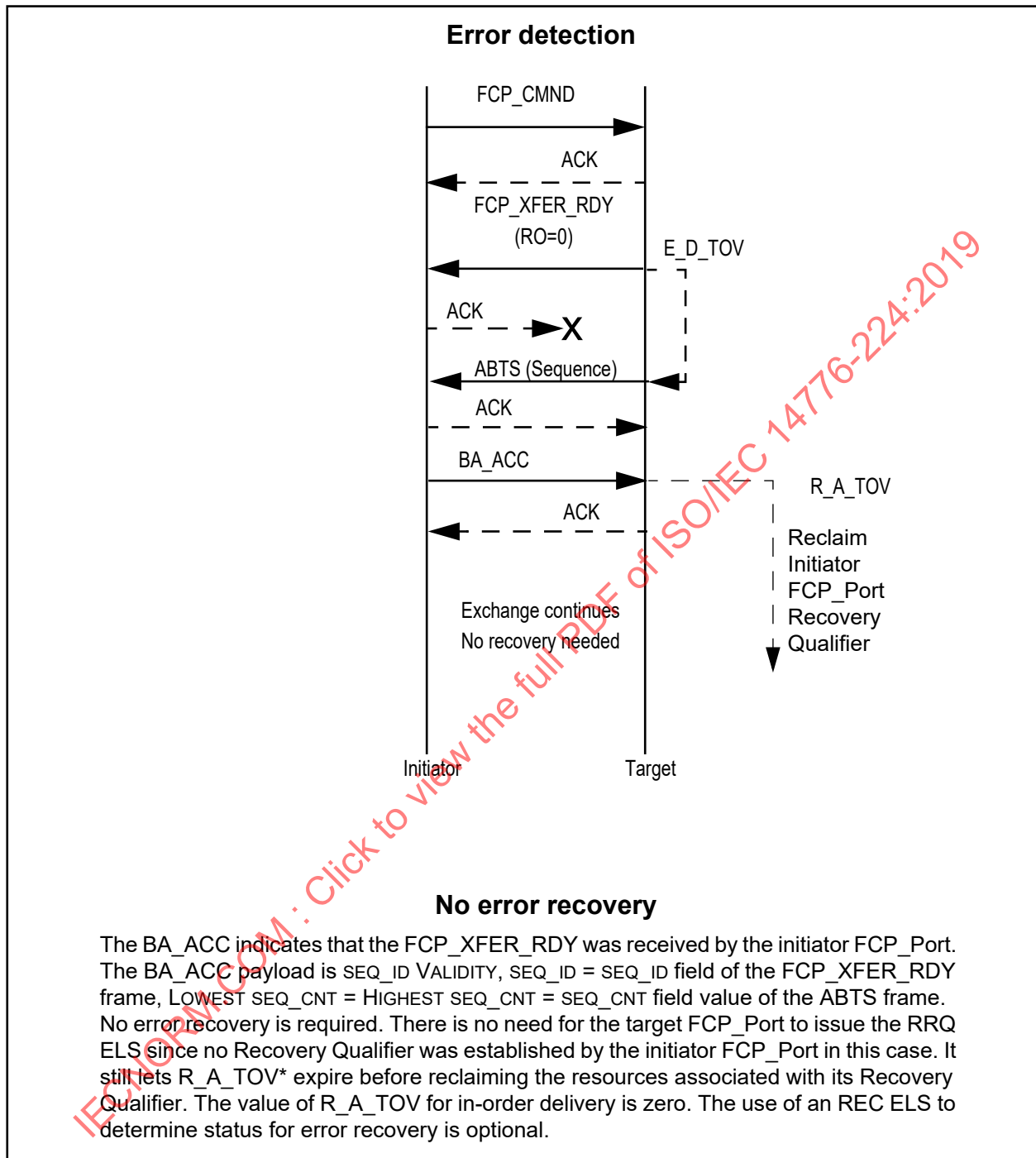
Figure C.7 - FCP_XFER_RDY received, ACK lost, acknowledged classes
