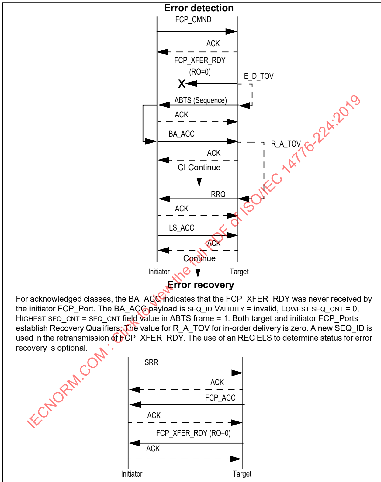
Figure C.6 - FCP_XFER_RDY lost, acknowledged classes
