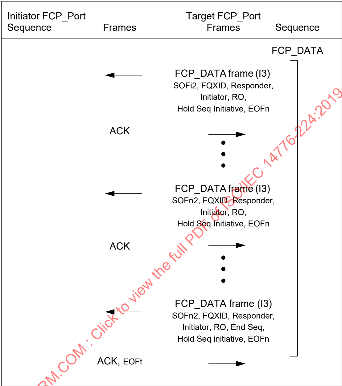
Figure B.4 - Class 2 read data example
