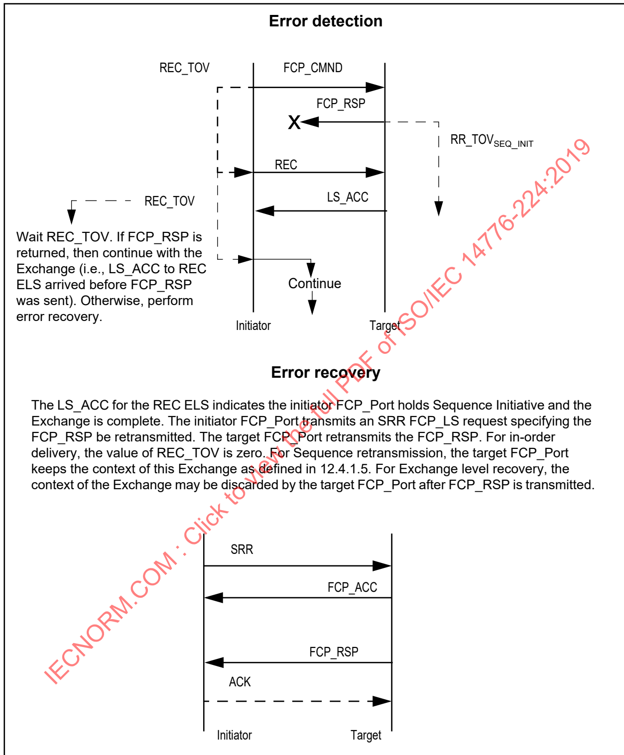
Figure C.8 - FCP_RSP lost, FCP_CONF not requested, unacknowledged classes
