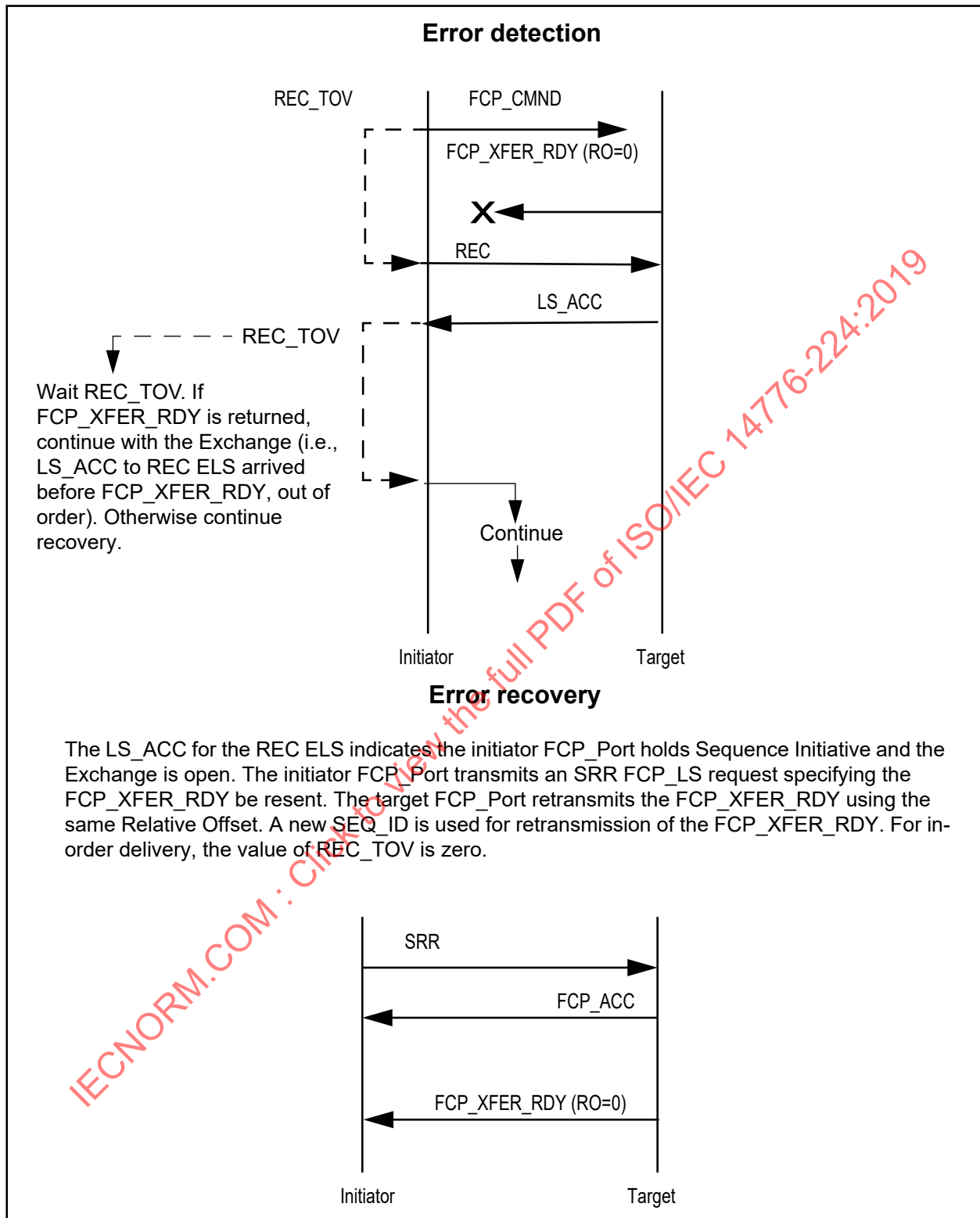
Figure C.5 - FCP_XFER_RDY lost, unacknowledged classes
