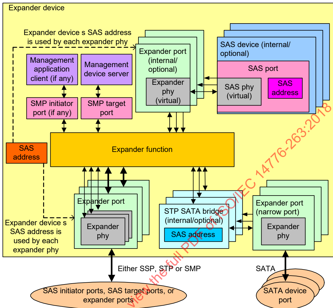
Figure 18 — Expander device
