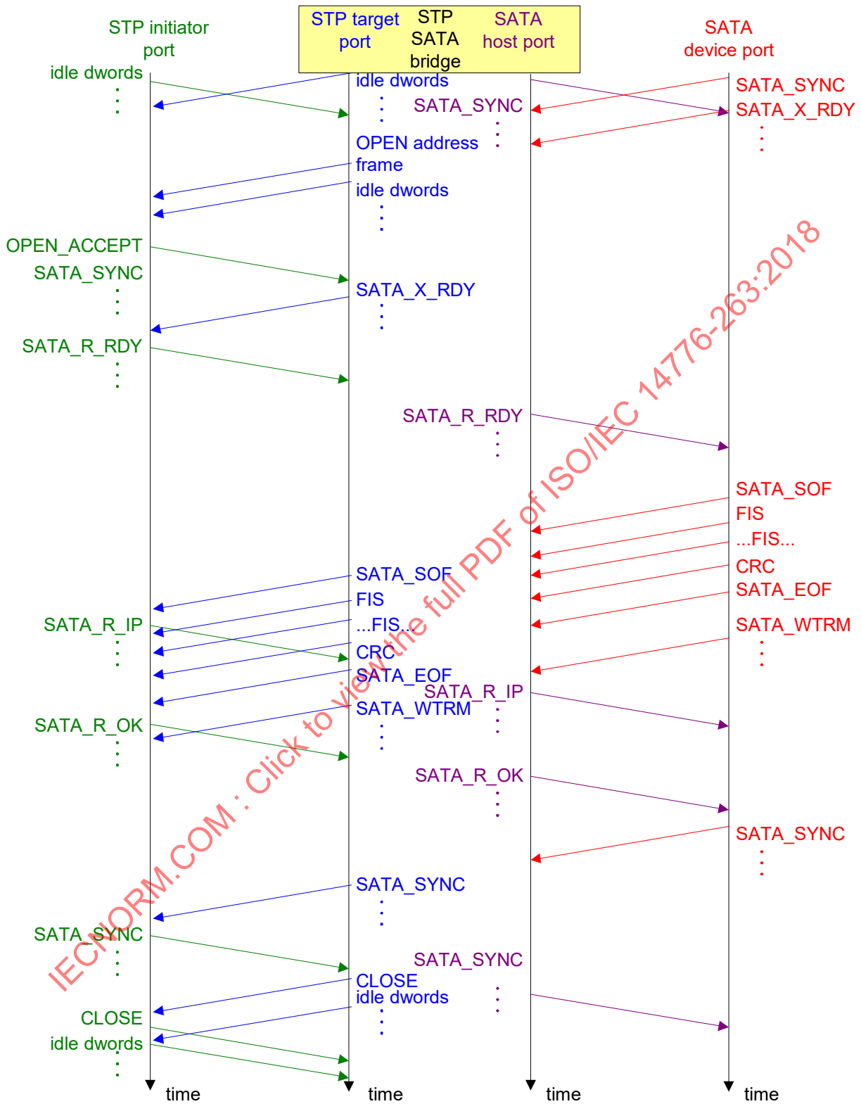
Figure 154 — STP target port opening an STP connection
