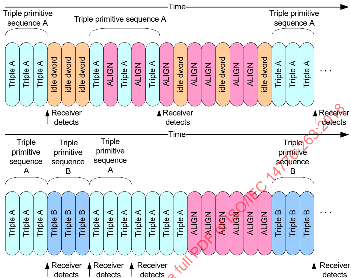
Figure 112 — Triple primitive sequences
