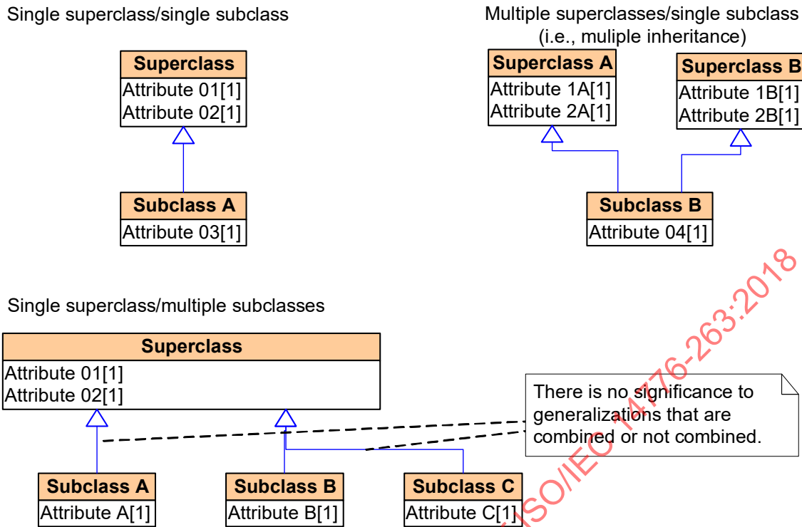
Figure 6 — Example of generalization relationships in class diagrams
