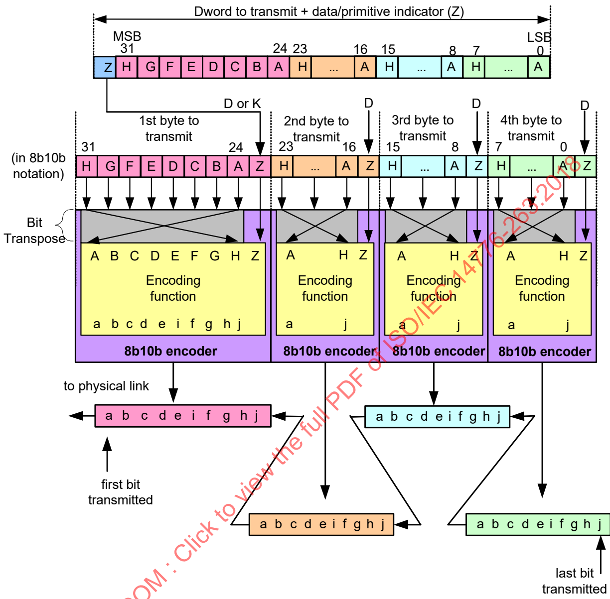
Figure 56 — SAS bit transmission logic
