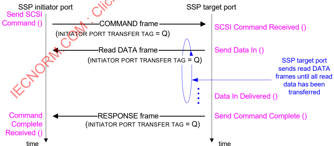
Figure 165 — Read command sequence of SSP frames
