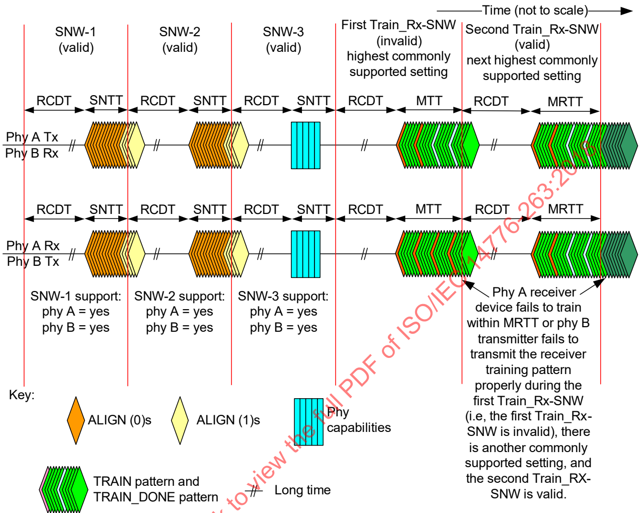
Figure 81 — SAS speed negotiation sequence - multiple Train_Rx-SNWs
