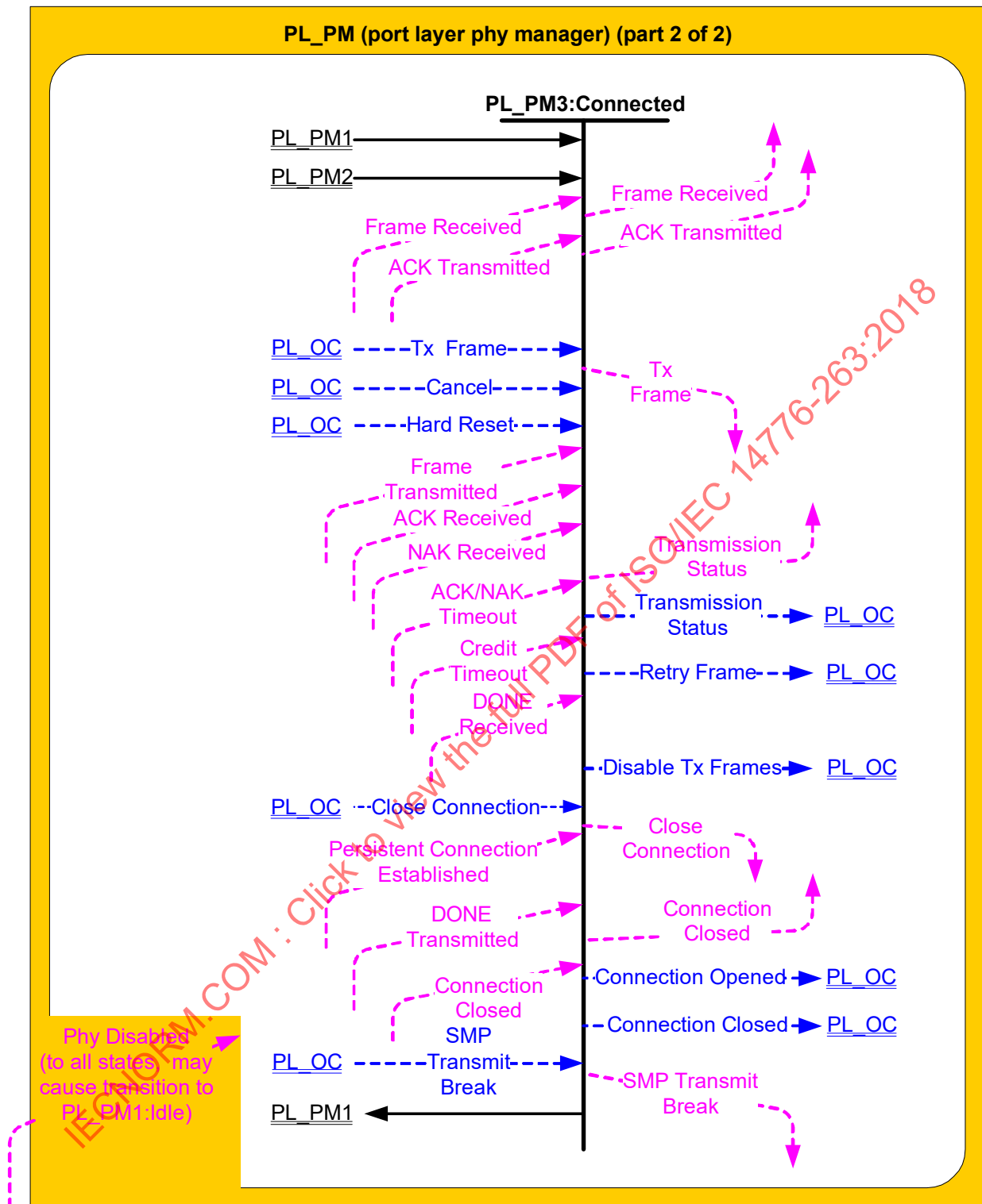
Figure 161 — PL_PM (port layer phy manager) state machine (part 2)
