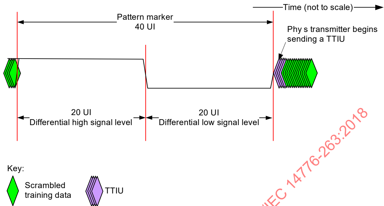
Figure 70 — Pattern marker transmission
