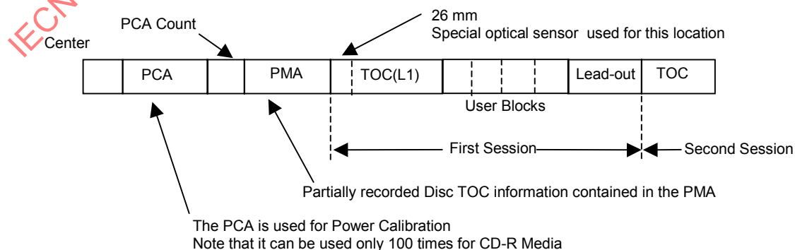
Figure 9 – CD-R and CD-RW medium
