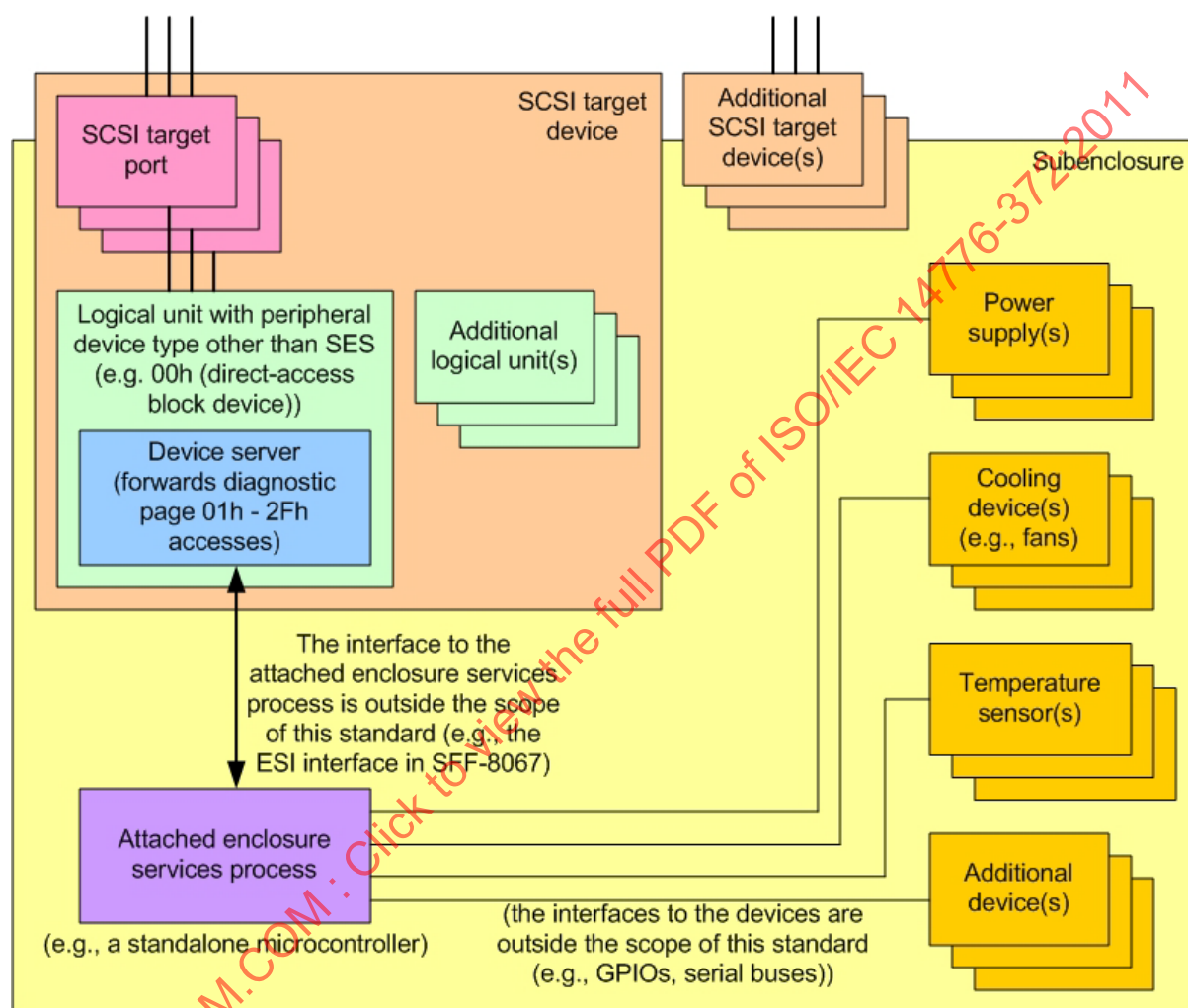
Figure 2 — Attached enclosure services process
