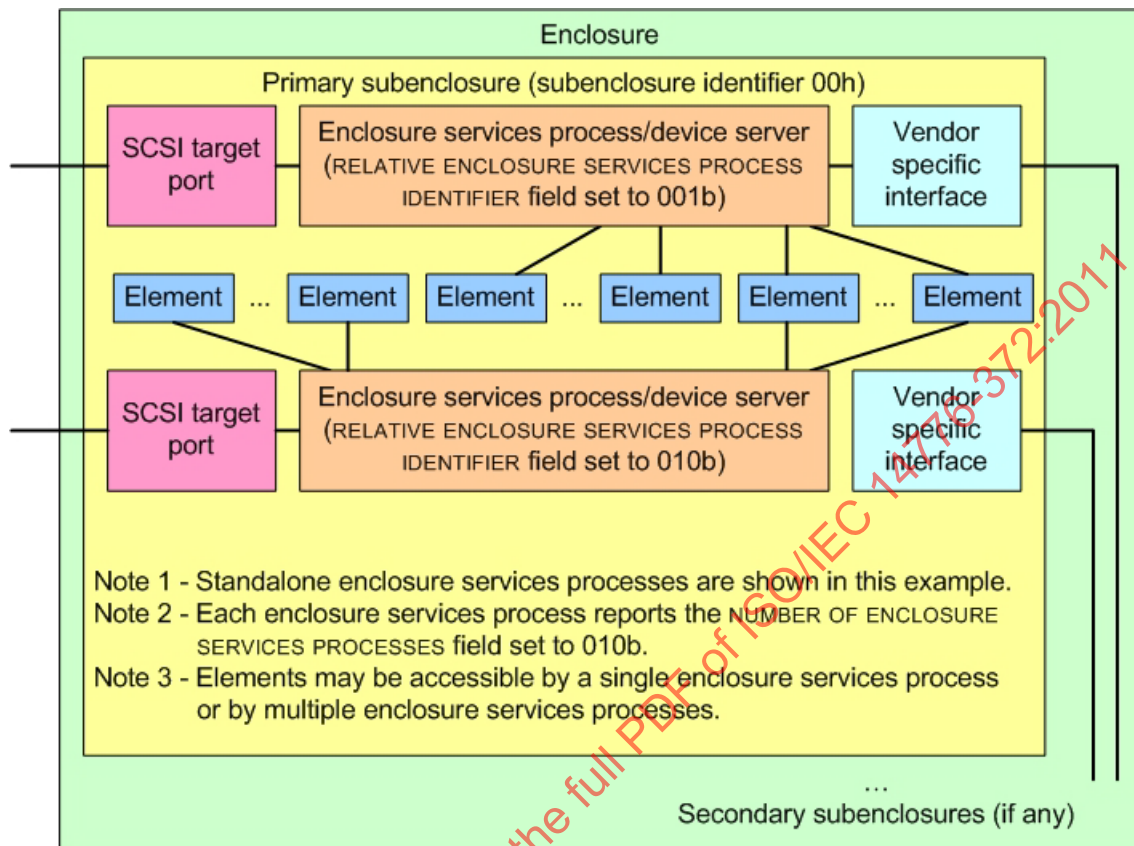
Figure 4 — Multiple enclosure service processes in a subenclosure
