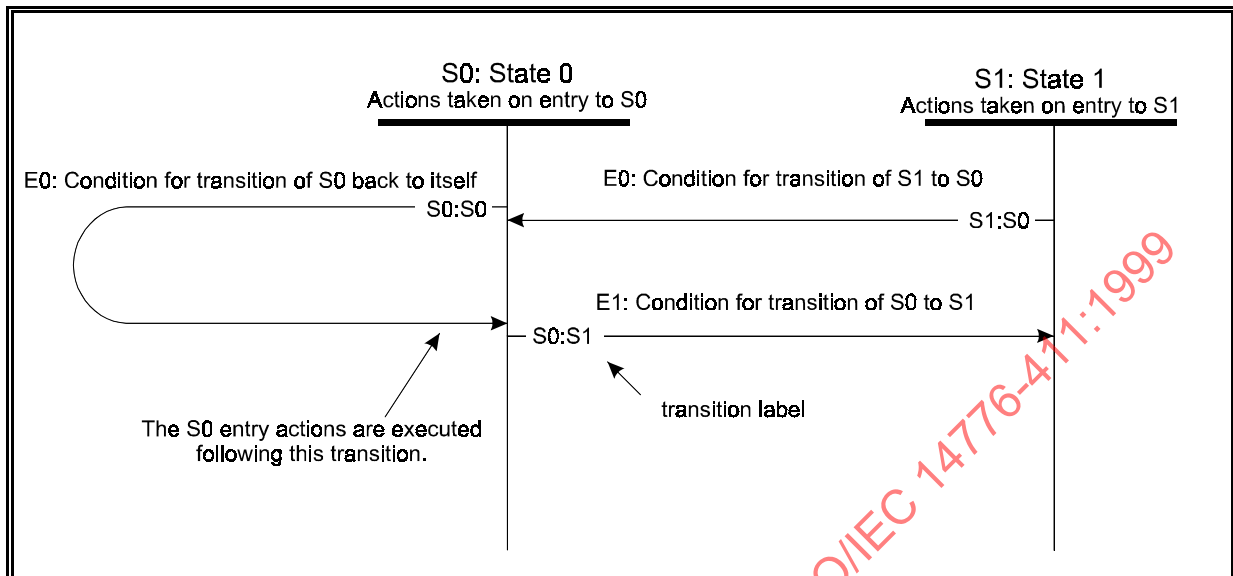
Figure 3 – State Diagram
