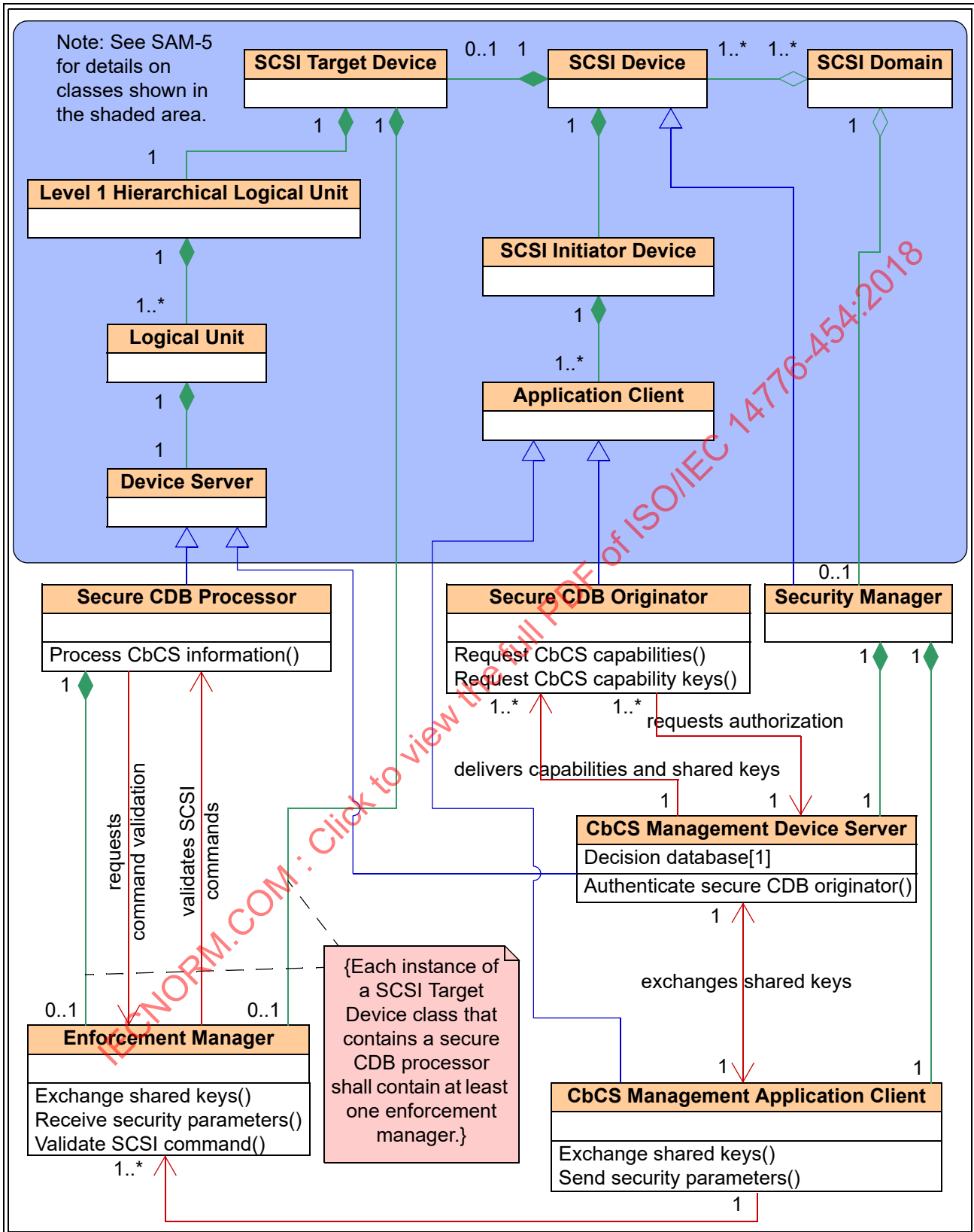
Figure 15 — CbCS overview class diagram
