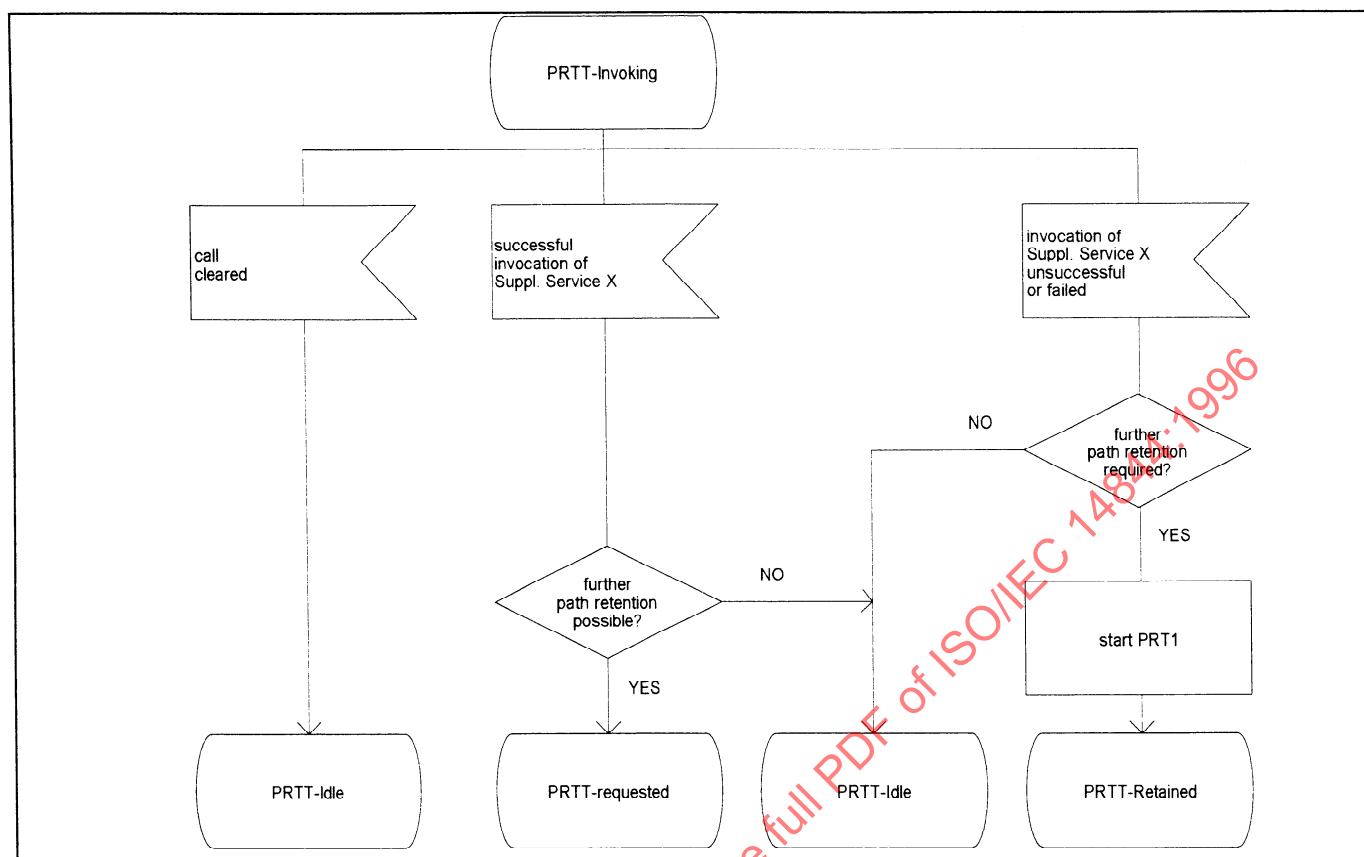
Figure A.2 (sheet 2 of 2) - SDL representation of Path Retention at the Terminating PINX
