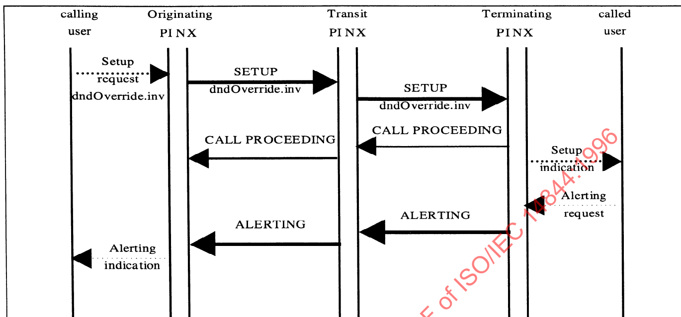
Figure C.3 - Message sequence for normal operation of SS-DNDO without using Path Retention, override successful
