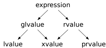
Figure 1: Expression category taxonomy [fig:basic.lval]
