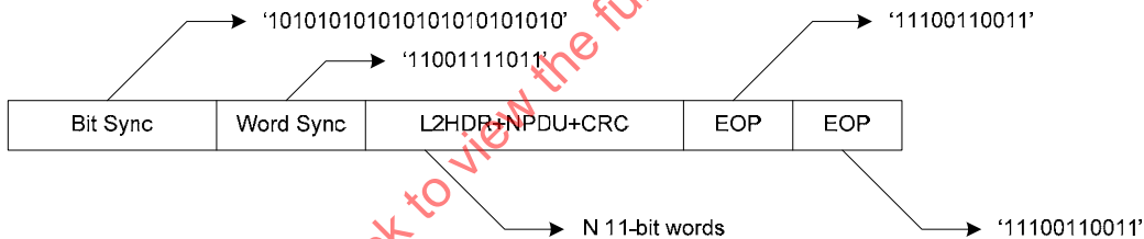
Figure 2 — Power line packet format
