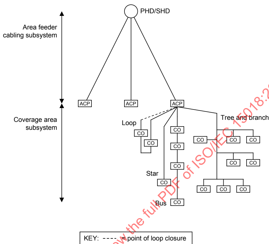
Figure 10 – Hierarchical structure of a generic cabling system in support of CCCB applications
