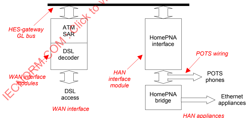
Figure A.5 – DSL/HomePNA Scenario
