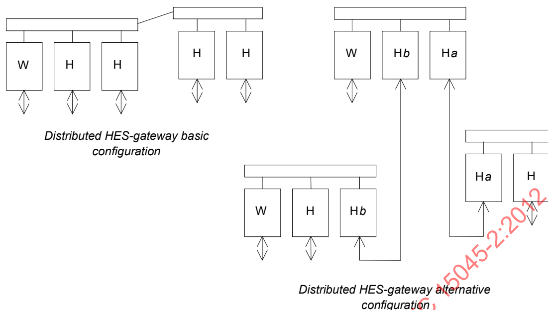
Figure 3 – Alternative distributed modular architectural models
