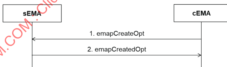
Figure 35 – Interaction diagram: Create opt
