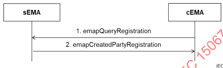
Figure 6 – Interaction diagram: Query registration
