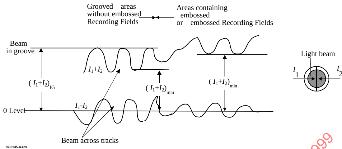
Figure 25a - Signals from grooves in the Tracking Channel
