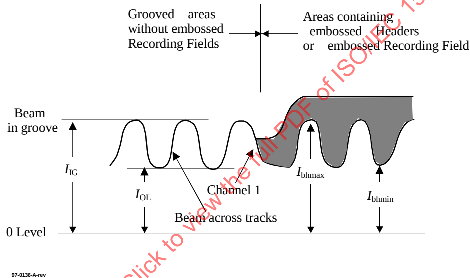
Figure 25b - Signals from grooves in Channel 1
