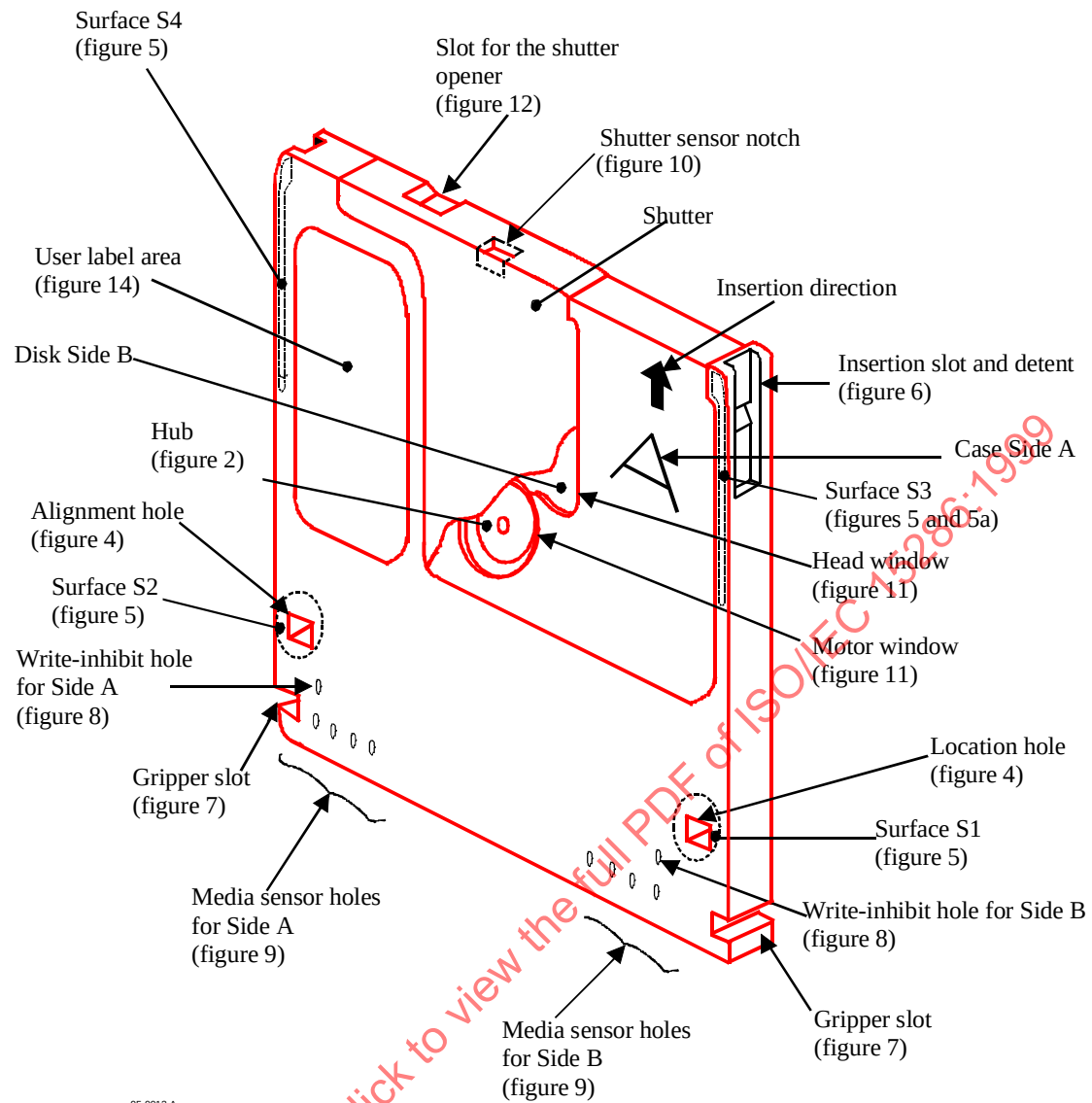
Figure 3 - Case
