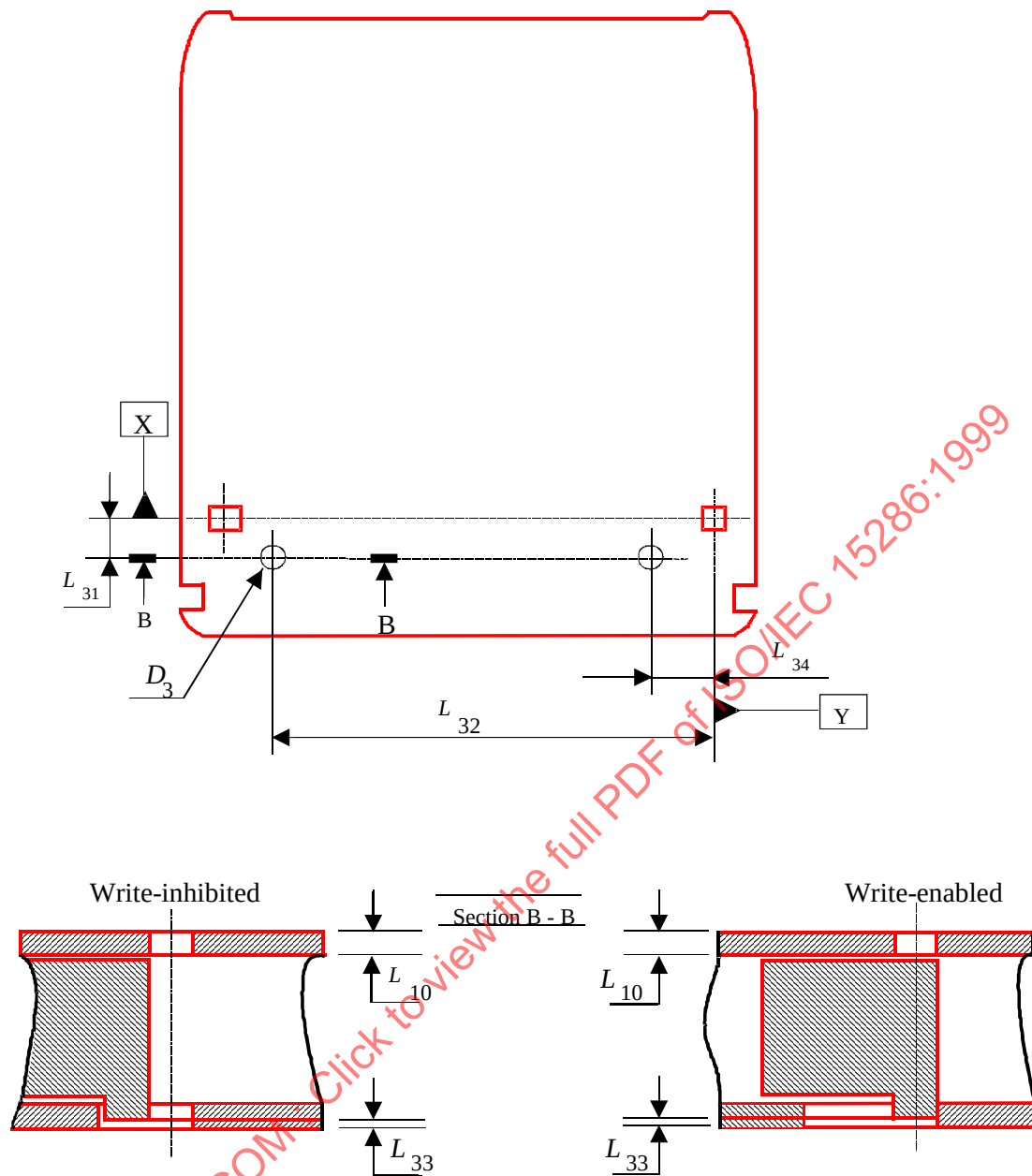
Figure 8 - Write-Inhibit holes
