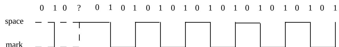
Figure 20 - Postamble pattern
