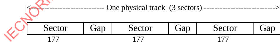
Figure 23 - Track format in the PEP Zone
