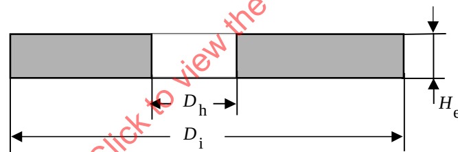
Figure D.1 - Test device for the clamping characteristic of the hub
