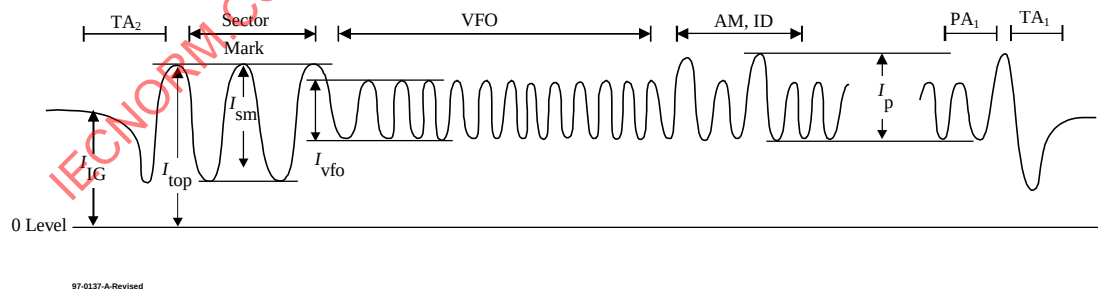
Figure 25c - Signals from Headers in Channel 1
