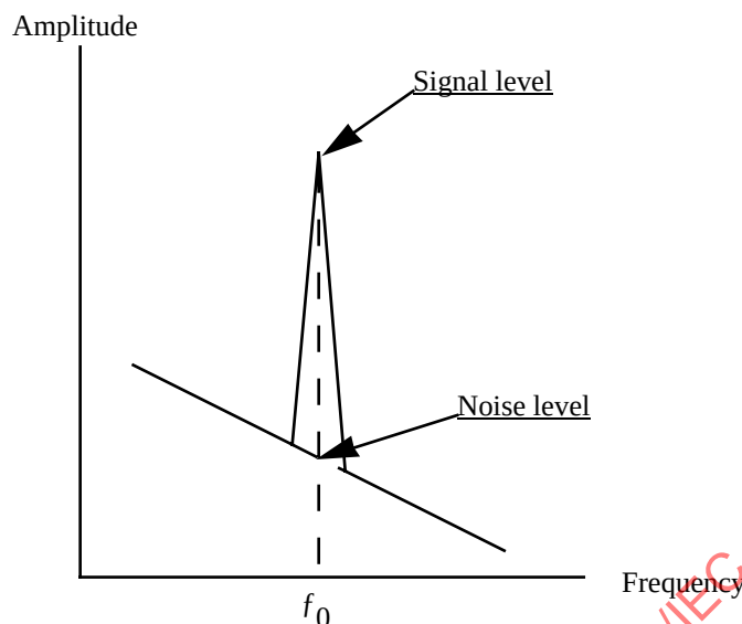
Figure 28 - Amplitude versus frequency for the magneto-optical signal
