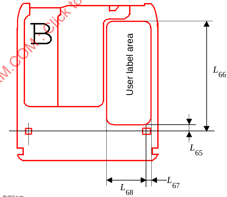
Figure 14c - User label area on Side B
