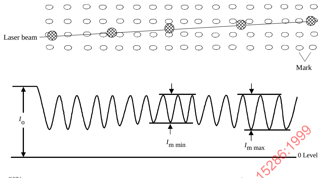
Figure 26 - Path of the laser beam when crossing tracks and the resulting PEP signals
