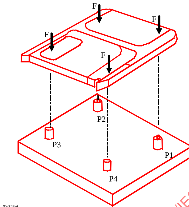
Figure C.1 - Compliance gauge
