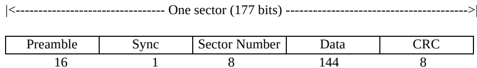
Figure 24 - Sector format in the PEP Zone
