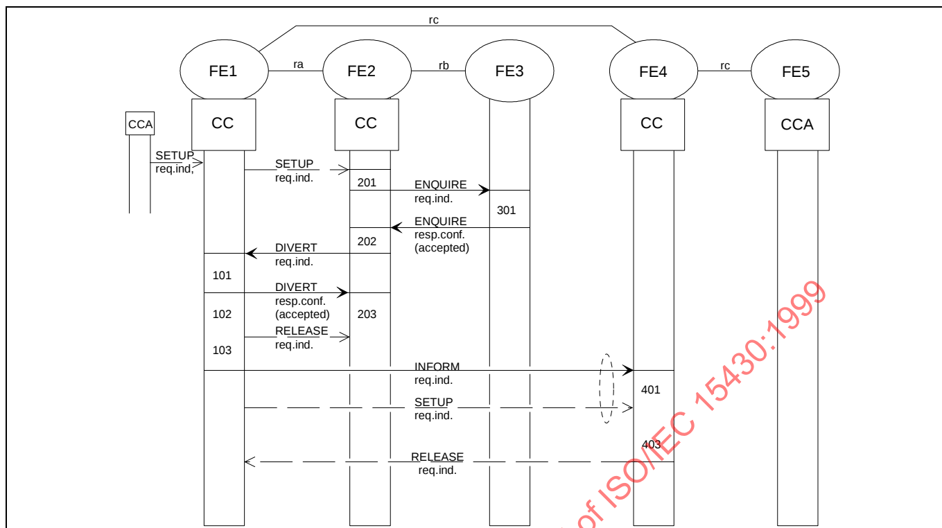
Figure 8 - Information flow sequence for unsuccessful WTMI operation: WTMI user not known at visitor PINX
