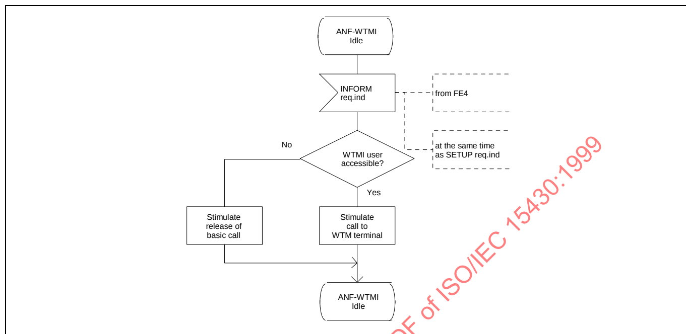
Figure 15 - ANF-WTMI, SDL for functional entity FE5
