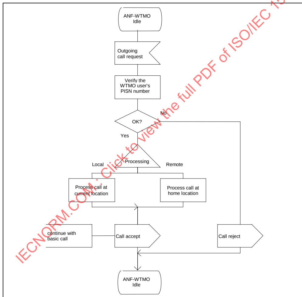
Figure 2 - ANF-WTMO, overall SDL
