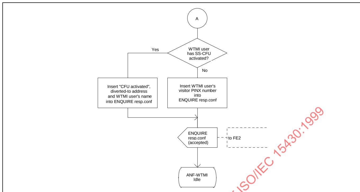
Figure 13 - ANF-WTMI, SDL for functional entity FE3 (page 2 of 2)
