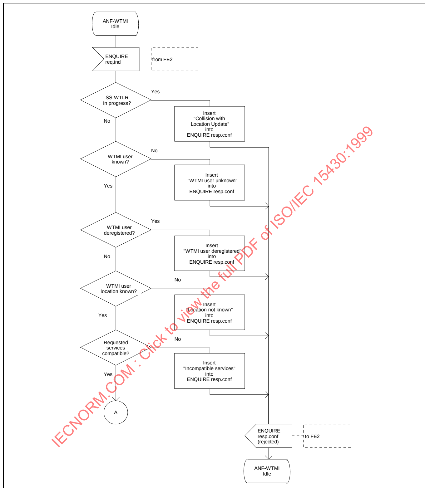
Figure 12 - ANF-WTMI, SDL for functional entity FE3 (page 1 of 2)
