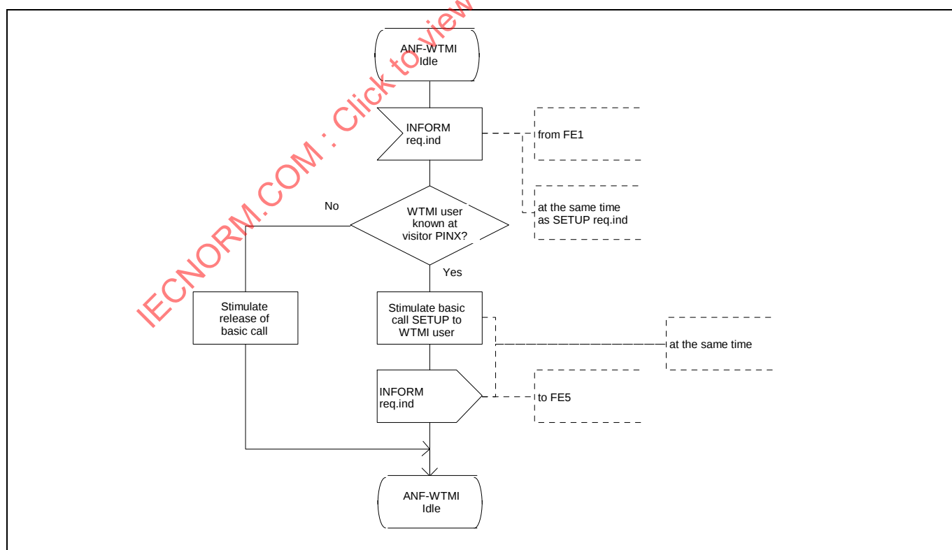
Figure 14 - ANF-WTMI, SDL for functional entity FE4
