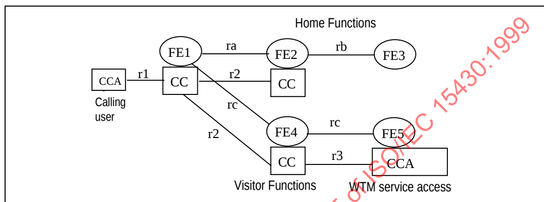
Figure 4 - Example relationship between model for ANF-WTMI and basic call
