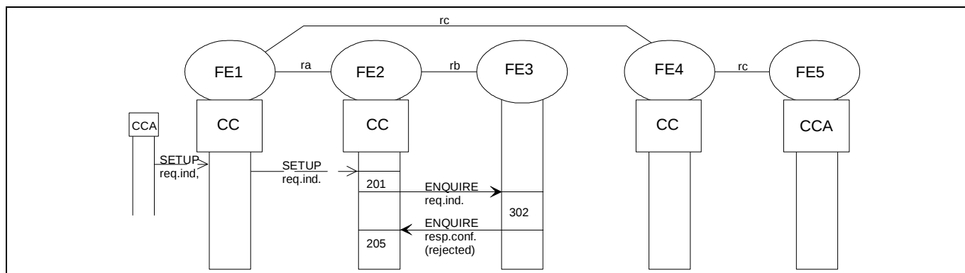
Figure 6 - Information flow sequence for unsuccessful WTMI operation: WTMI user (location) not known at home PINX or WTMI user deregistered
