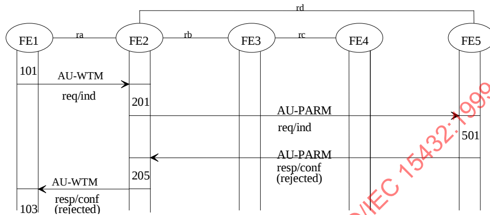
Figure 7: Unsuccessful case, rejection from FE5
