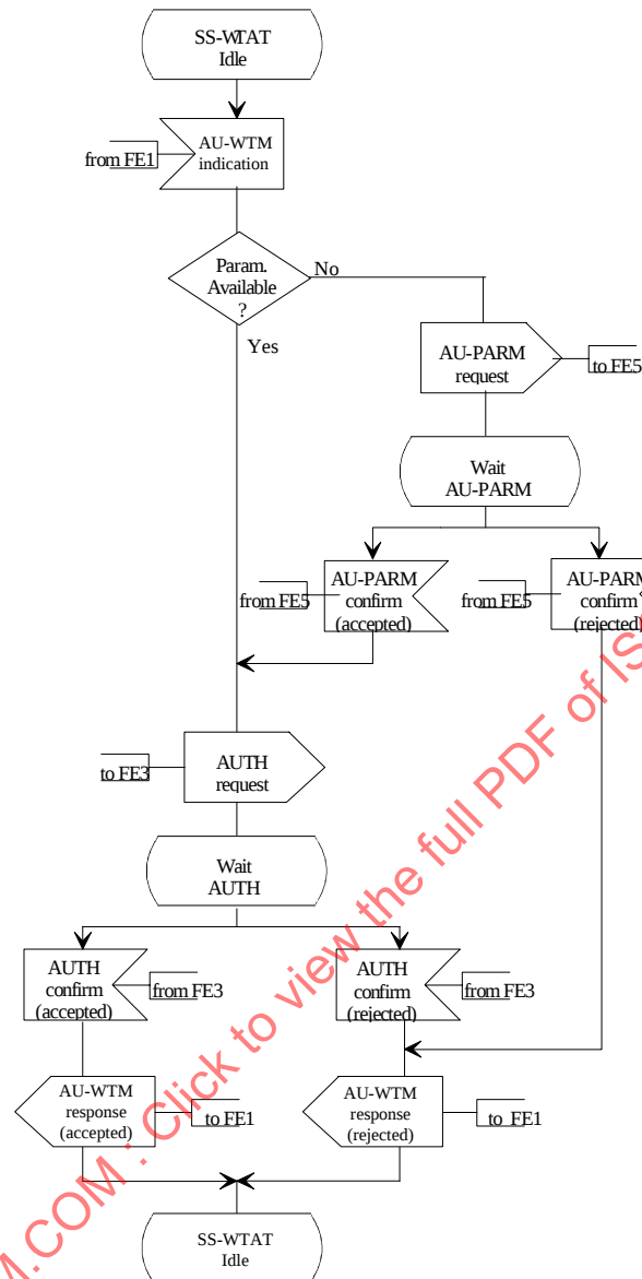
Figure 10: SS-WTAT, SDL for functional entity FE2
