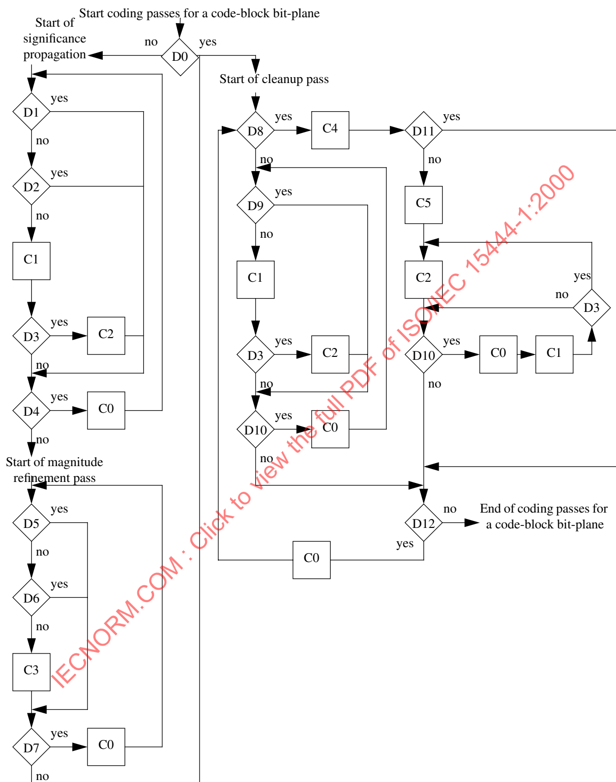
Figure D-3 — Flow chart for all coding passes on a code-block bit-plane
