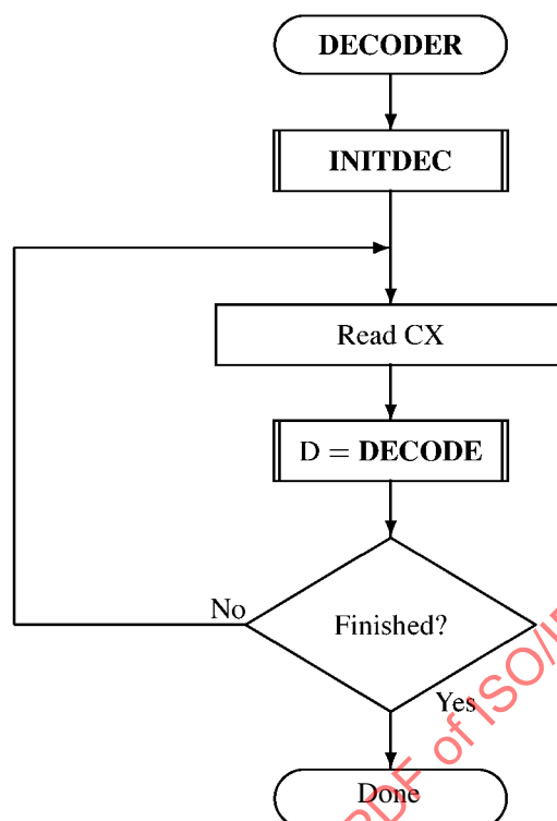
Figure C-14 — Decoder for the MQ-coder
