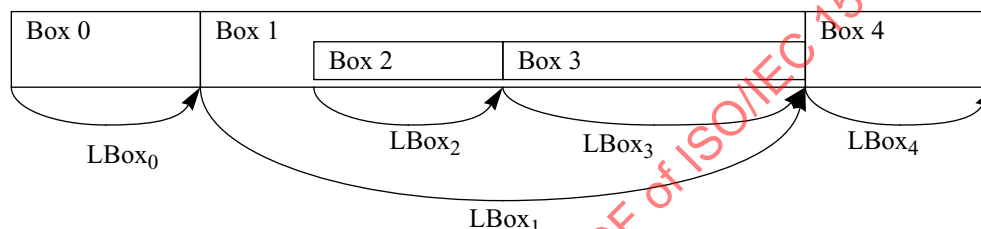
Figure I-5 — Illustration of box lengths
