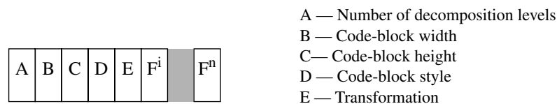
Figure A-11 — Coding style parameter diagram of the SPcoc parameters
