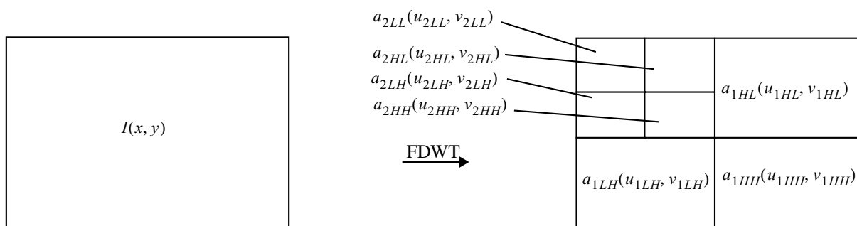
Figure F-18 — The FDWT ( N_L=2 )
