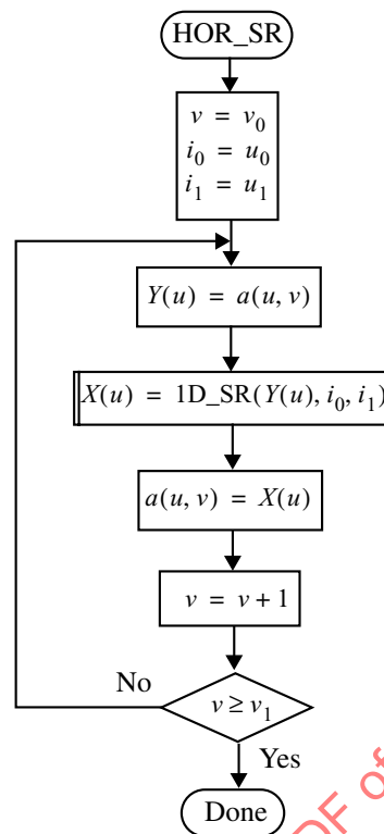
Figure F-10 — The HOR_SR procedure
