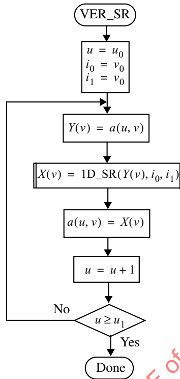
Figure F-12 — The VER_SR procedure
