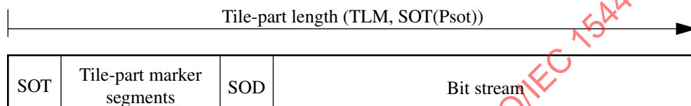
Figure A-16 — Tile-part lengths
