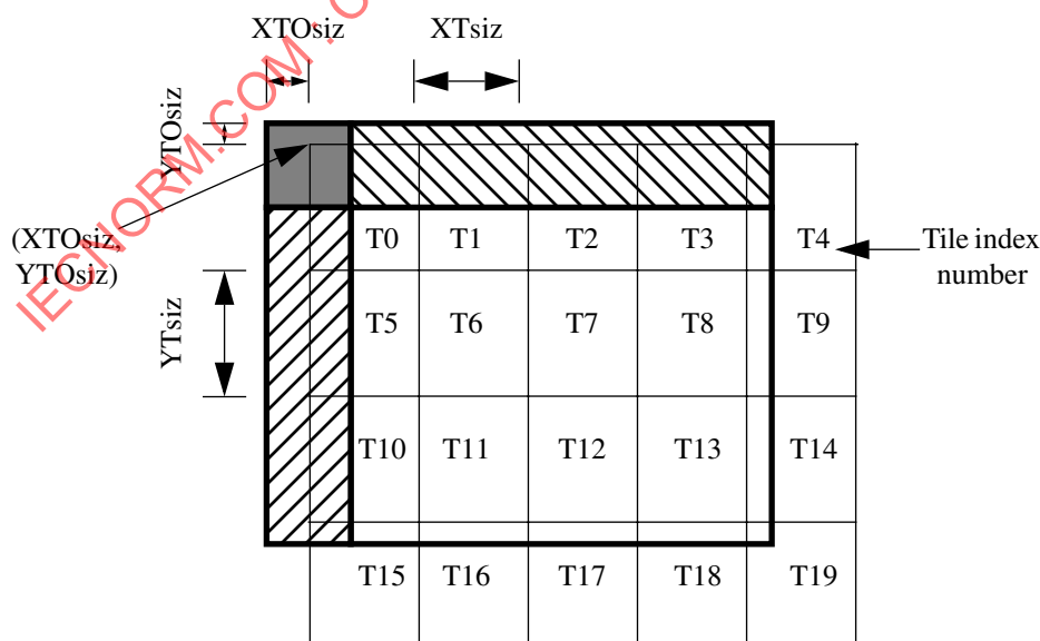
Figure B-4 — Tiling of the reference grid diagram
