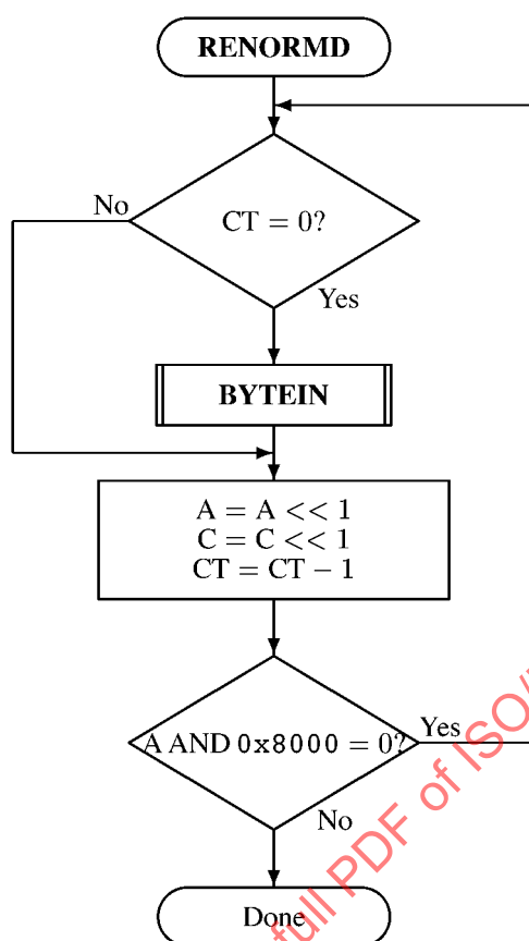
Figure C-18 — Decoder renormalisation procedure
