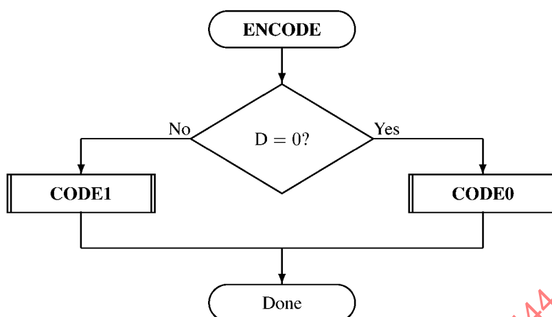
Figure C-3 — ENCODE procedure
