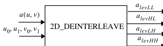
Figure F-27 — Parameters of 2D_DEINTERLEAVE procedure
