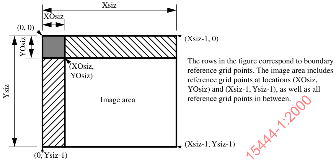
Figure B-1 — Reference grid diagram
