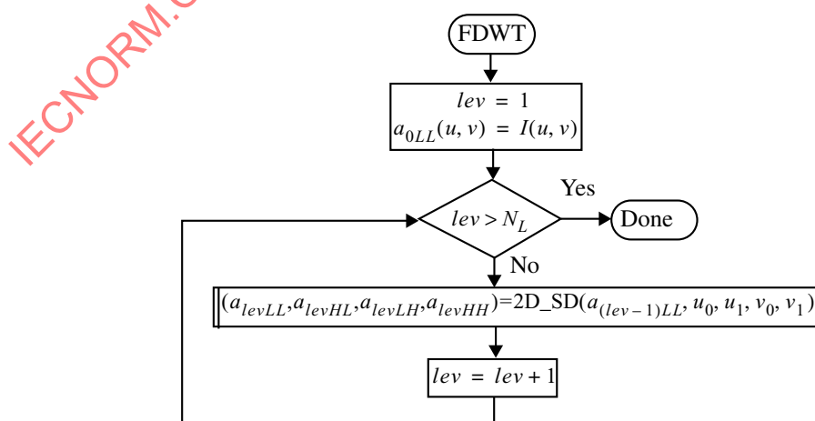
Figure F-19 — The FDWT procedure
