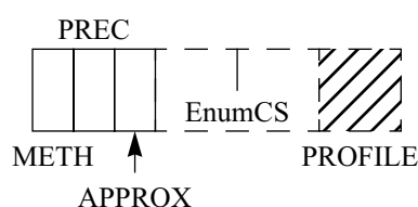
Figure I-10 — Organization of the contents of a Colour Specification box
