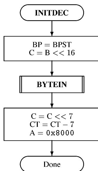
Figure C-20 — Initialisation of the decoder
