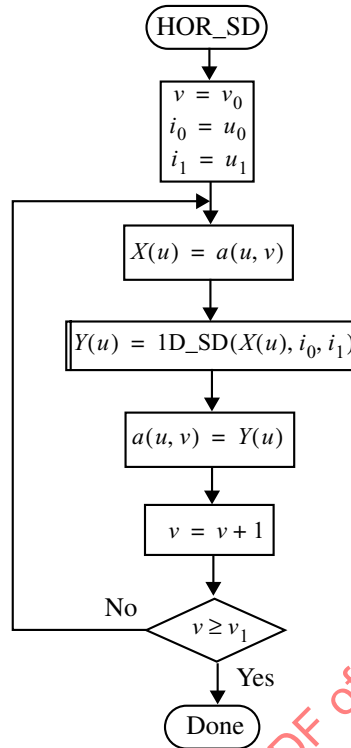
Figure F-26 — The HOR_SD procedure
