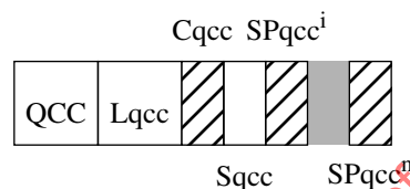
Figure A-14 — Quantization component syntax
