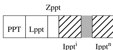
Figure A-21 — Packed packet headers, tile-part header syntax
