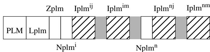
Figure A-18 — Packets length, main header syntax
