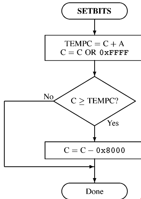
Figure C-12 — Setting the final bits in the C register
