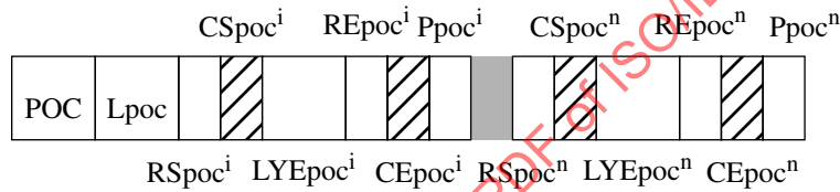
Figure A-15 — Progression order change tile syntax
