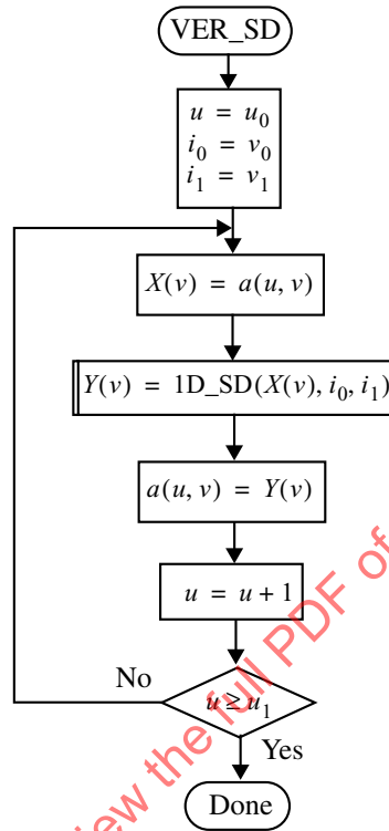
Figure F-24 — The VER_SD procedure
