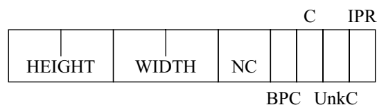
Figure I-8 — Organization of the contents of an Image Header box
