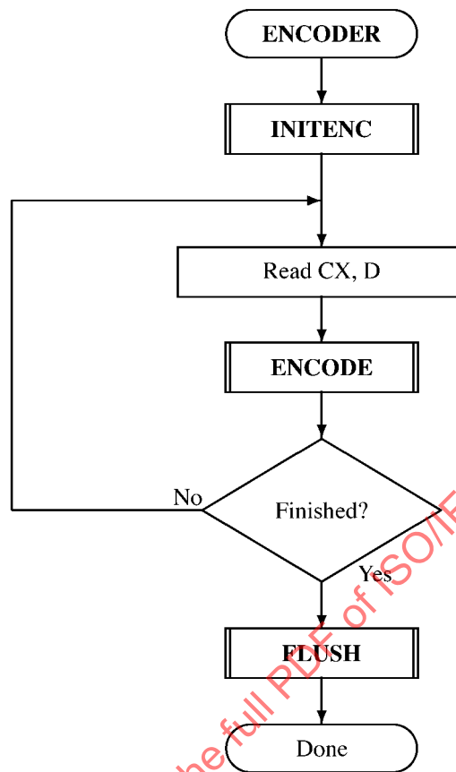
Figure C-2 — Encoder for the MQ-coder
