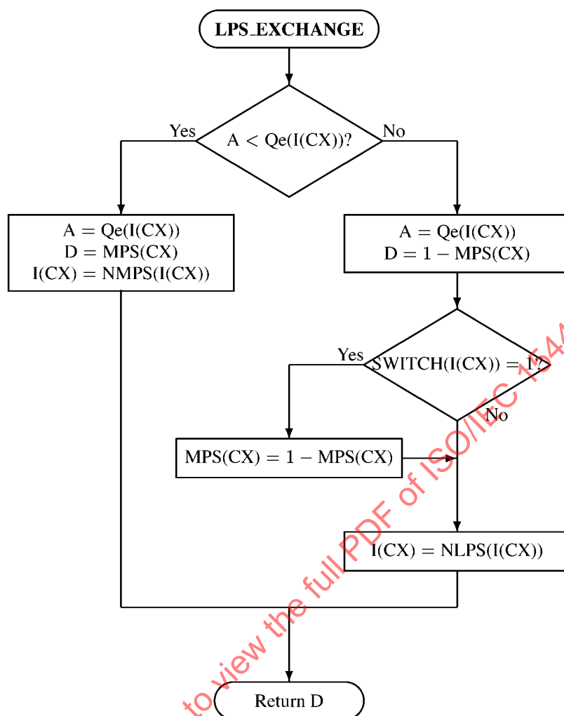
Figure C-17 — Decoder LPS path conditional exchange procedure
