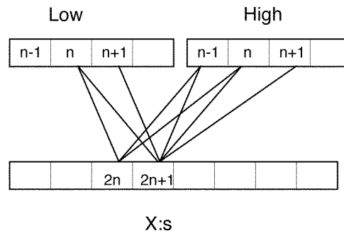
Figure H-1 — The inverse wavelet transformation with the 5-3 reversible filter
