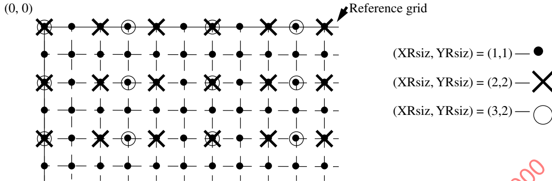
Figure B-2 — Component sample locations on the reference grid for different XRsize and YRsize values
