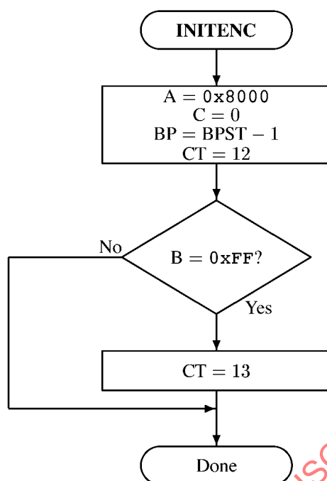
Figure C-10 — Initialisation of the encoder
