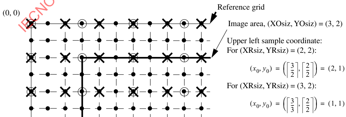
Figure B-3 — Example of upper left component sample locations
