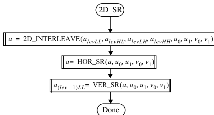
Figure F-6 — The 2D_SR procedure
