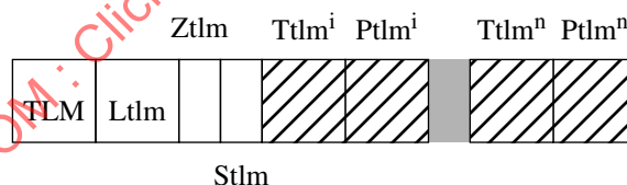
Figure A-17 — Tile-part length syntax
