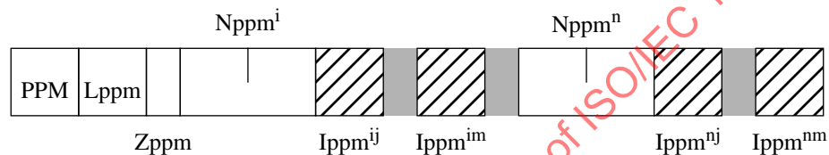
Figure A-20 — Packed packet headers, main header syntax
