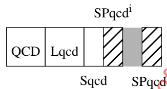
Figure A-13 — Quantization default syntax
