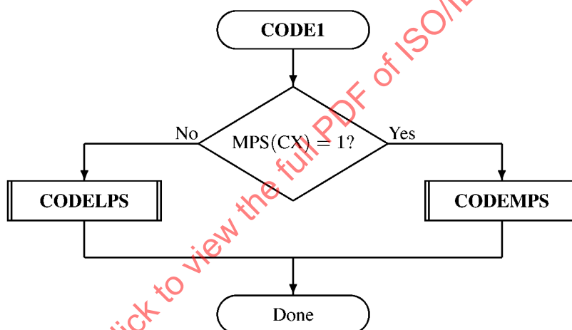
Figure C-4 — CODE1 procedure
