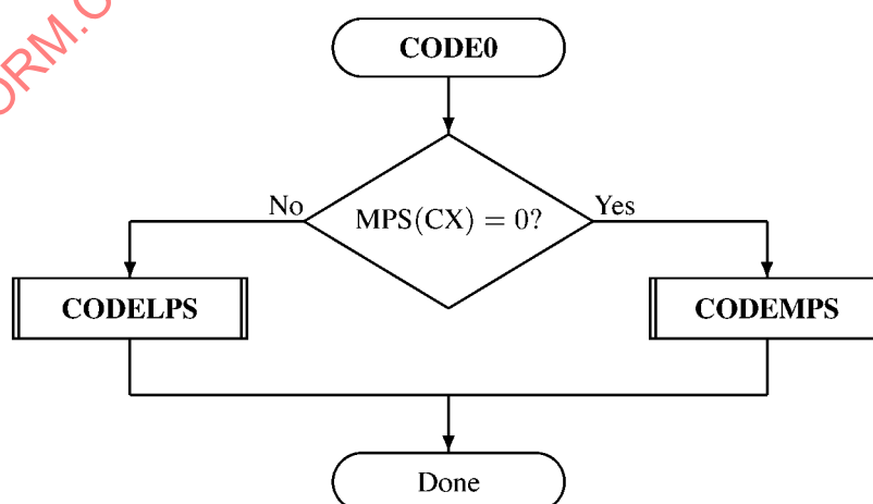
Figure C-5 — CODE0 procedure
