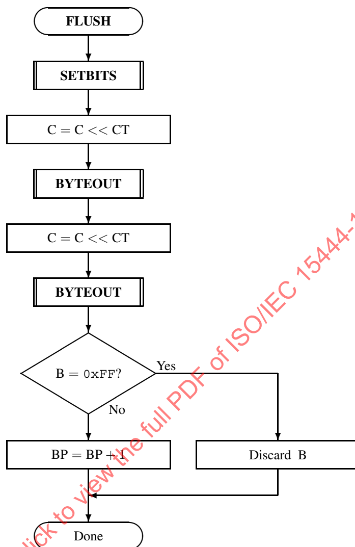
Figure C-11 — FLUSH procedure
