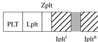
Figure A-19 — Packet length, tile-part header syntax
