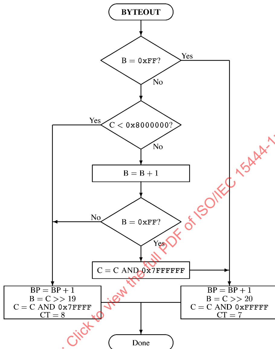
Figure C-9 — BYTEOUT procedure for encoder
