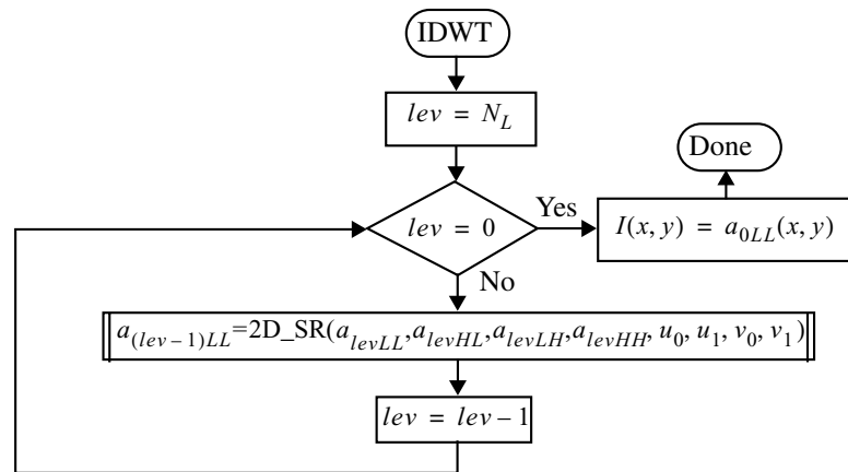
Figure F-3 — The IDWT Procedure
