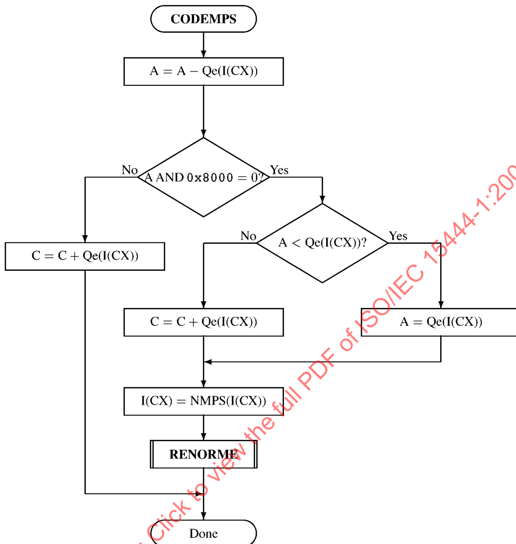
Figure C-7 — CODEMPS procedure with conditional MPS/LPS exchange
