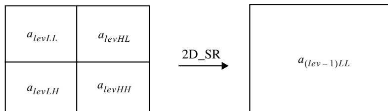
Figure F-5 — One level of reconstruction from four subbands (2D_SR procedure) into subbands
