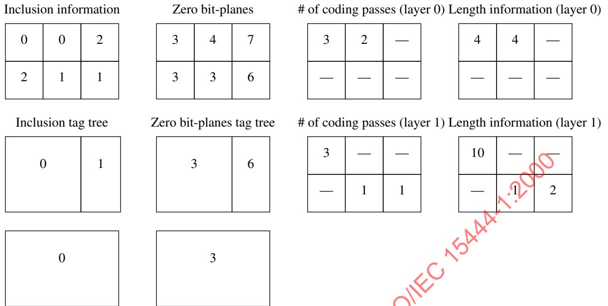
Figure B-13 — Example of the information known to the encoder
