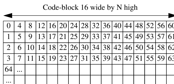
Figure D-1 — Example scan pattern of a code-block bit-plane
