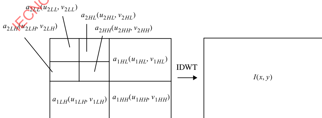
Figure F-2 — The IDWT ( N_L=2 )
